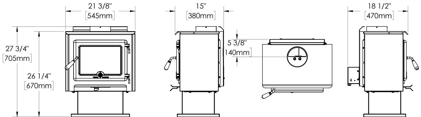
Figure 2: TN10 Dimensions, Pedestal Model.
