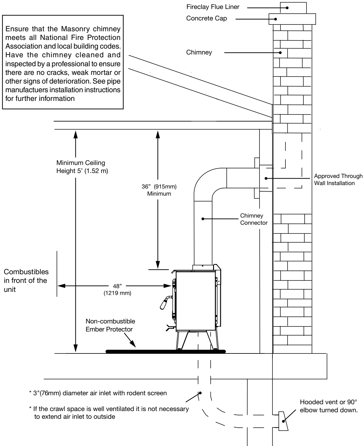
Figure 12: TN10 Venting to a masonry chimney.
