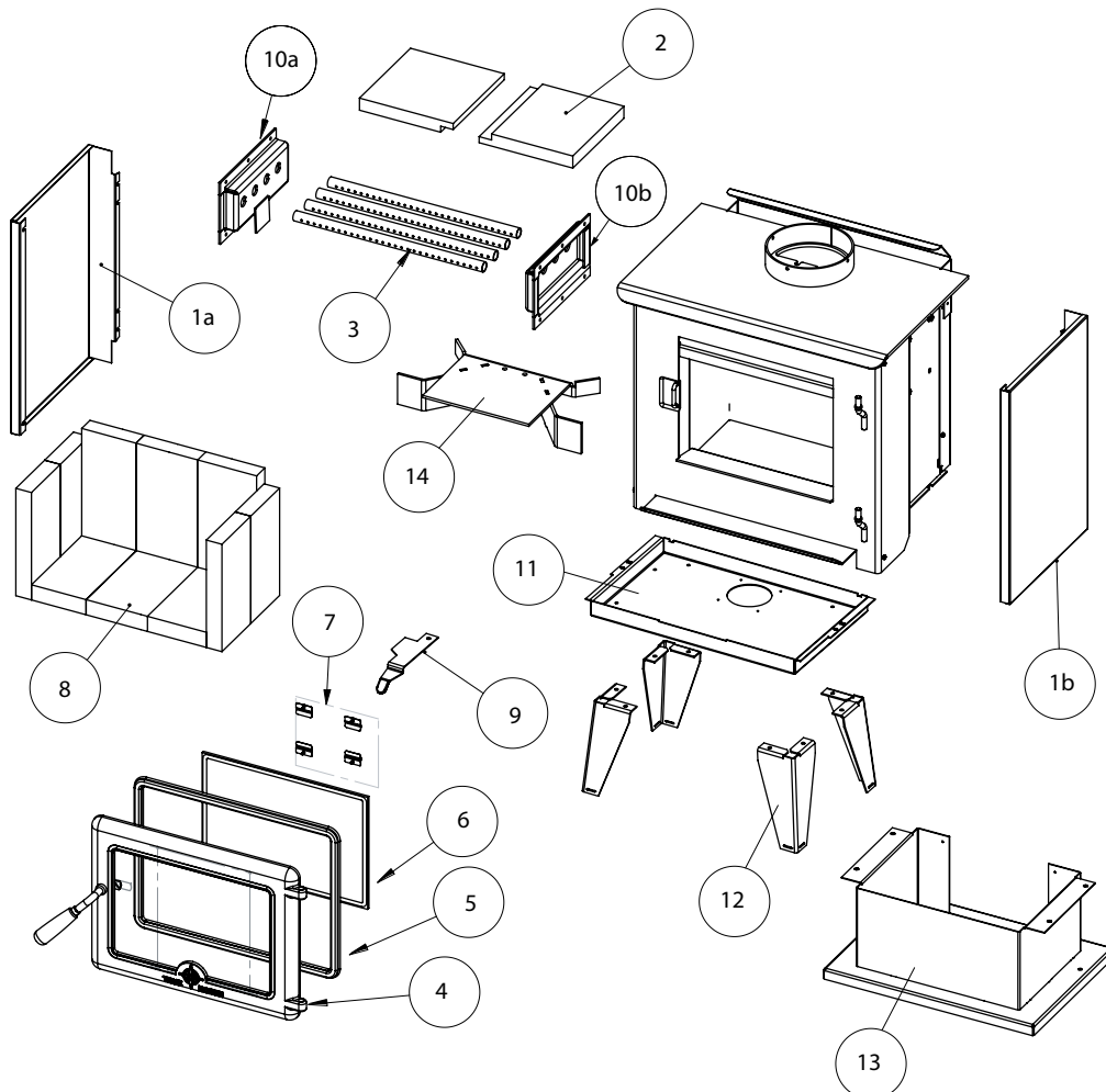
Figure 17: TN10 Exploded BOM .
