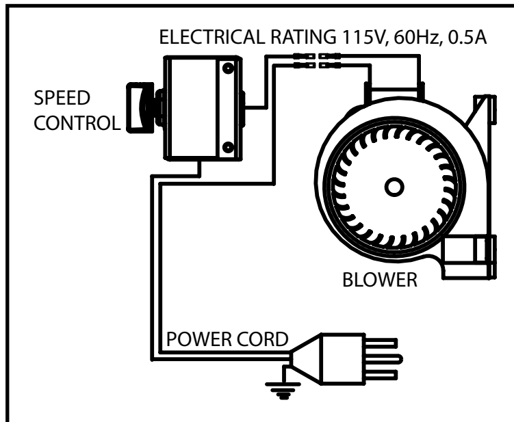
Figure 14: Blower Wiring Diagram.
