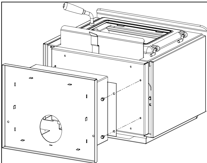
Figure 6: TN10 Pedestal Kit install.
