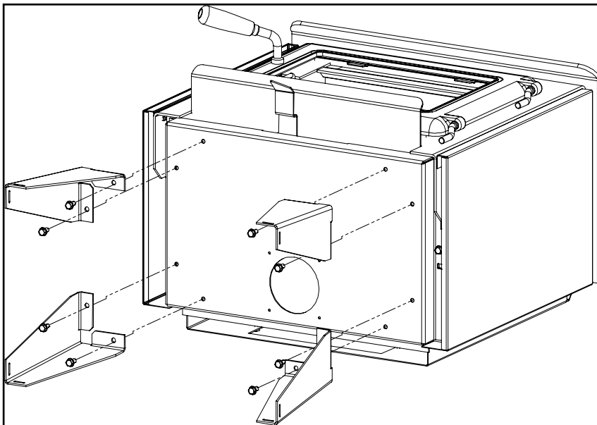
Figure 5: TN10 Leg Kit install.
