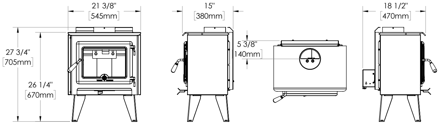
Figure 1: TN10 Dimensions, Leg Model.
