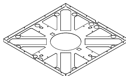
SUPPORT DE DESSUS (C) TOP SUPPORT PL77323
