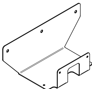
SUPPORT LATÉRAL (A) SIDE BRACKET 2X PL77322
