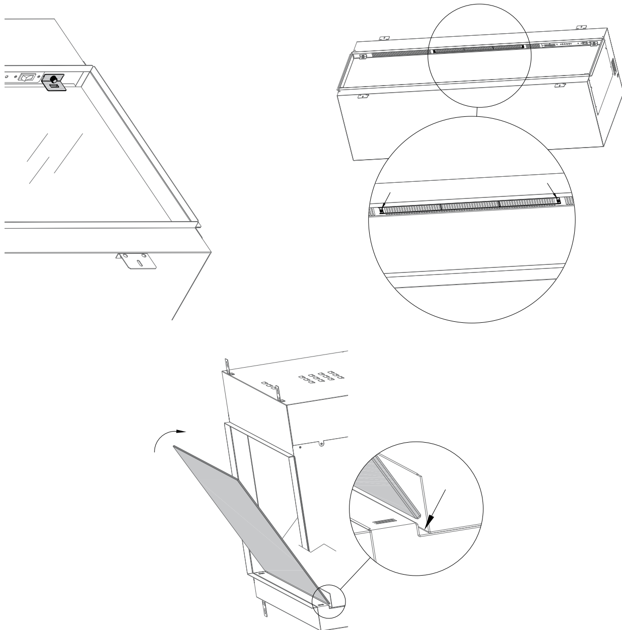
Figure 4.1 - Glass Removal
