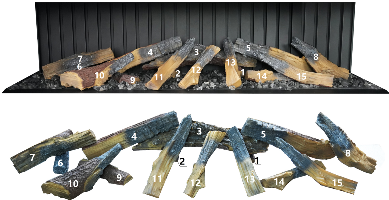
Figure 4.3 - Log Location and Identification
