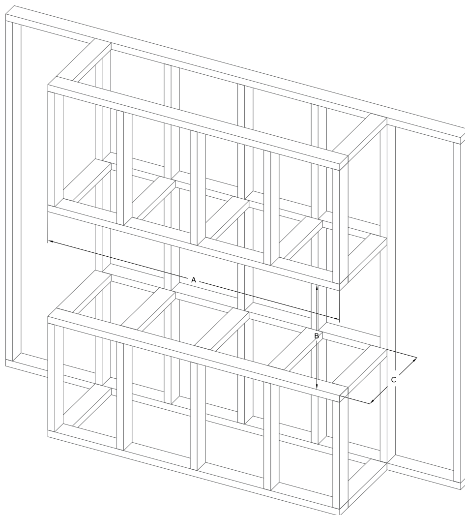
Figure 2.8 - Framed Opening - 3-Sided (Bay) Installation
