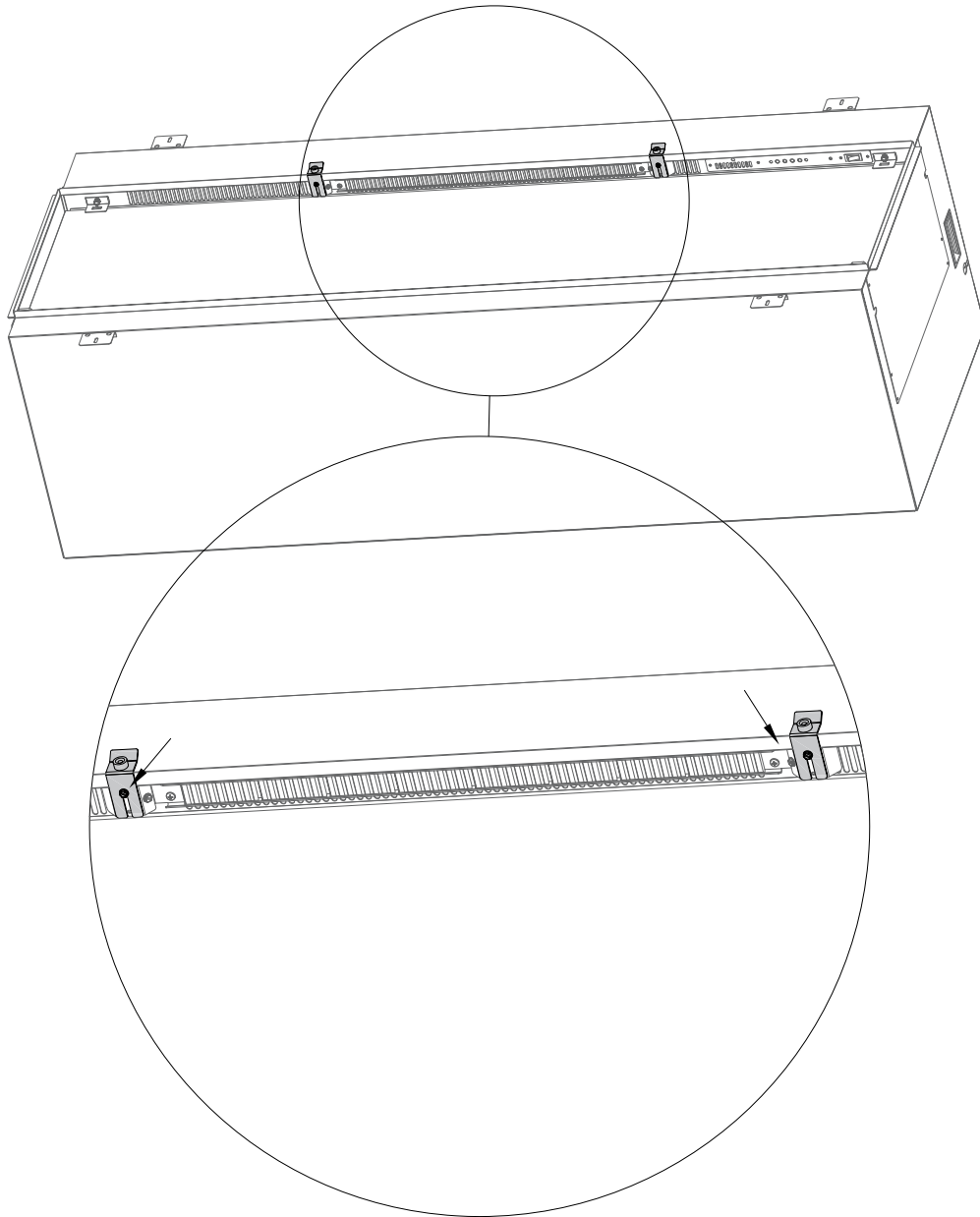
Figure 2.12 - Hanging Brackets
