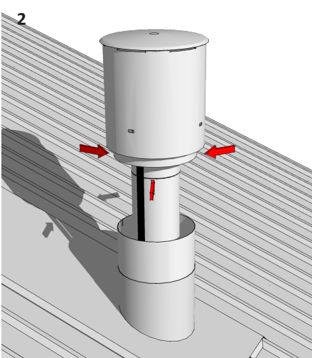
2 Install roof penetration flashing per local regulations. Attach 4" x 6 5/8" vent pipe to Power Vent Terminal. Connect Power Cable to fireplace, ensuring wiring by qualified electrician.
