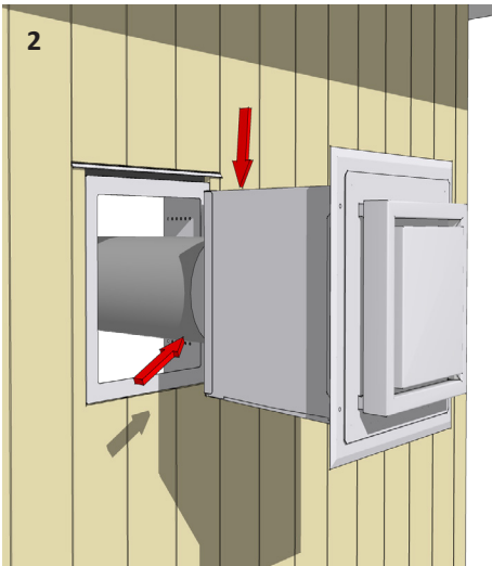
2 Attach the 4" x 6 5/8" vent pipe to the Vertical Power Vent Terminal. Connect the supplied power cable to the fireplace, with all wiring performed by a qualified electrician. Complete the wall siding installation, ensuring weathertightness in accordance with local building codes.
