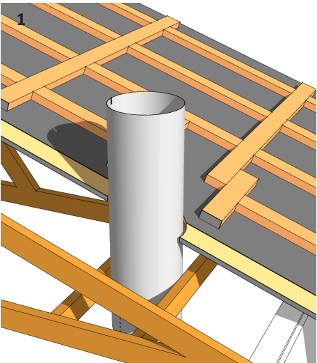
1 Locate and clear the vent pipe centerline. Create a 12" roof hole for the 11" vent liner, ensuring proper combustible material clearances and heights are met, as required.
