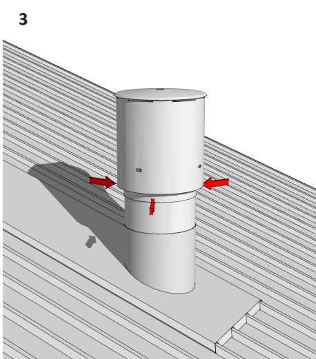
3 Fit the Vertical Power Vent Terminal onto the 11" Vent Liner and, seal and secure in place.
