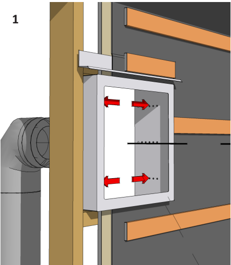
1 Establish the vent pipe centerline for the Horizontal Power Vent terminal, ensuring external clearances are met. Construct a 14 1/2" framework inside the wall, following minimum combustible clearance guidelines. Install the wall thimble into the wall to align with the siding.
