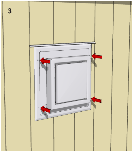
3 Install the Horizontal Power Vent Terminal onto the wall thimble, securely sealing and screwing it into place.
