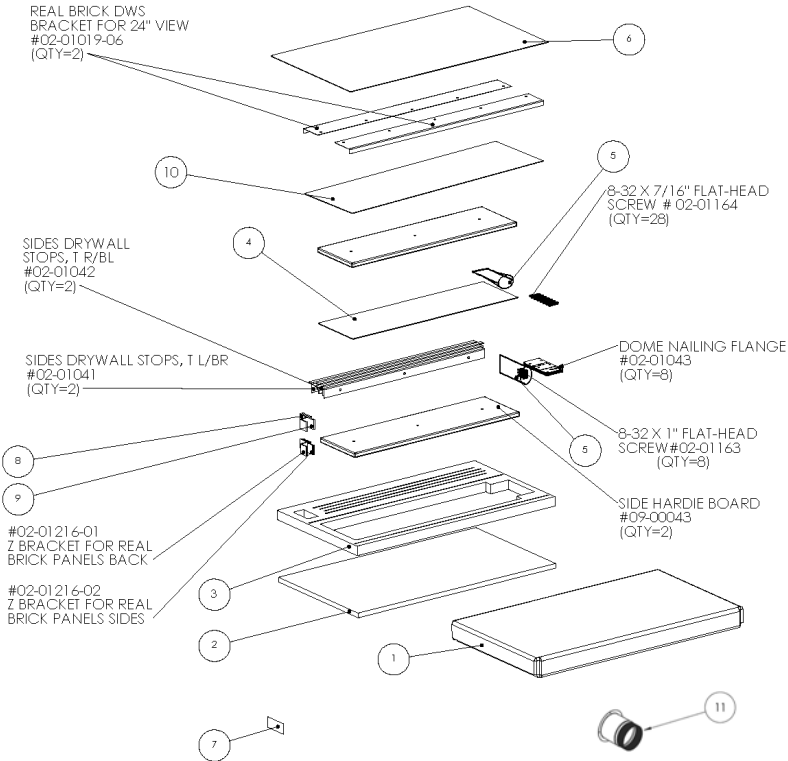
Figure 56 - Accessory Kit
