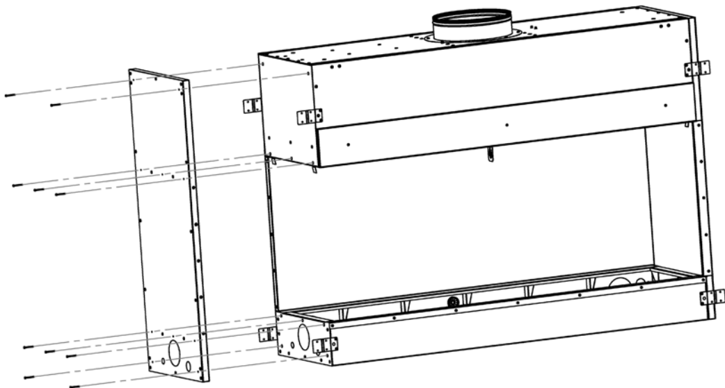
Step 2. Removing left side panel.
