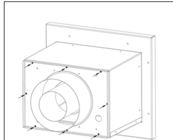
Figure 6.1 - Rear Plate Screws
