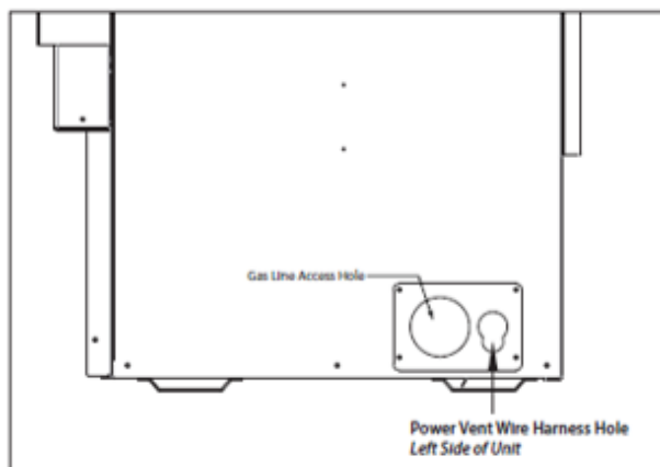
Figure 6.14 - Power Vent Wire Harness Hole Location (Callaway 40 Shown)
