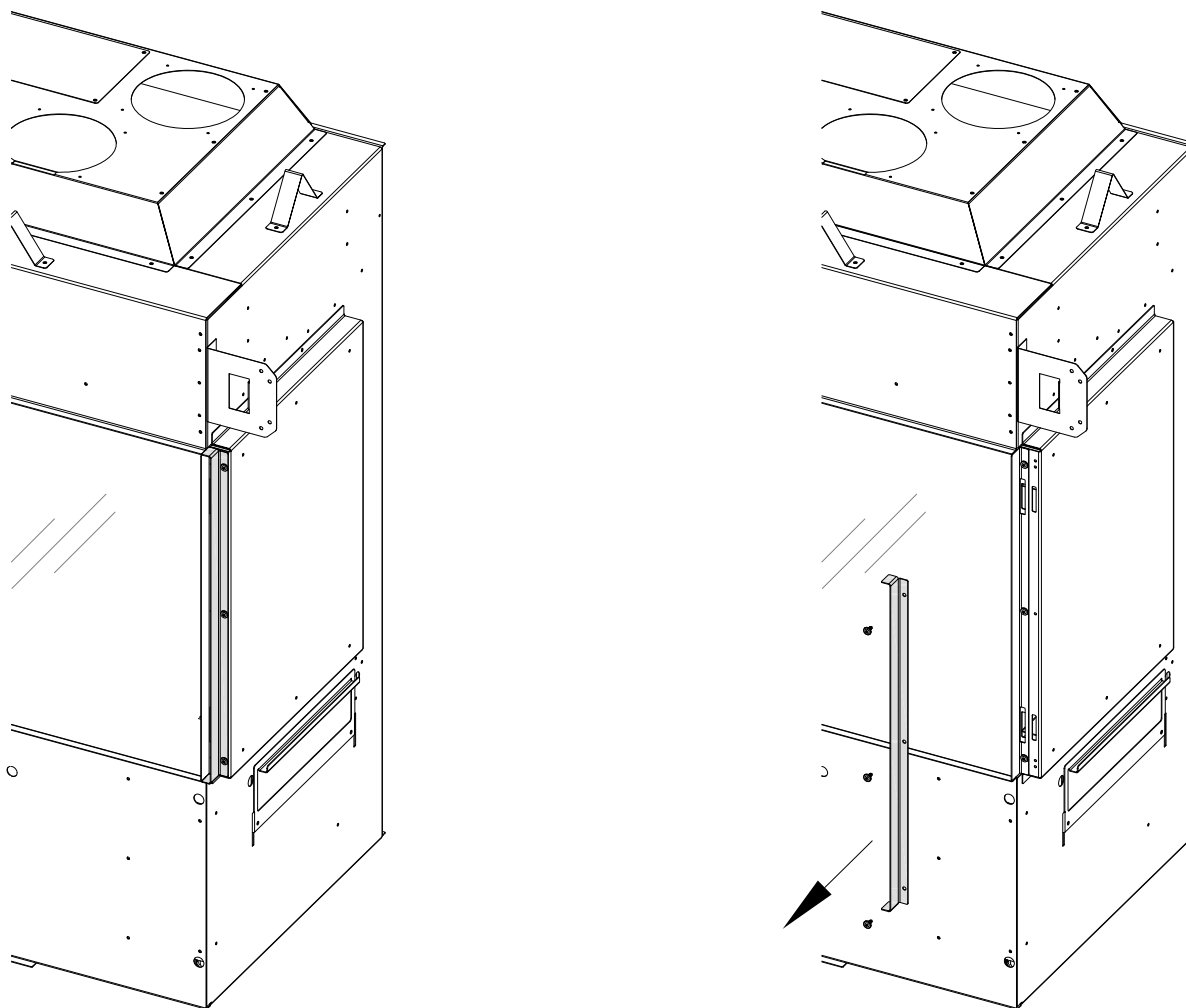
Figure 4.12 - Side Finishing Edge Extension - Rectangle Surround
