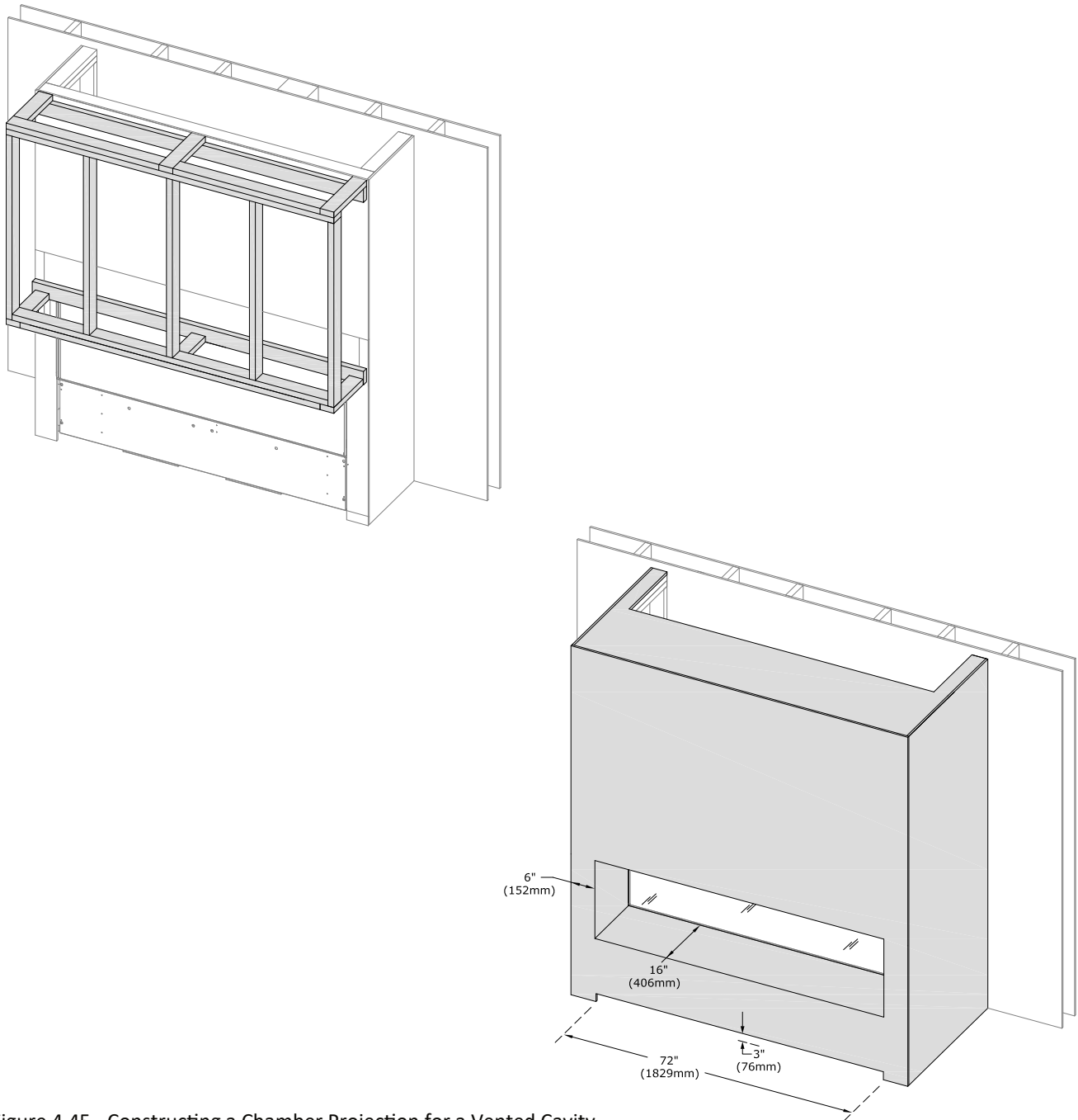
Figure 4.45 - Constructing a Chamber Projection for a Vented Cavity
