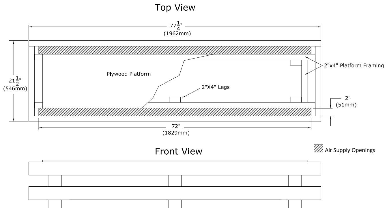
Figure 4.7 - Elevated Platform Air Openings
