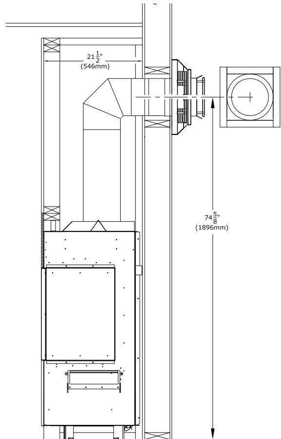
Figure 4.10 - Minimum Wall Thimble Framing
