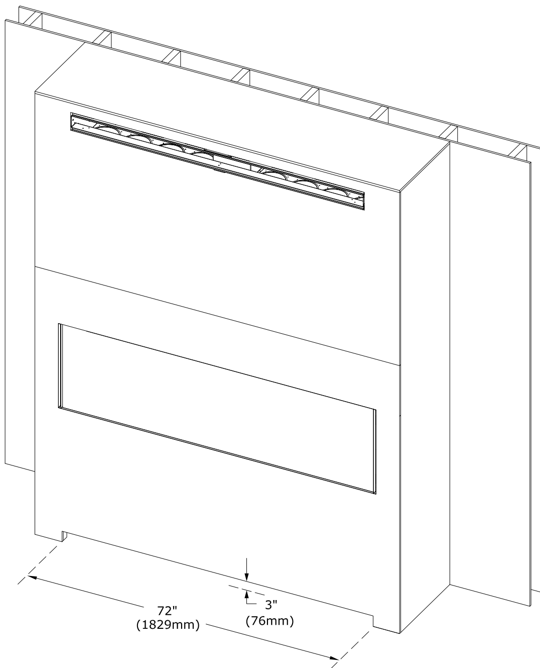
Figure 4.19 - Minimum Air Intake Opening
