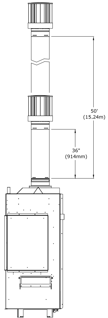
Figure 6.6 - 4"x6-5/8" Vertical Vent Pipe
