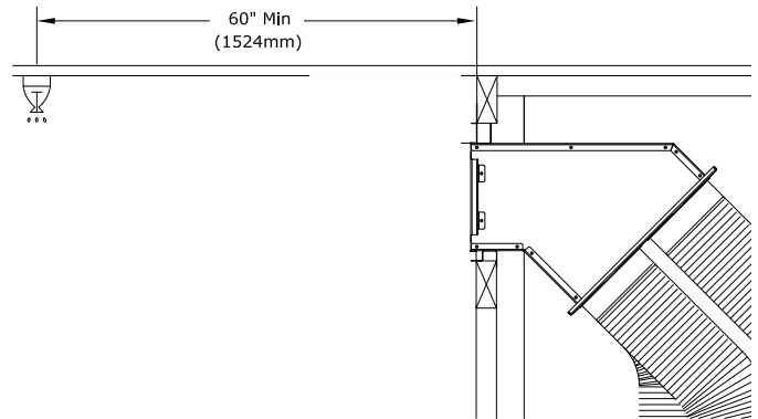
Figure 4.9 - Clearance to Sprinkler
