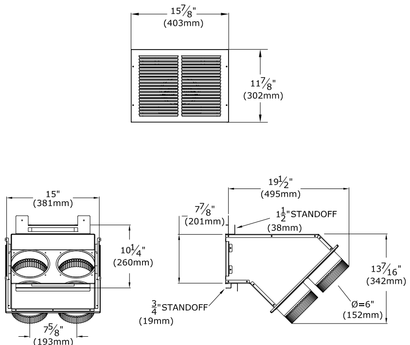
Figure 4.23 - KZK-1510B Overview
