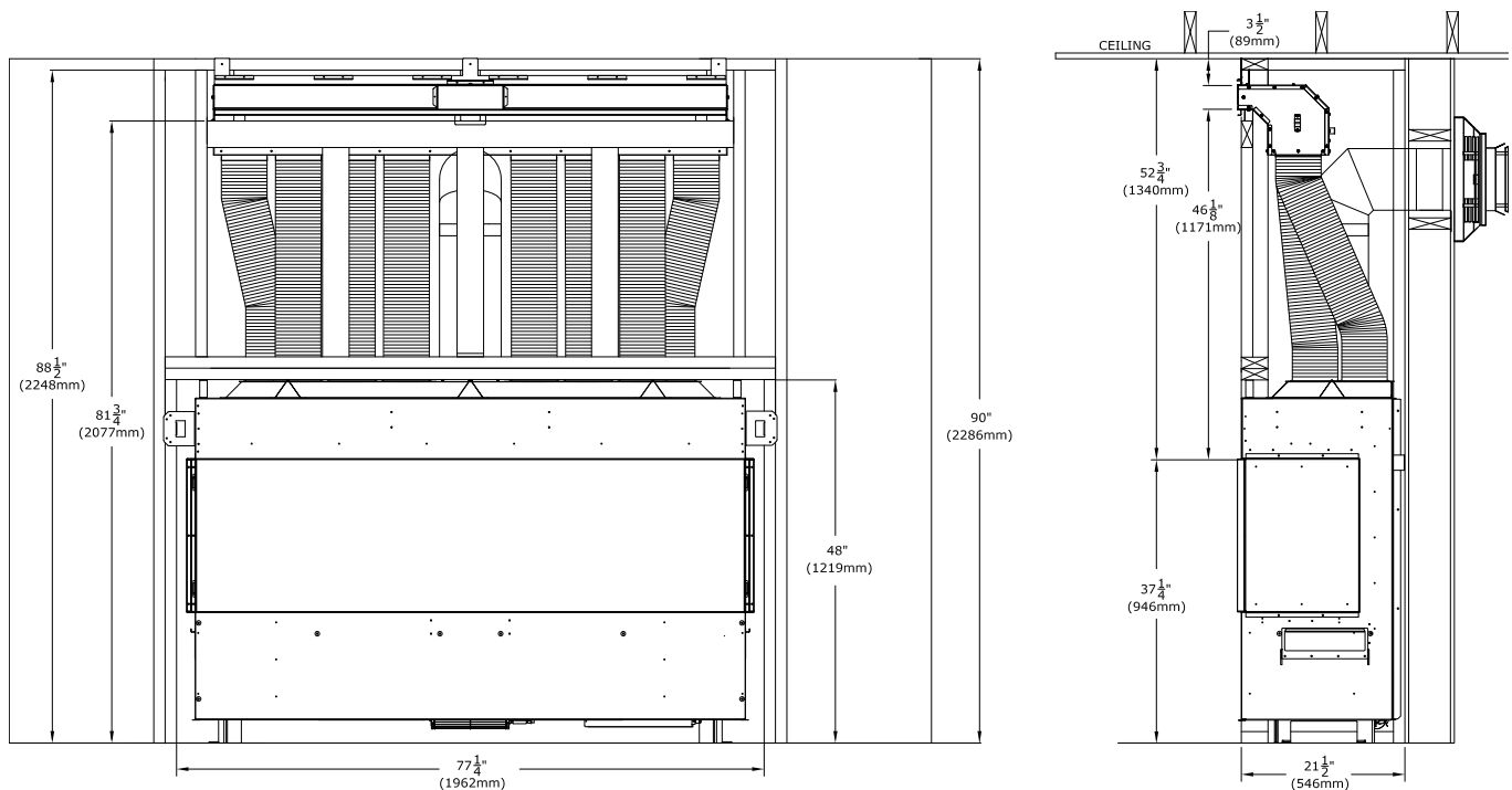
Figure 4.18 - Minimum Chamber Height Plenum Framing
