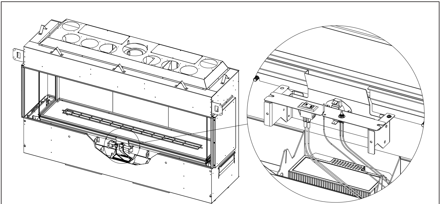
Figure 7.18 - Switch Panel
