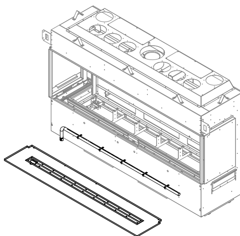
Figure 7.10 - Burner Media Tray and Burner Tube Removal
