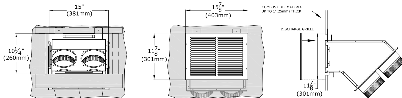
Figure 4.27 - KZK Grille - Finishing Options
