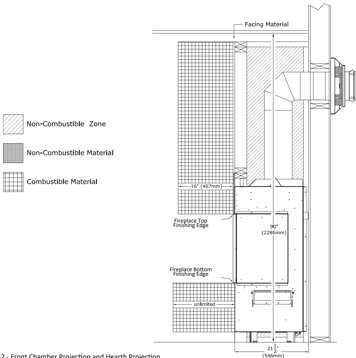
Figure 4.42 - Front Chamber Projection and Hearth Projection
