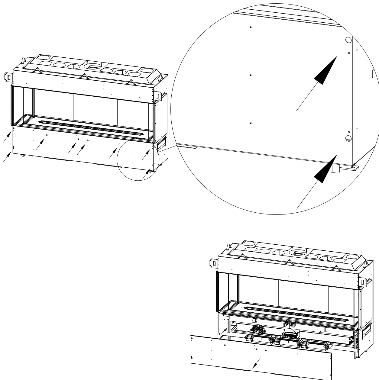
Figure 3.6 - Front Access Panel
