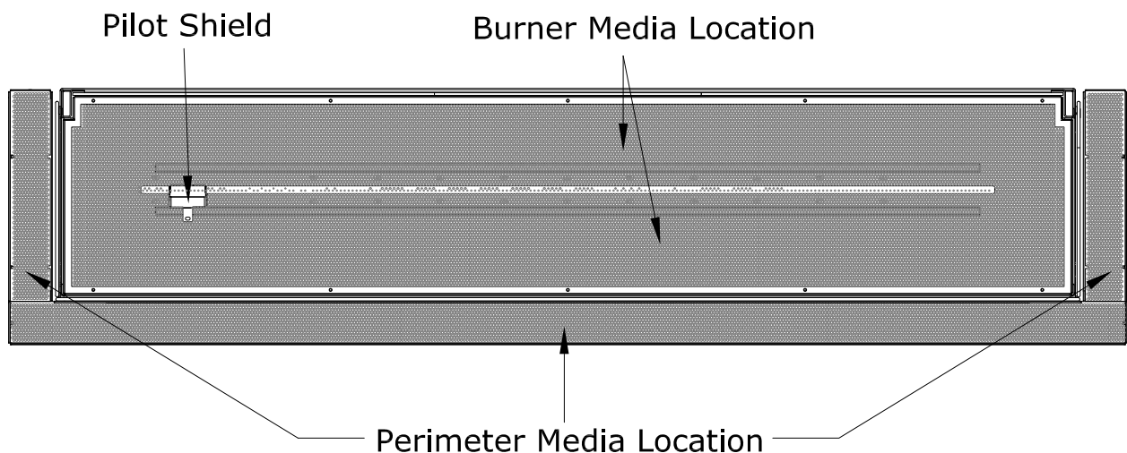
Figure 7.11 - Crushed Media Location
