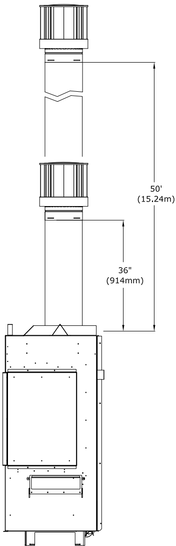
Figure 6.5 - 5"x8" Vertical Vent Pipe
