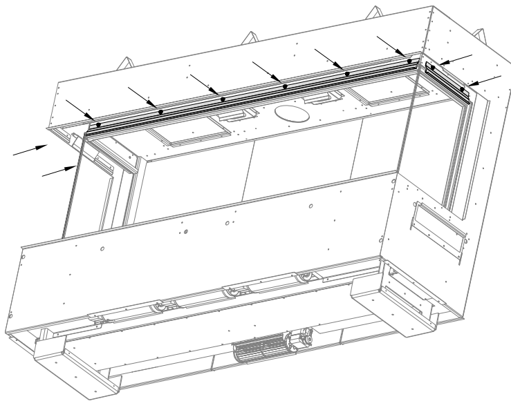
Lower Glass Brackets
