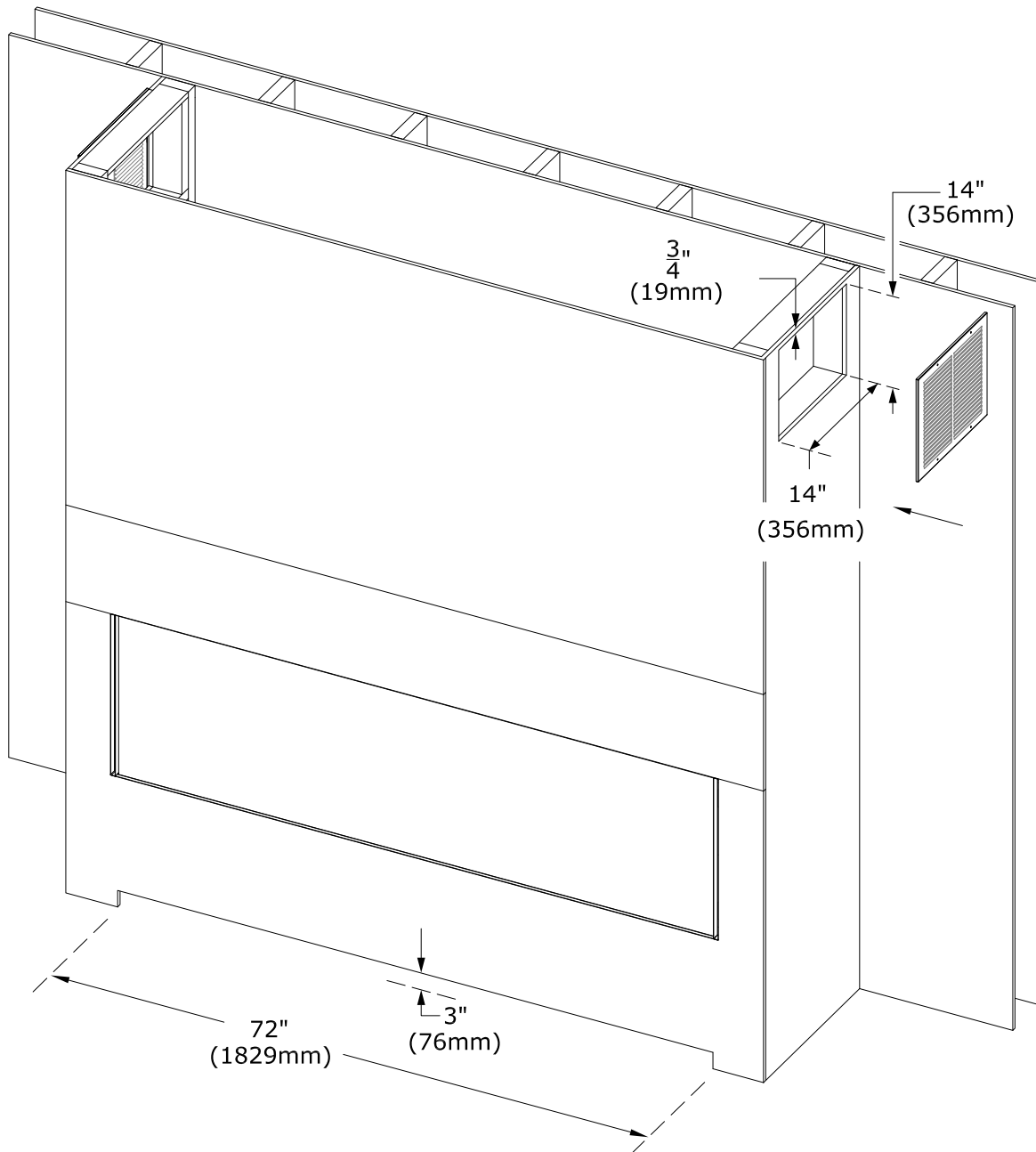
Figure 4.36 - Heat Release - Side Opening Option
