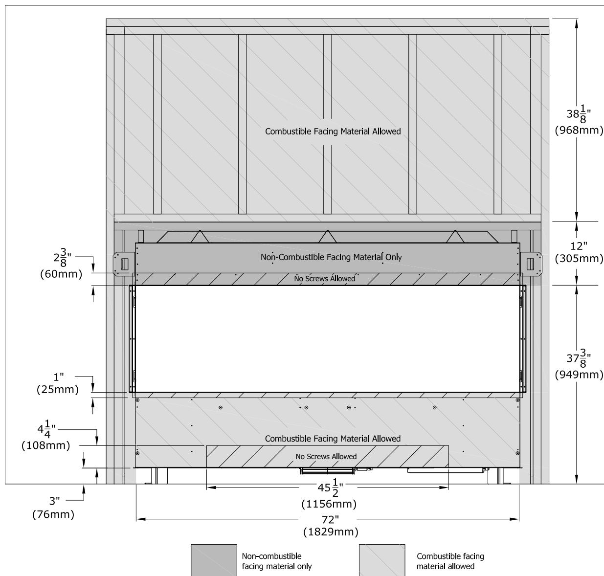
Figure 4.11 - Facing Material Requirements
