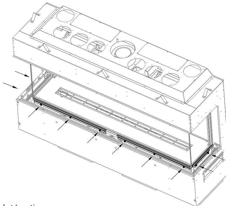
Figure 7.5 - Glass Bracket Location
