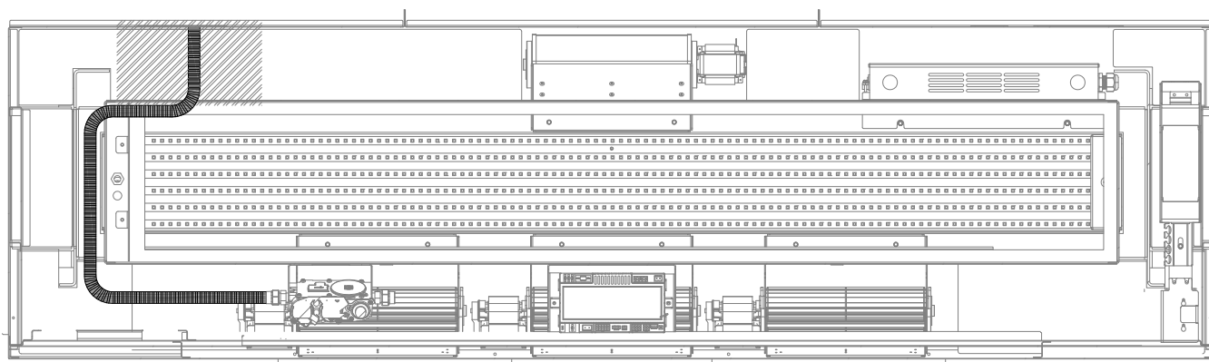
Figure 5.1 - Gas Line Path (Top View)
