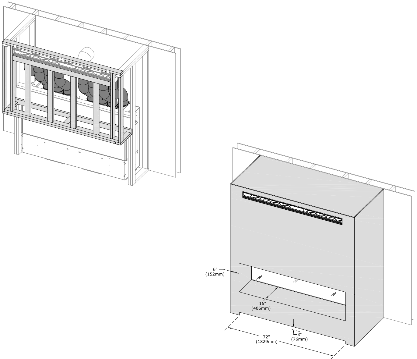
Figure 4.40 - Constructing a Chamber Projection with a KZK
