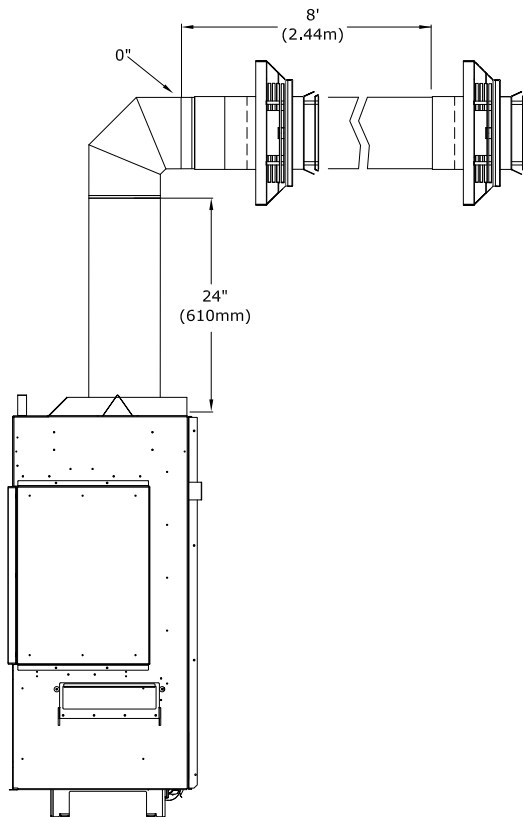
Figure 6.7 - Horizontal Terminations
