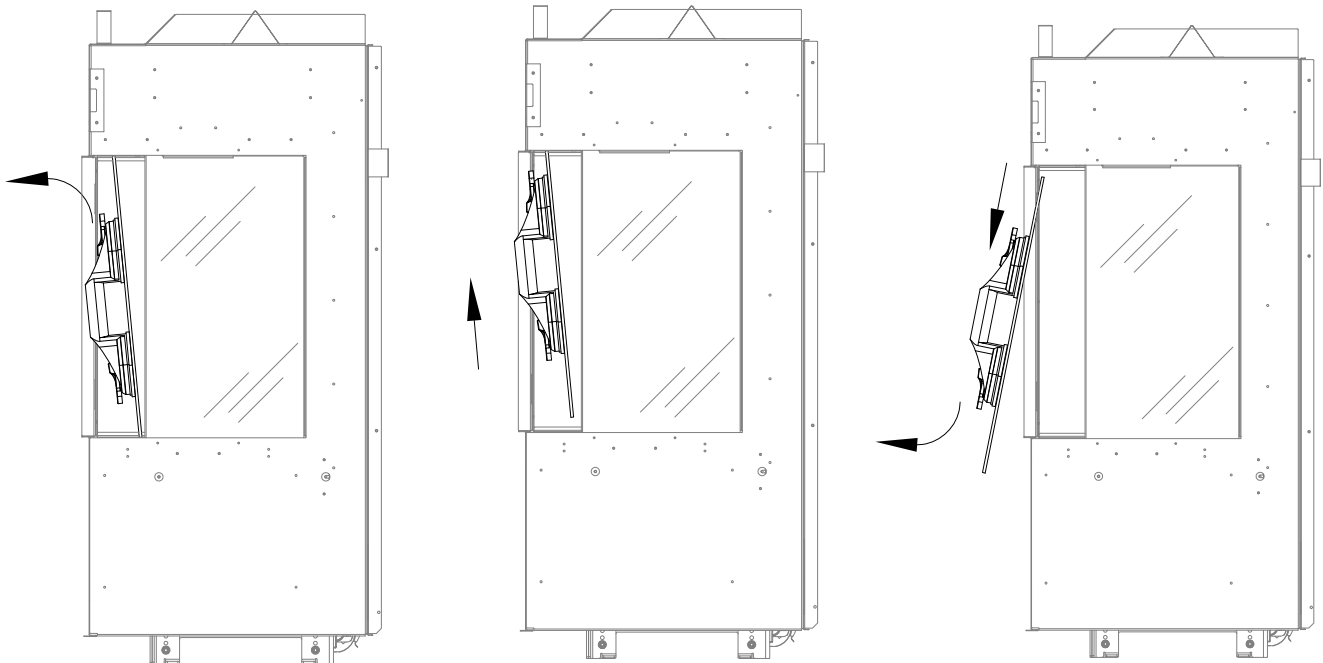
Figure 7.4 - Firebox Glass Removal
