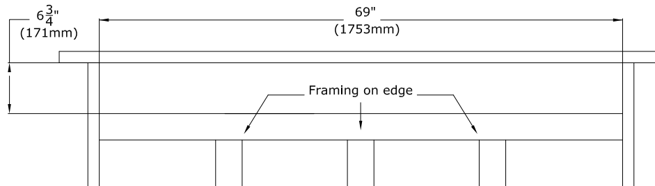
Figure 4.17 - Front KZK - Plenum Framed Opening
