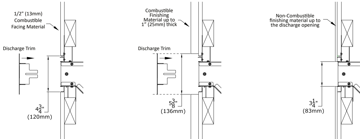
Figure 4.20 - KZK Plenum Air Discharge Opening - Finishing Options
