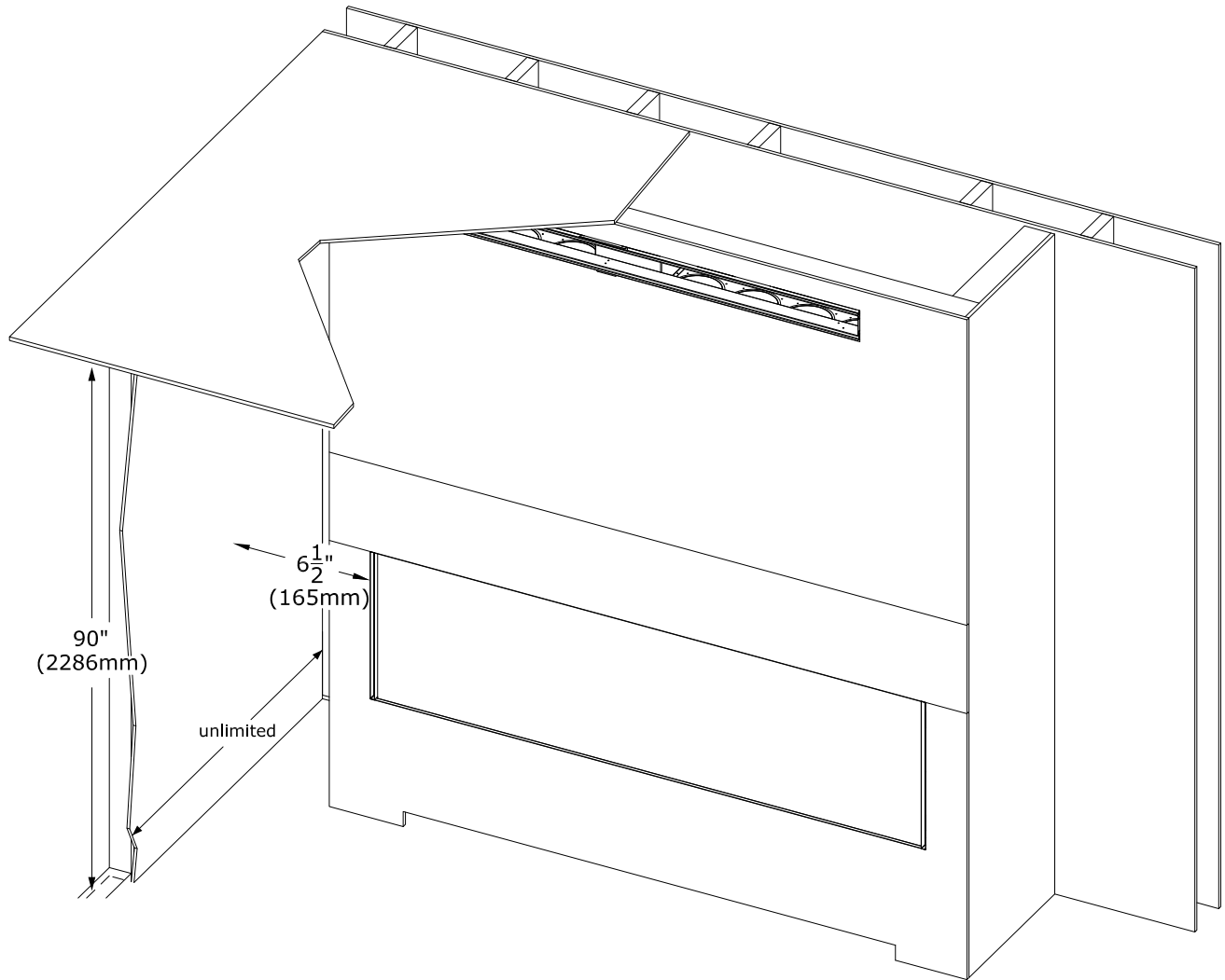
Figure 4.46 - Clearance to Sidewall
