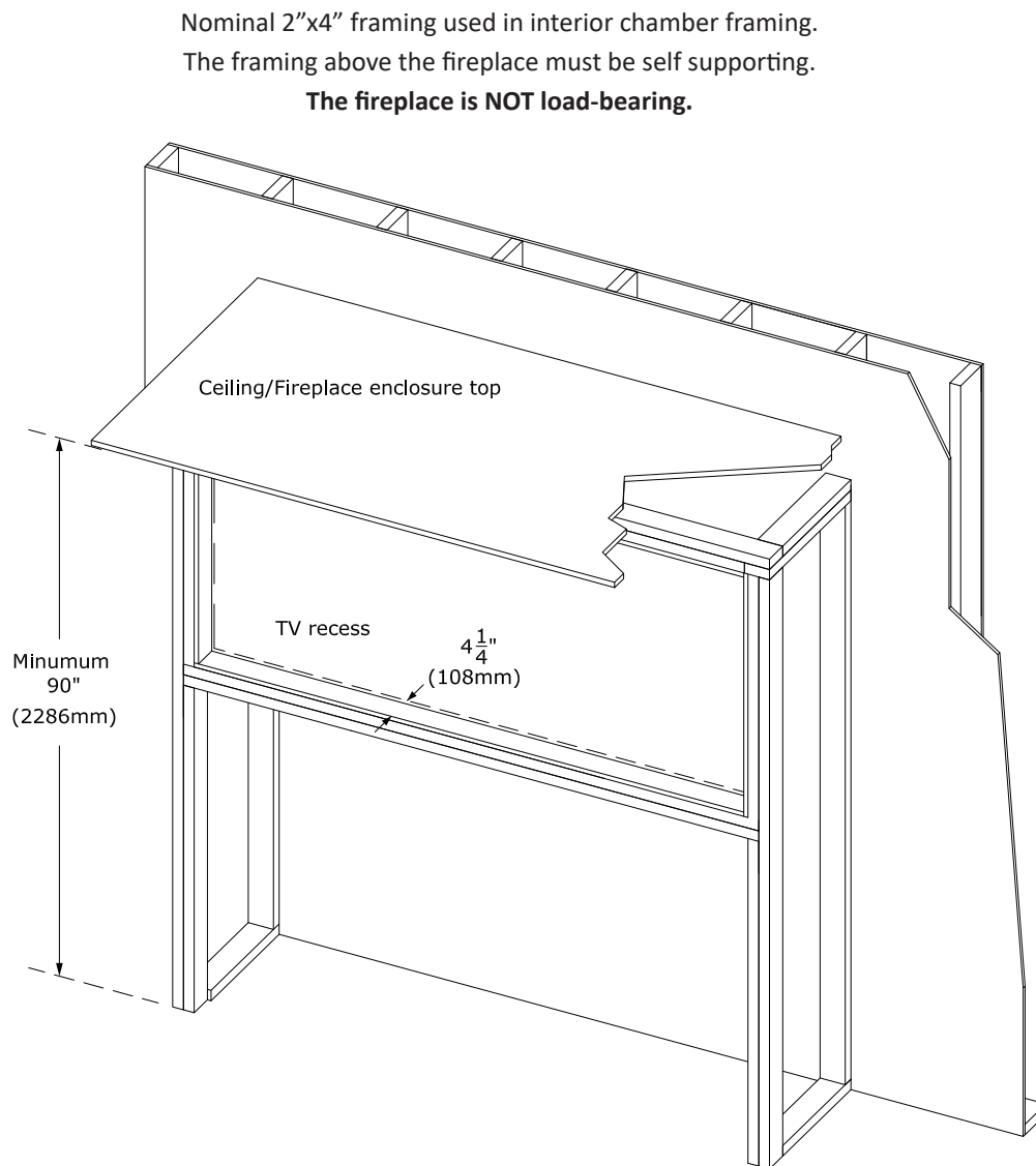
Figure 4.2 - Recess TV Installation
