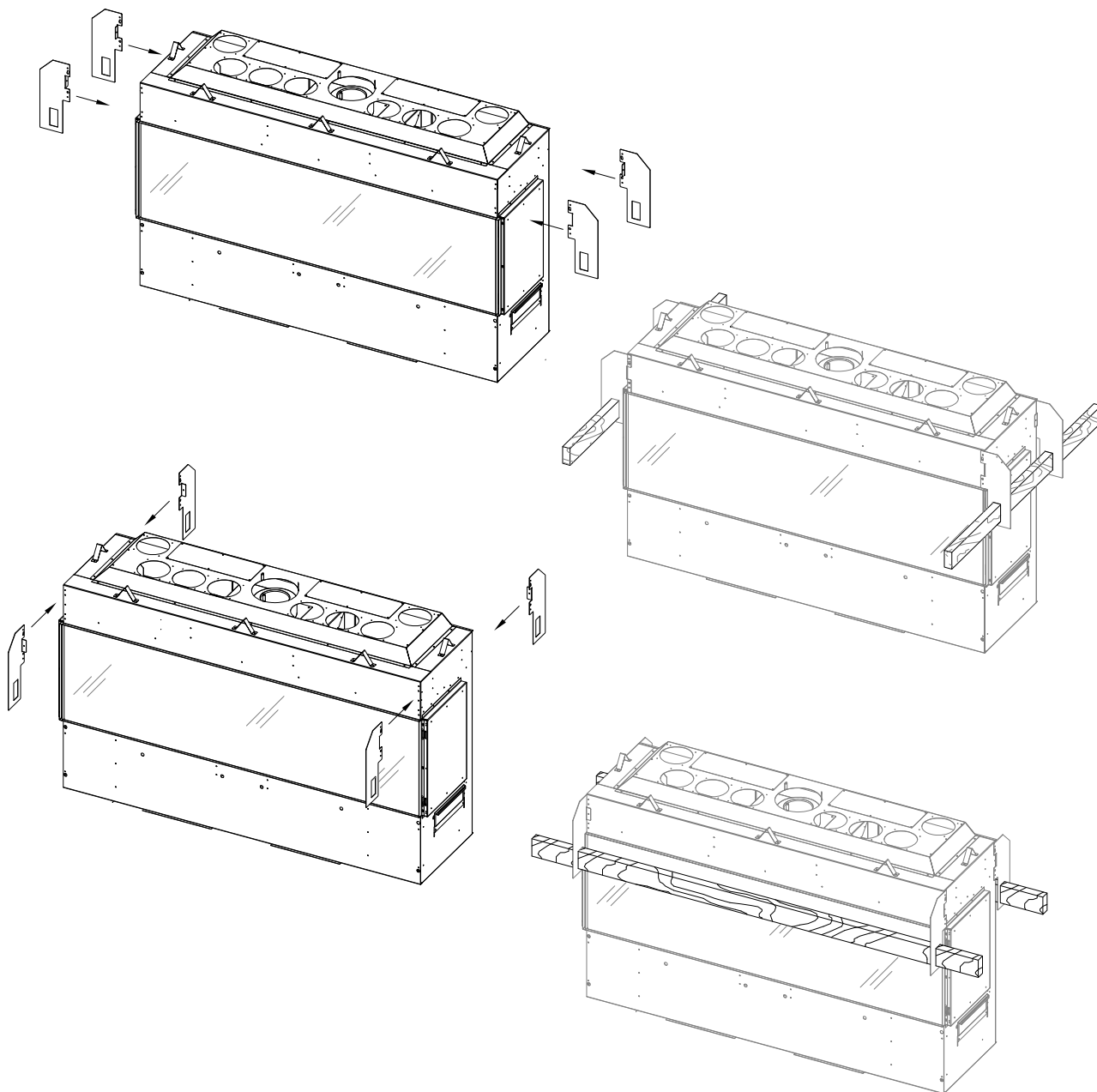
Figure 3.2 - Installation and Use of 2x4 Lifting Handles
