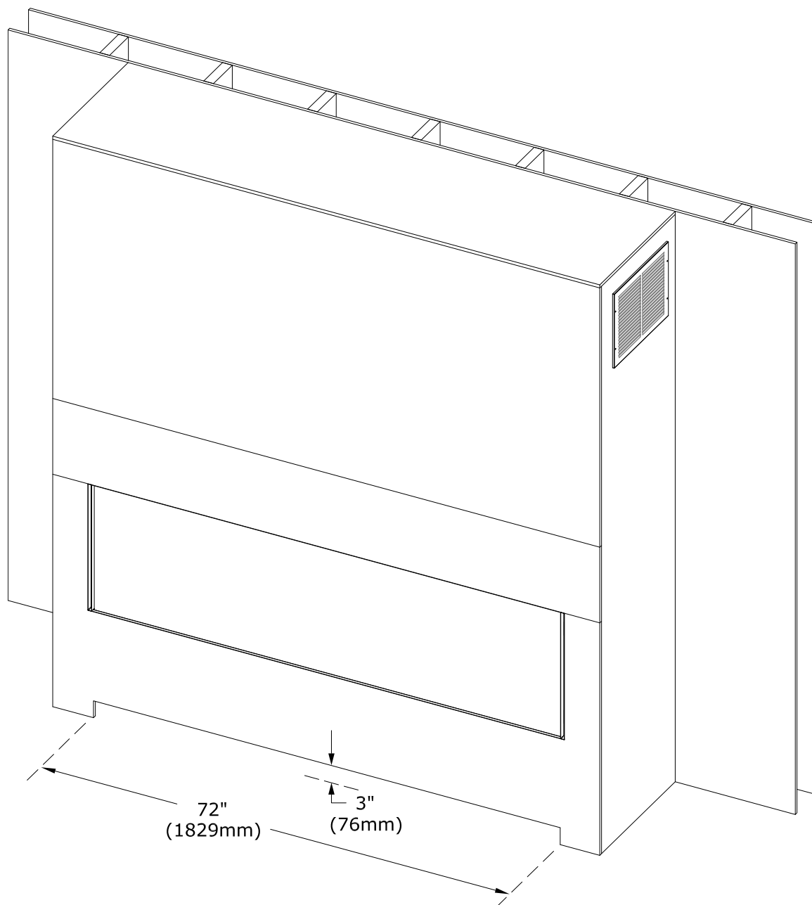
Figure 4.26 -Minimum Air Intake Opening
