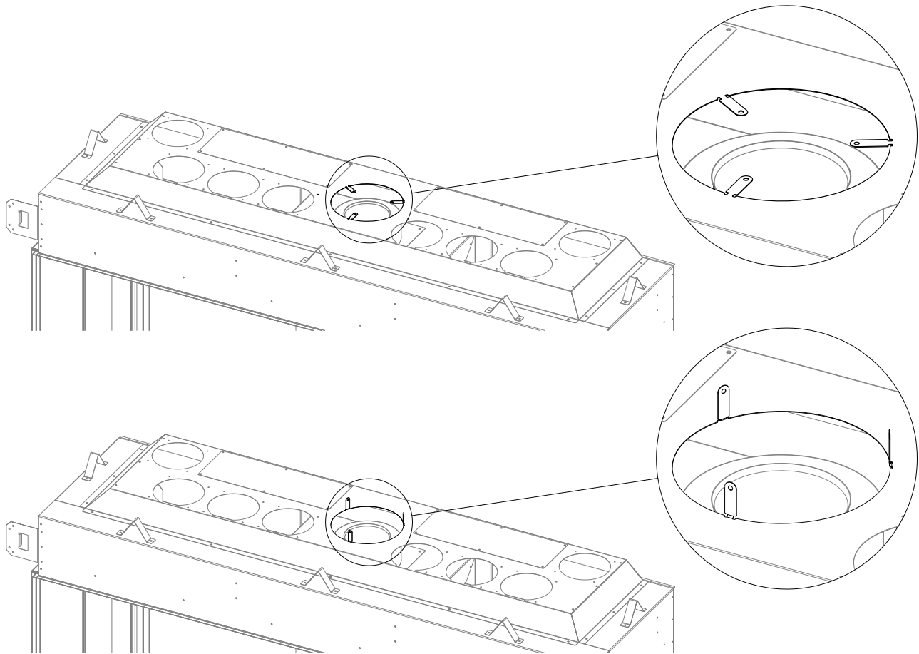
Figure 6.11 - Vent Tabs
