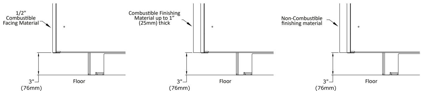
Figure 4.21 - Fireplace Chamber Air Intake Opening - Finishing Options
