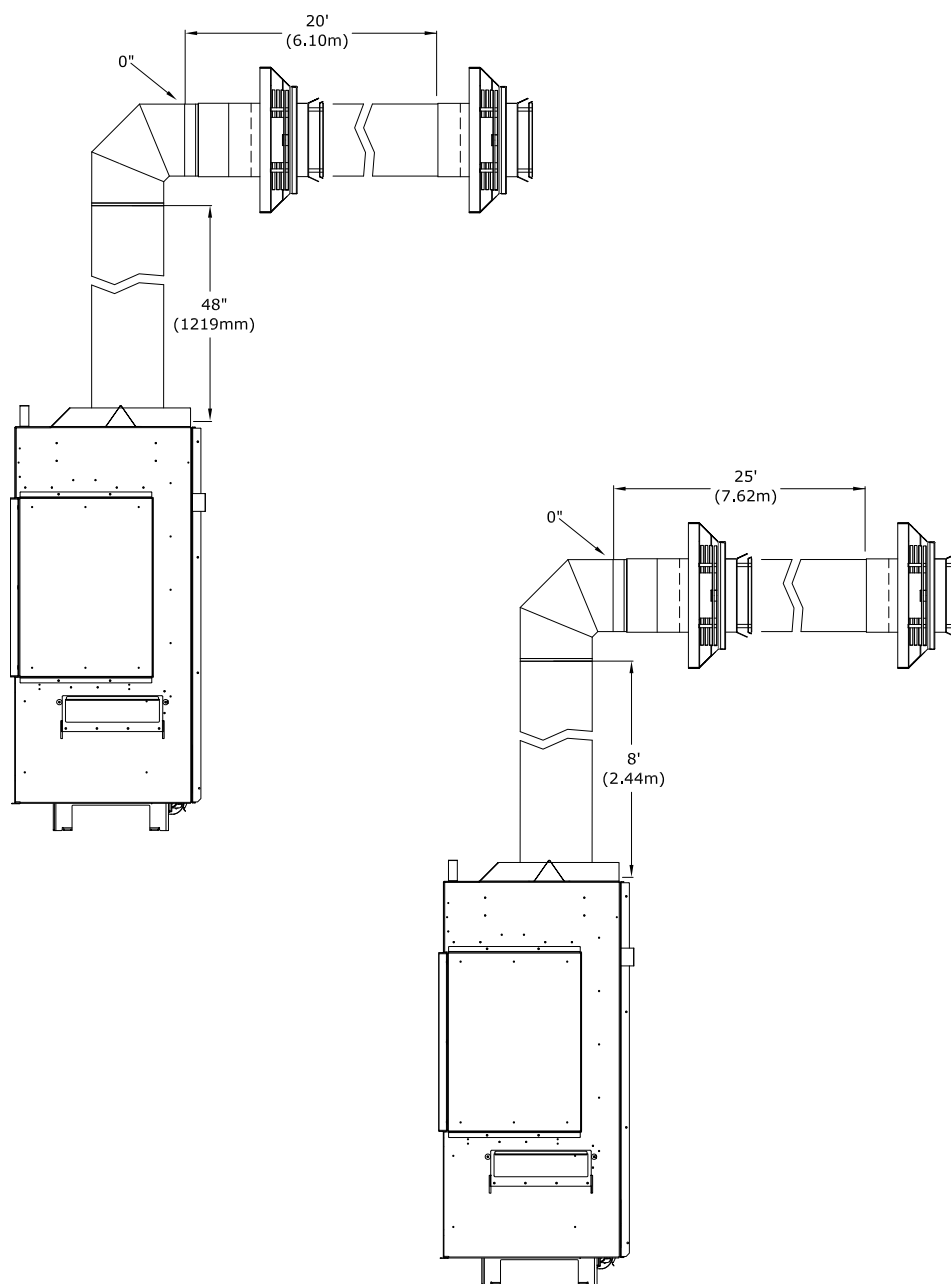
Figure 6.8 - Horizontal Terminations
