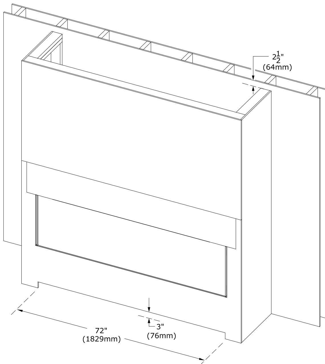
Figure 4.30 - Air Openings - Three-Sided Installation
