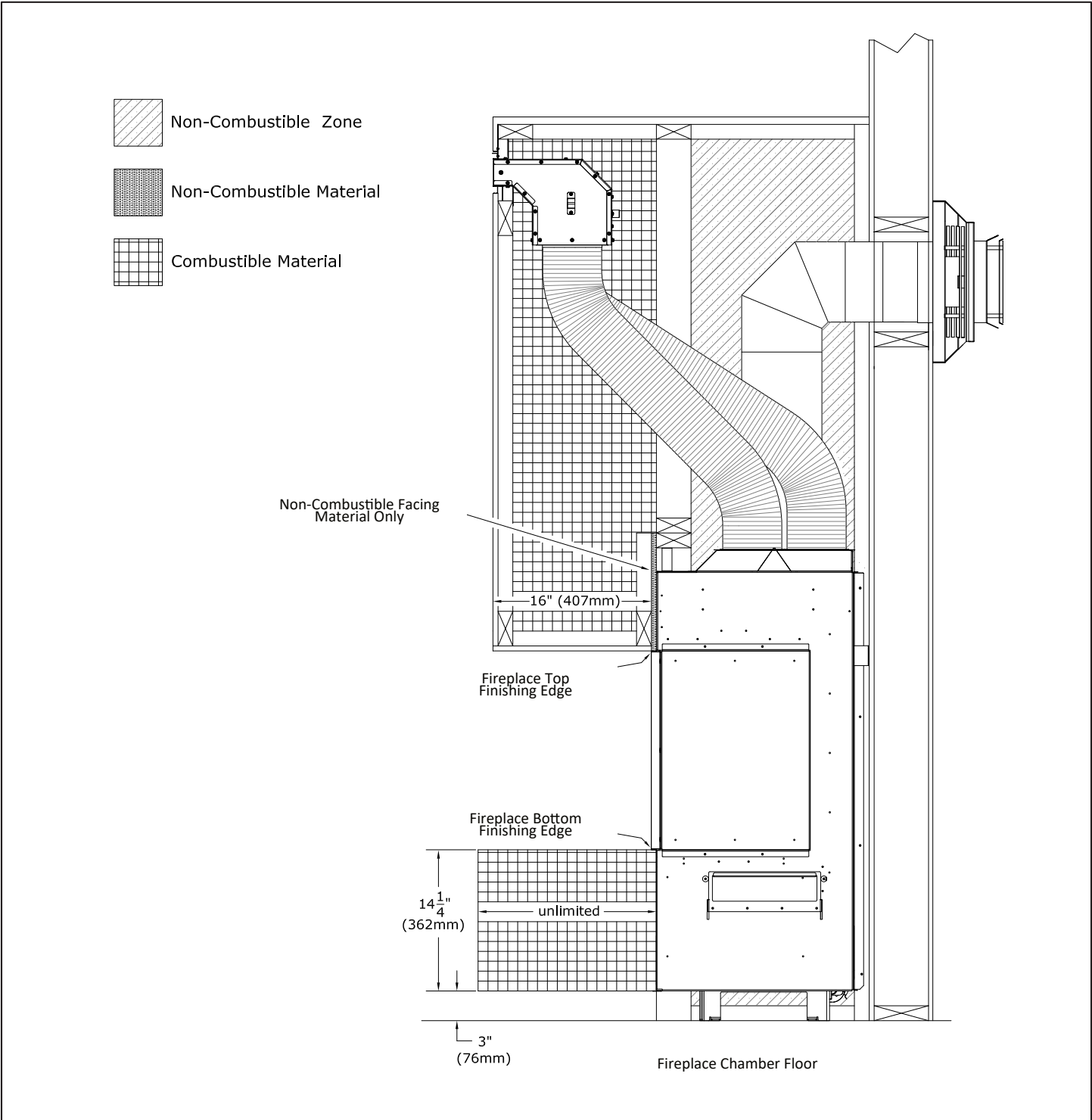
Figure 4.38 - Front Chamber Projection and Hearth Projection
