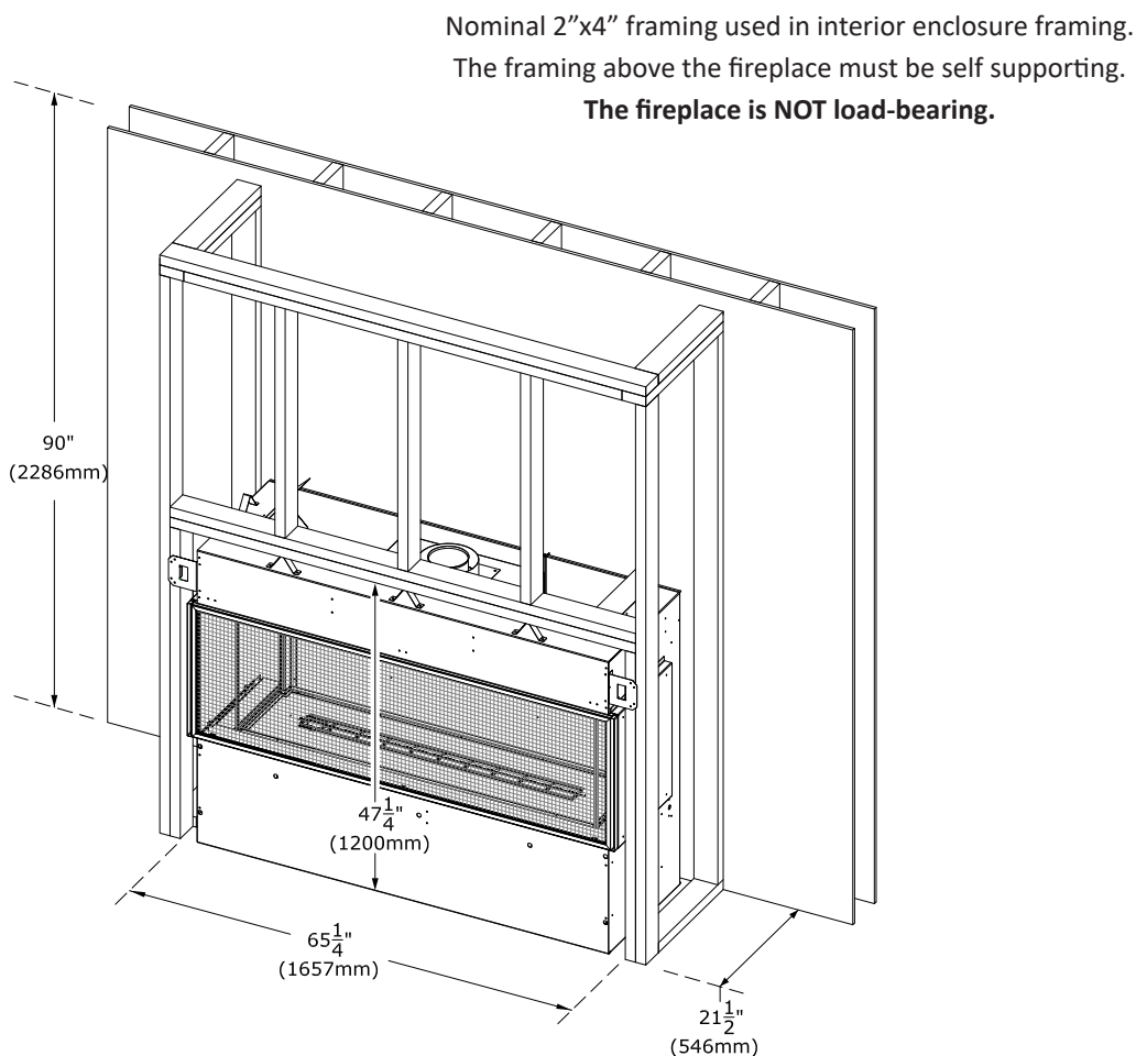
Figure 4.1 - Framing Requirements
