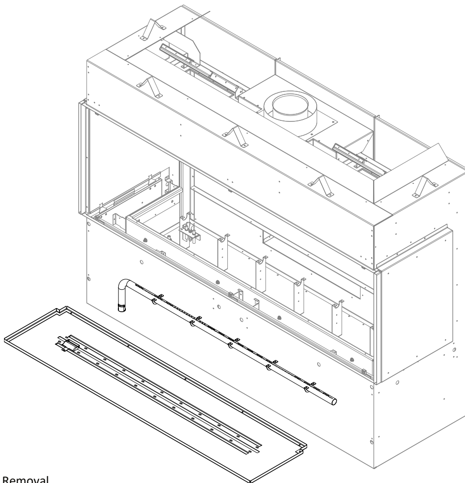
Figure 7.9 - Burner Removal
