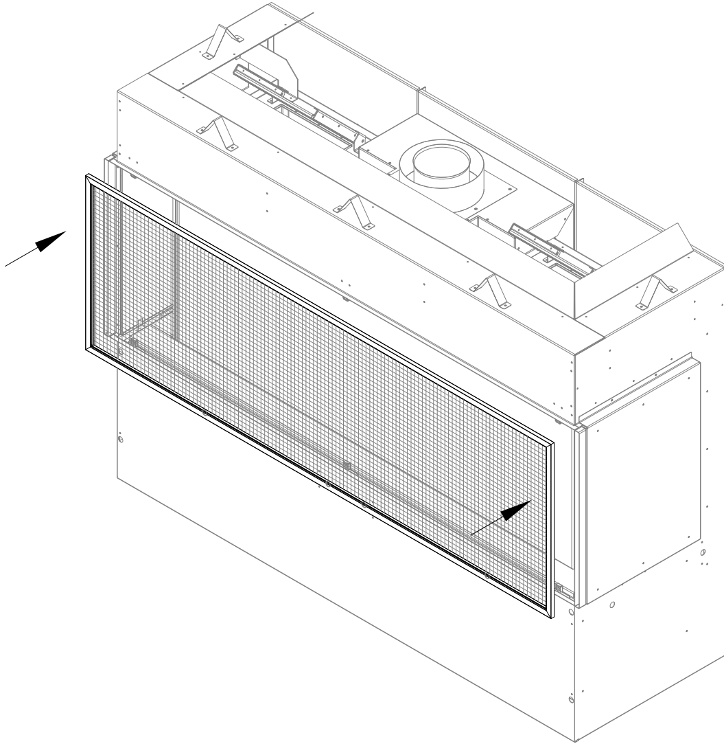
Figure 7.2 - Safety Screen Installation
