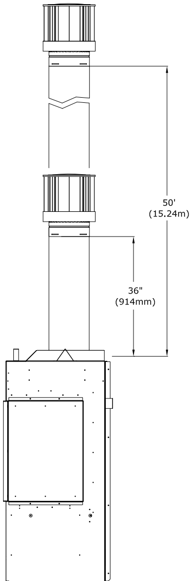
Figure 6.5 - 5"x8" Vertical
