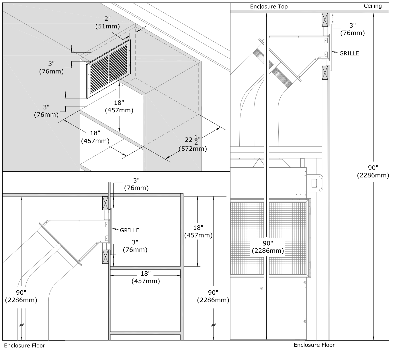
Figure 4.36 - Clearance to Sidewall
