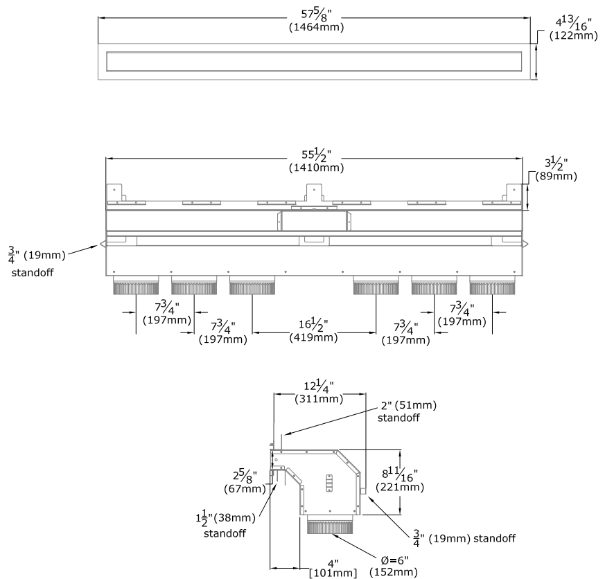
Figure 4.10 - KZK Overview
