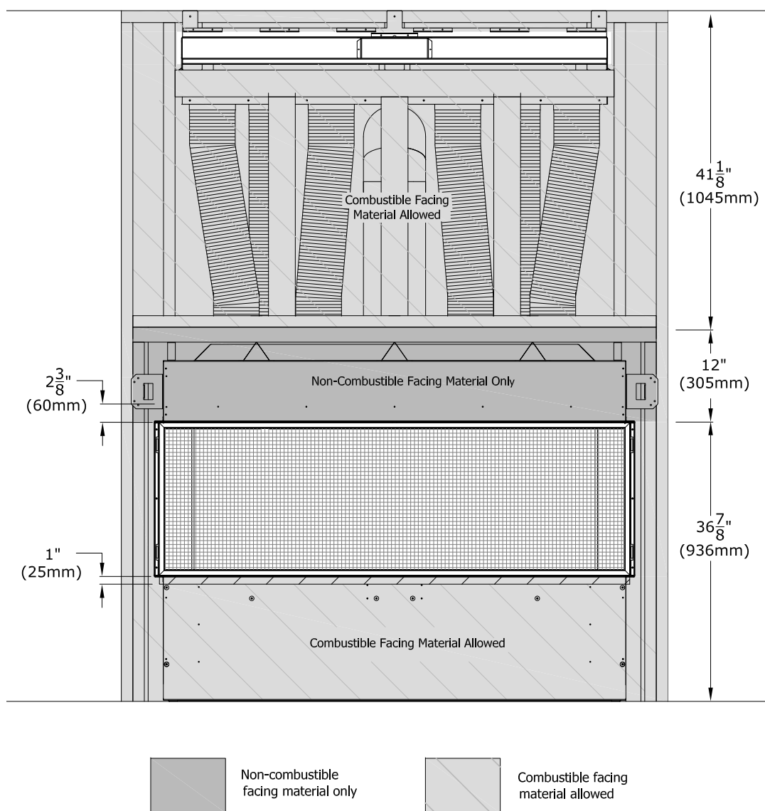
Figure 4.6 - Facing Material Requirements
