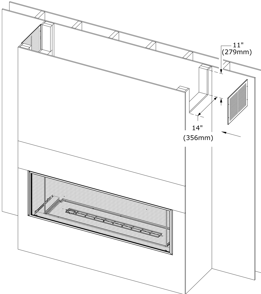
Figure 4.26 - Heat Release - Side Opening
