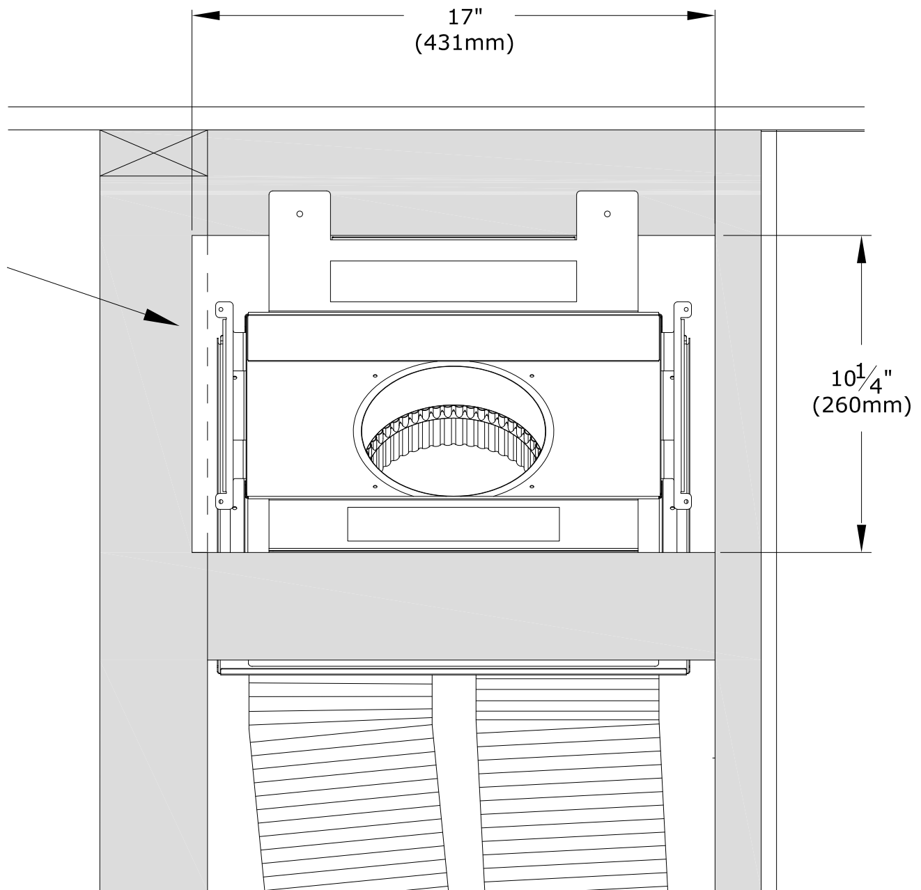
Figure 4.16 - Side KZK - Plenum Framed Opening
