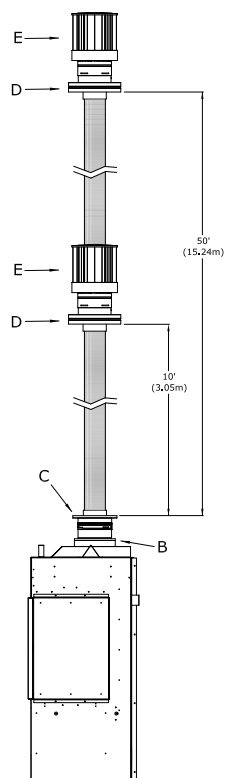
Figure 6.10 - Class A Chimney Conversion
