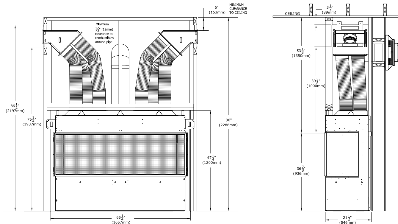
Figure 4.17 - Minimum Chamber Height Plenum Framing
