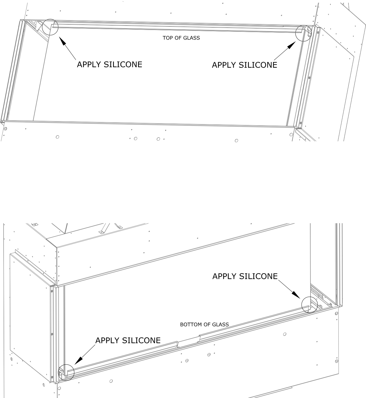
Figure 7.8 - Firebox Glass Corner Silicone Seal
