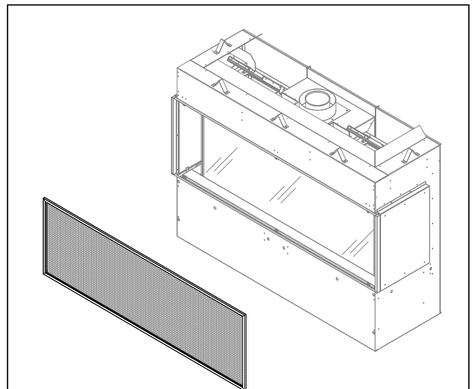
Figure 7.11 - Remove Safety Screen
