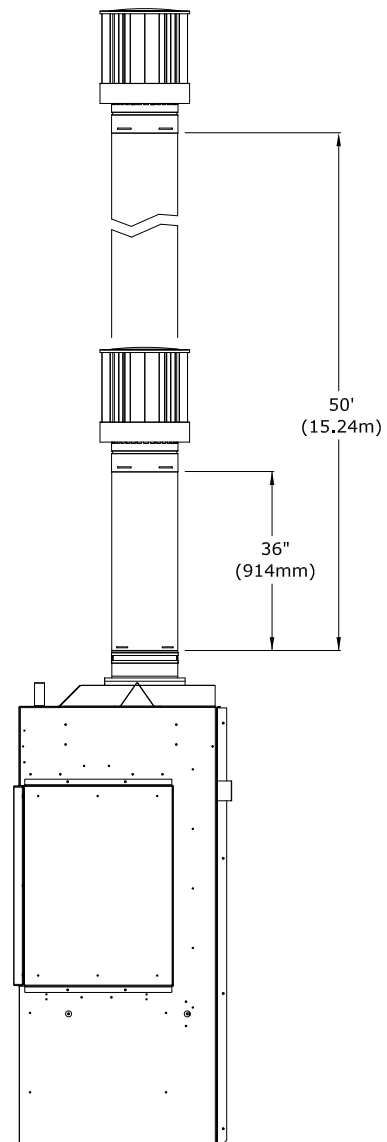
Figure 6.6 - 4"x6-5/8" Vertical
