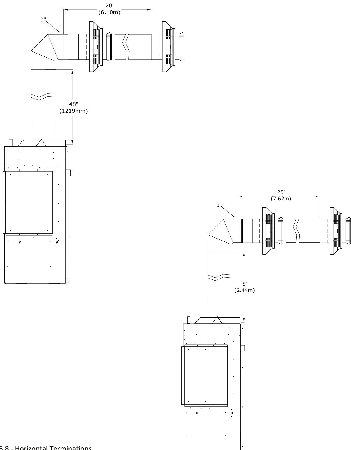
Figure 6.8 - Horizontal Terminations
