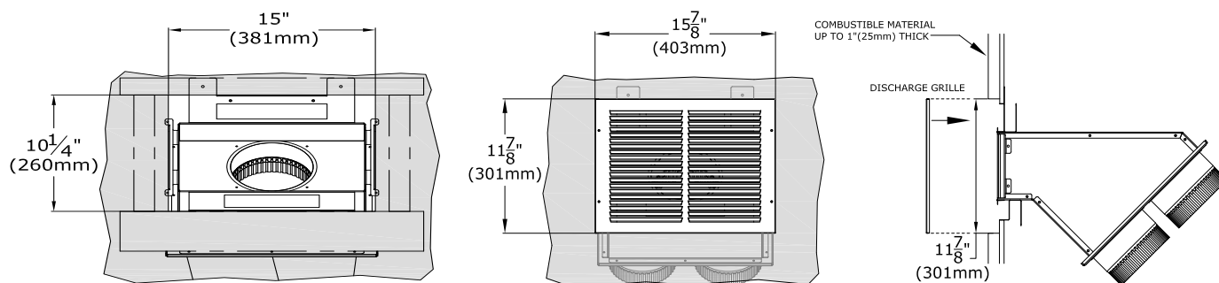
Figure 4.18 - KZK Grille - Finishing Options
