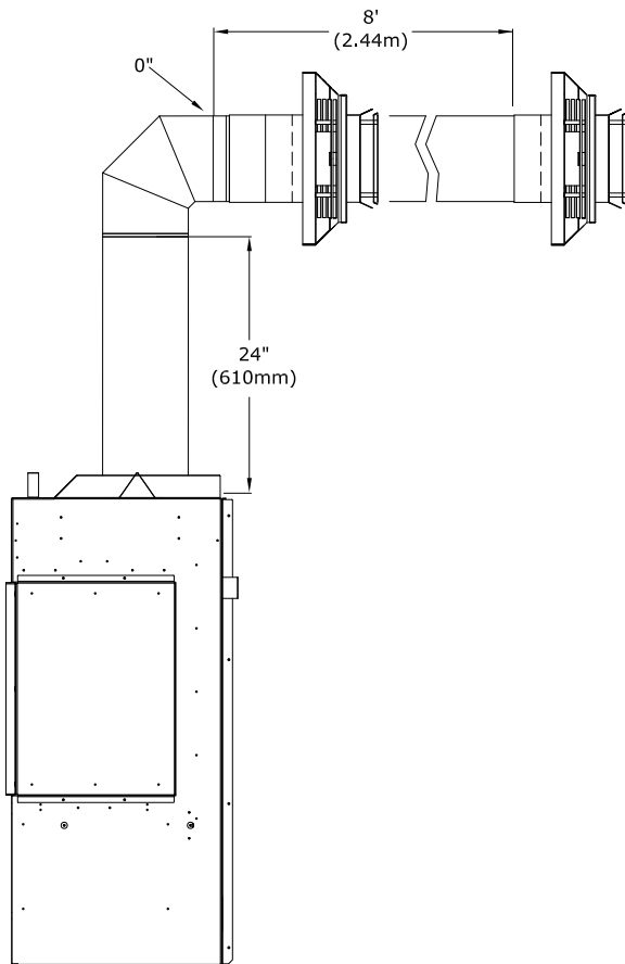
Figure 6.7 - Horizontal Terminations
