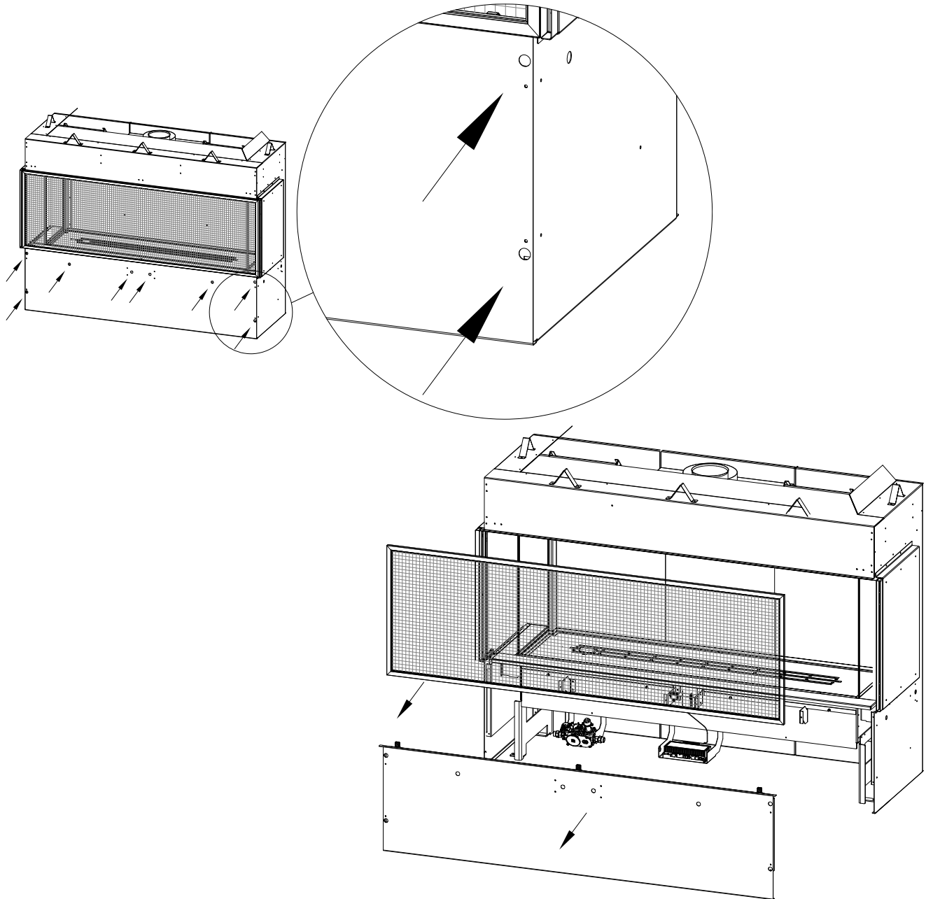
Figure 3.5 - Front Access Panel
