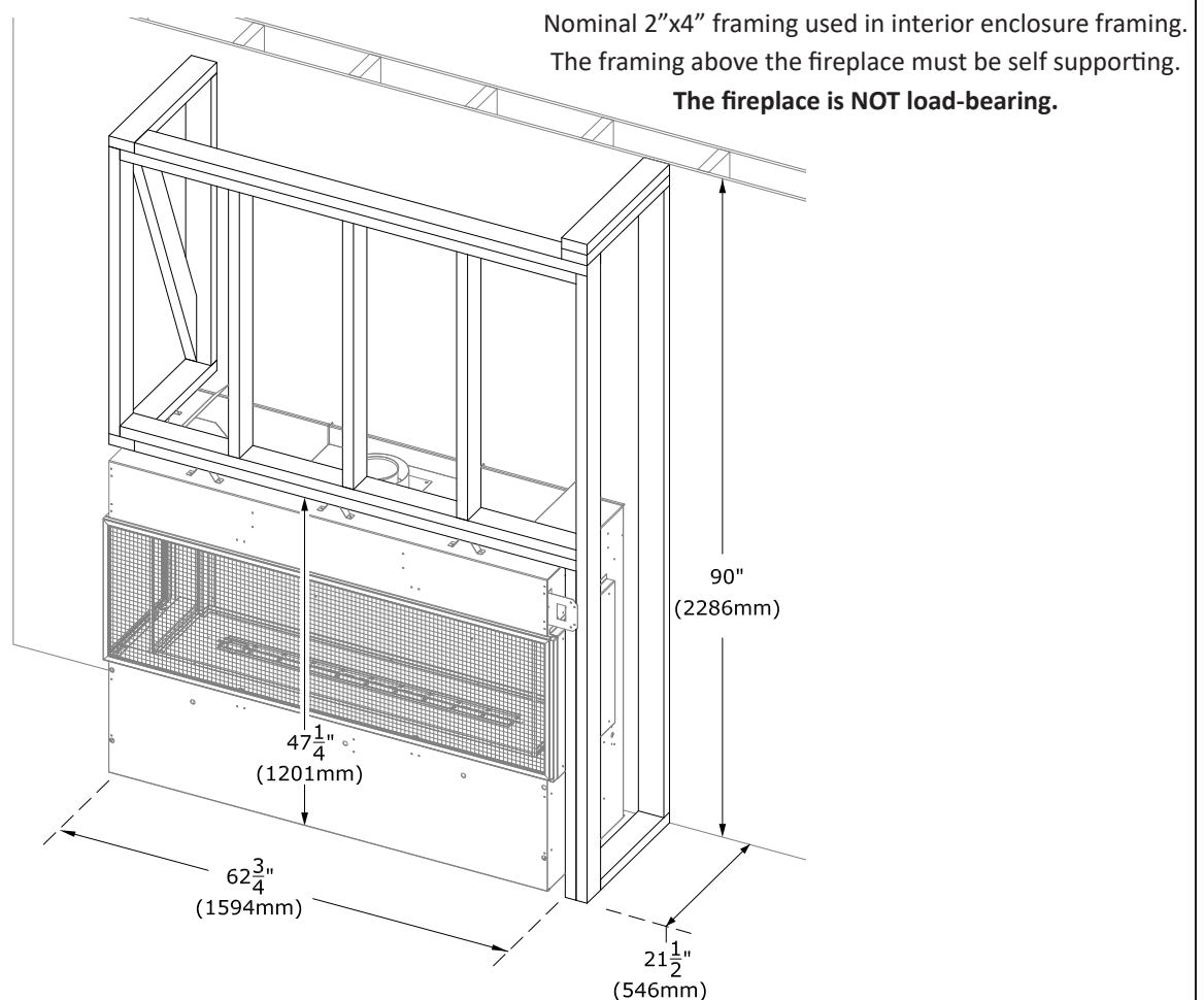
Figure 2.1 - Framing Requirements
