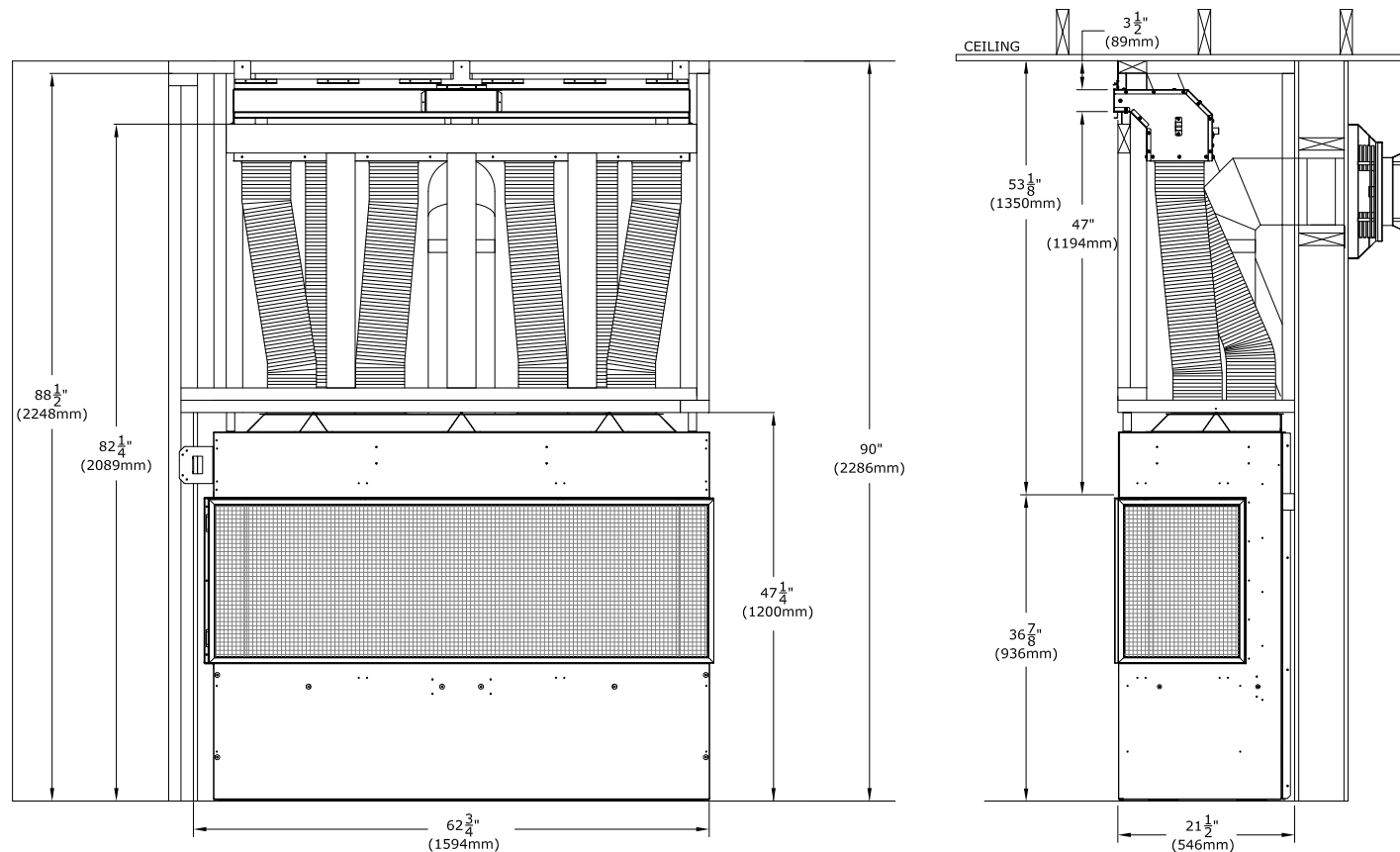
Figure 2.7 - Minimum Chamber Height Plenum Framing
