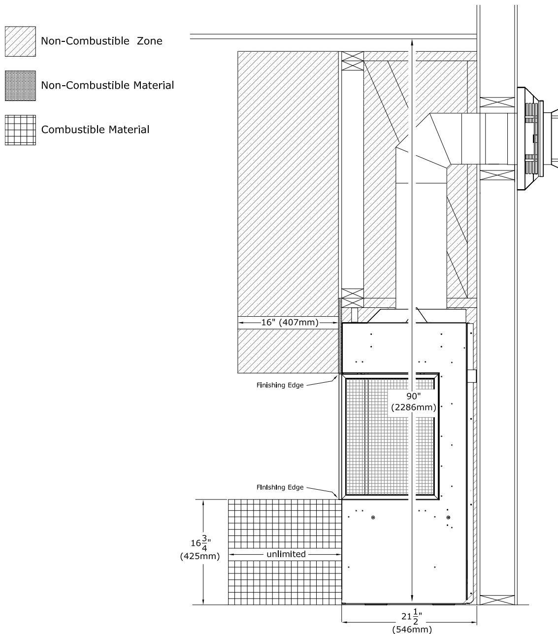
Figure 3.27 - Chamber and Hearth Projection
