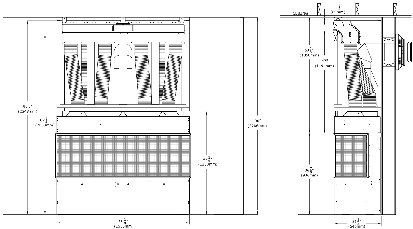
Figure 3.7 - Minimum Chamber Height Plenum Framing
