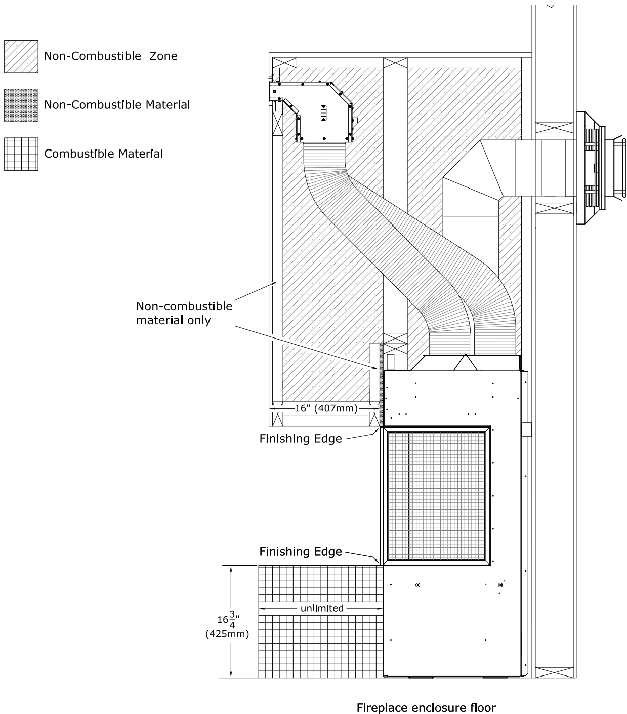
Figure 3.23 - Front Chamber Projection and Hearth Projection
