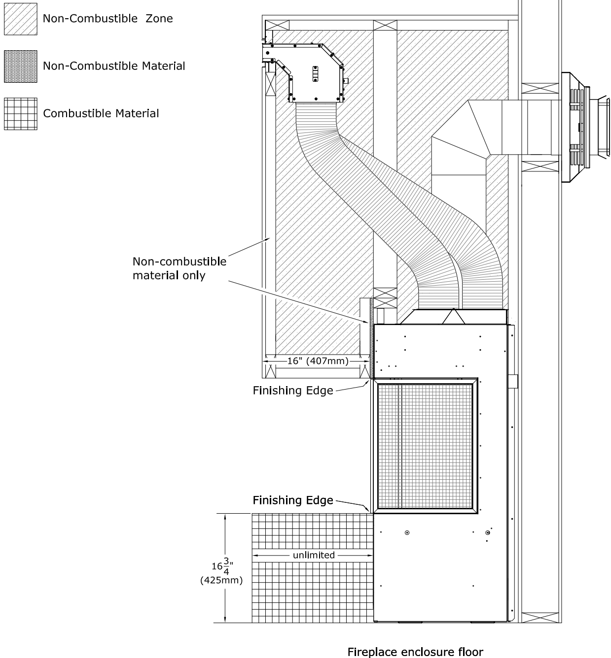
Figure 2.14 - Front Chamber Projection and Hearth Projection
