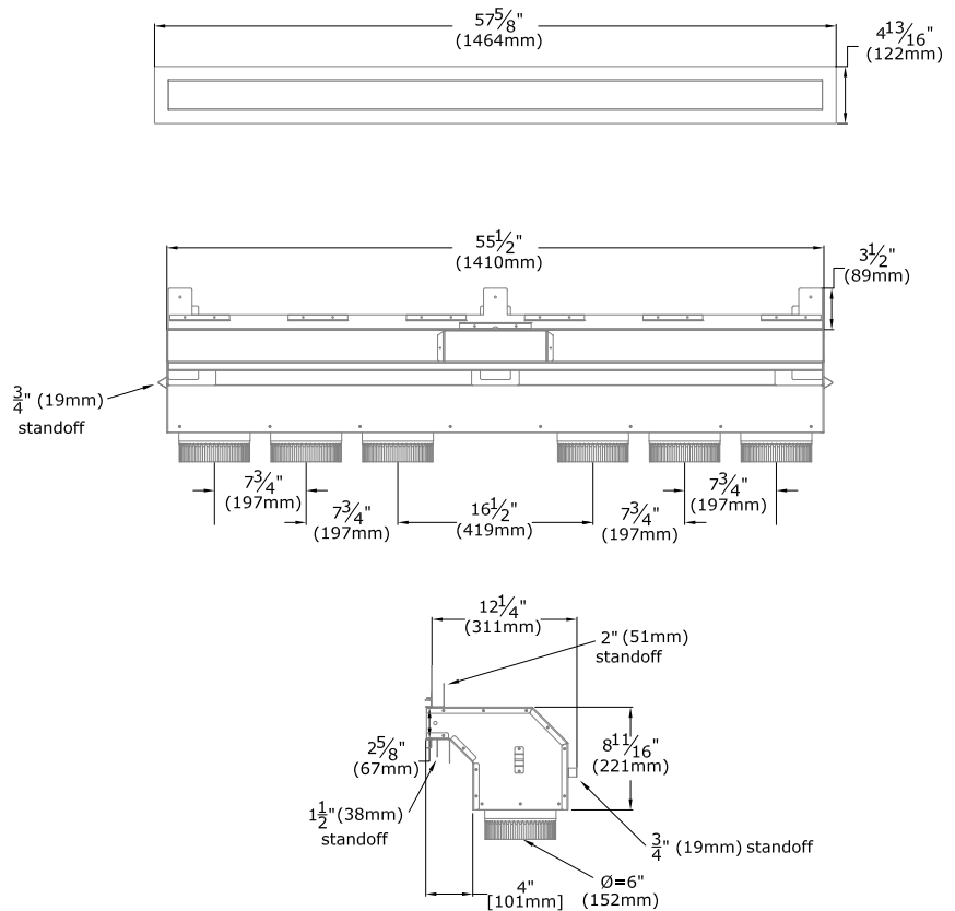
Figure 3.5 - KZK Overview
