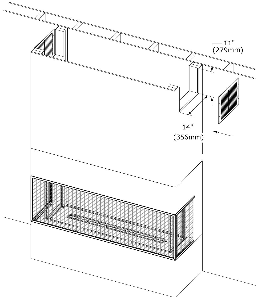
Figure 3.21 - Heat Release - Side Opening Option
