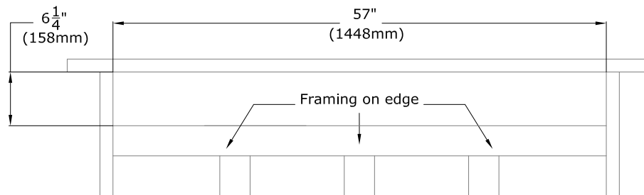
Figure 3.6 - Front KZK - Plenum Framed Opening
