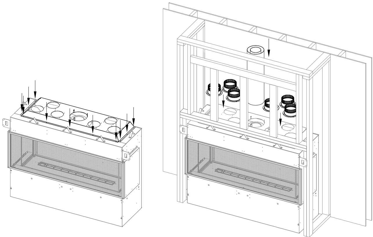
Figure 3.14 - KZK Collar Plate and Collar Installation
