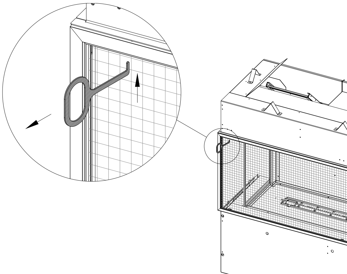
Figure 4.1 - Safety Screen Removal
