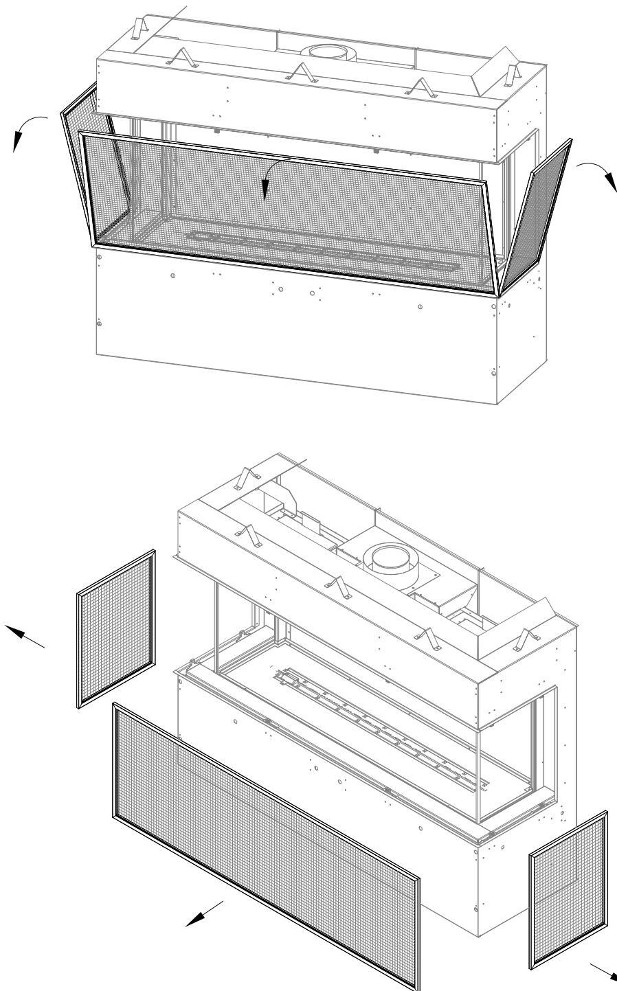
Figure 4.2 - Safety Screen Removal
