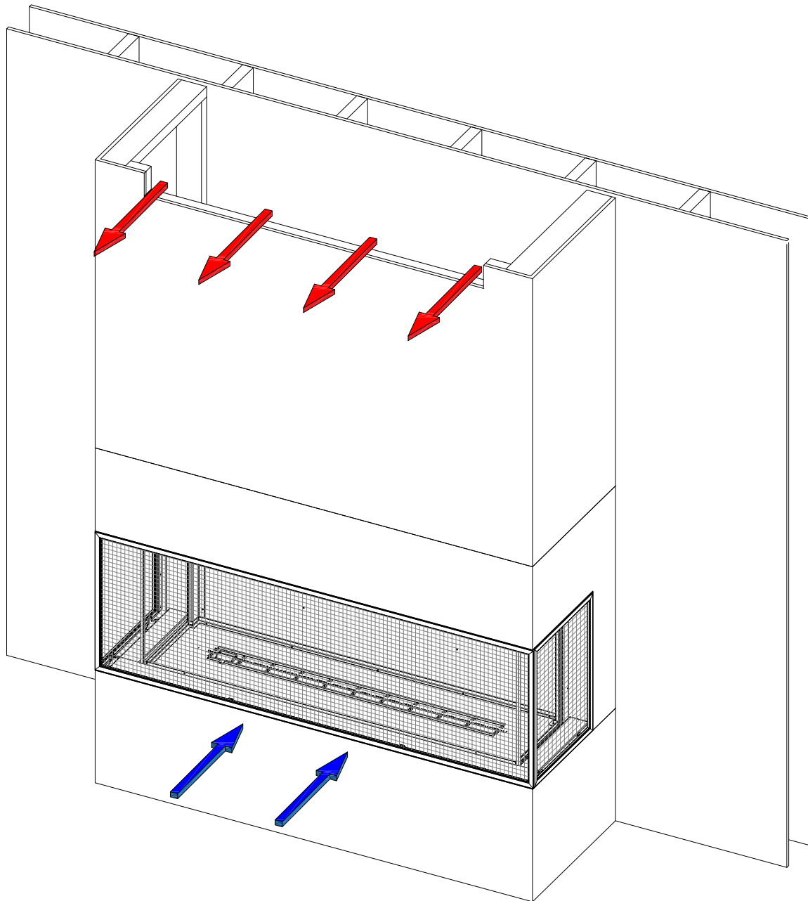
Figure 3.3 -Cooling the Fireplace Chamber and Safety Glass
