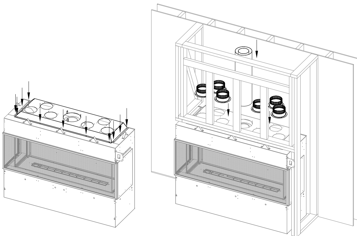
Figure 2.9 - KZK Collar Plate and Collar Installation
