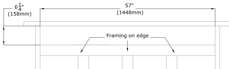
Figure 2.6 - Front KZK - Plenum Framed Opening
