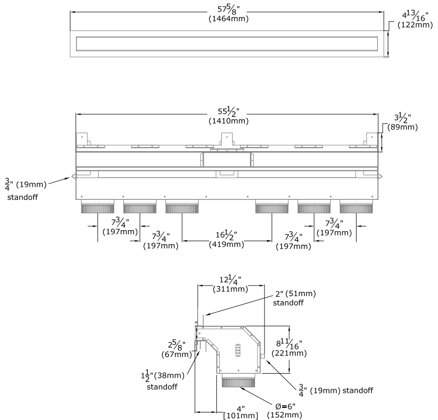
Figure 2.5 - KZK Overview
