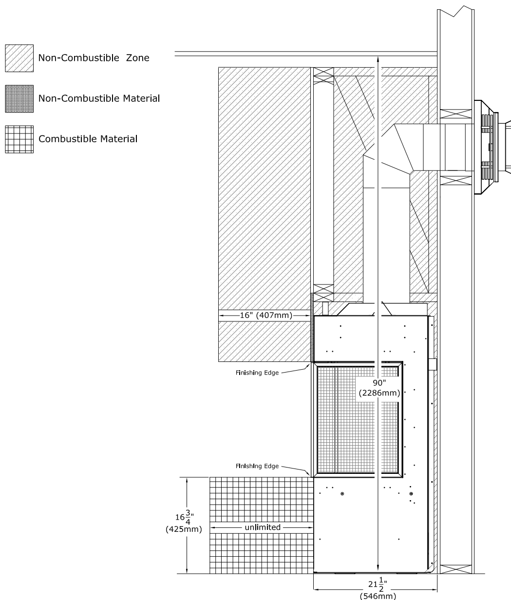
Figure 2.18 - Chamber and Hearth Projection
