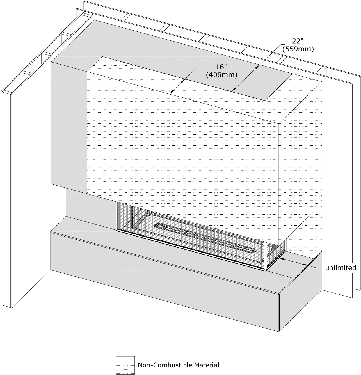
Figure 2.19 - Front and Side Projection
