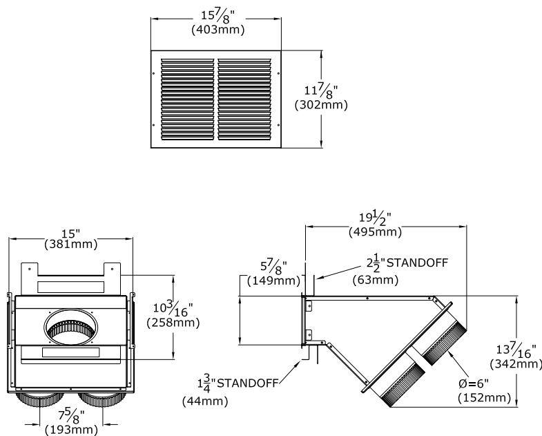
Figure 4.18 - KZK-1510 Overview
