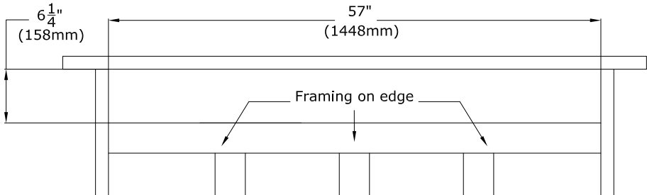
Figure 4.13 - Front KZK - Plenum Framed Opening
