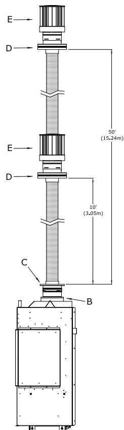
Figure 6.10 - Class A Chimney Conversion
