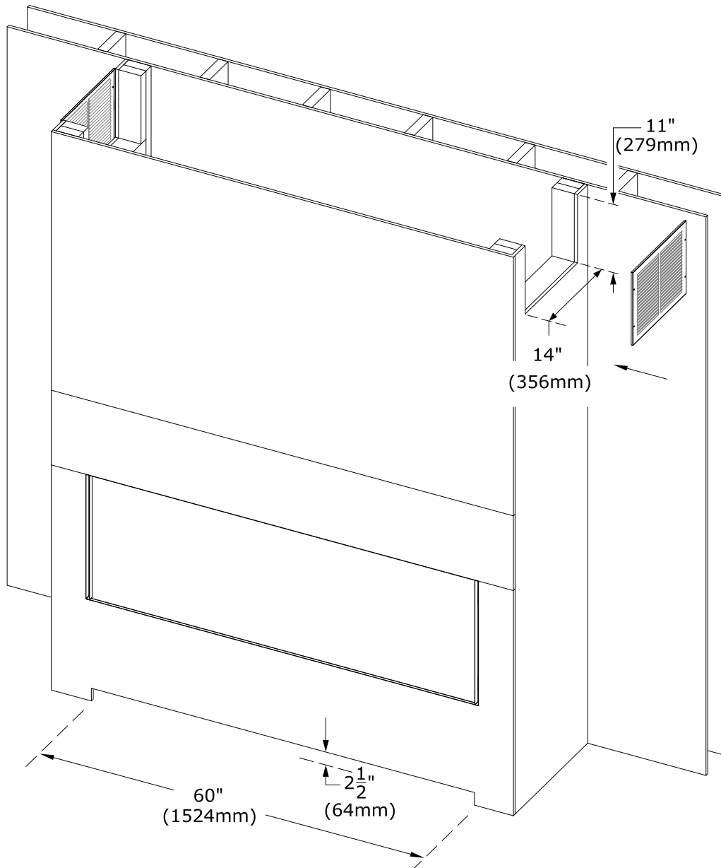
Figure 4.31 - Heat Release - Side Opening Option
