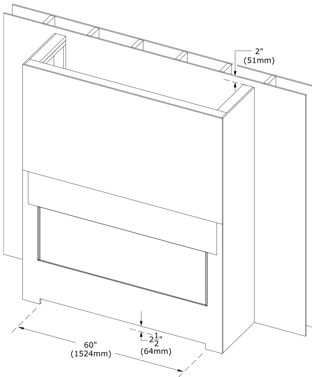
Figure 4.25 - Air Openings - Three-Sided Installation
