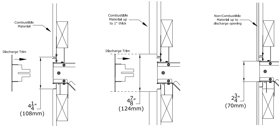
Figure 4.15 - KZK Plenum Opening - Finishing Options
