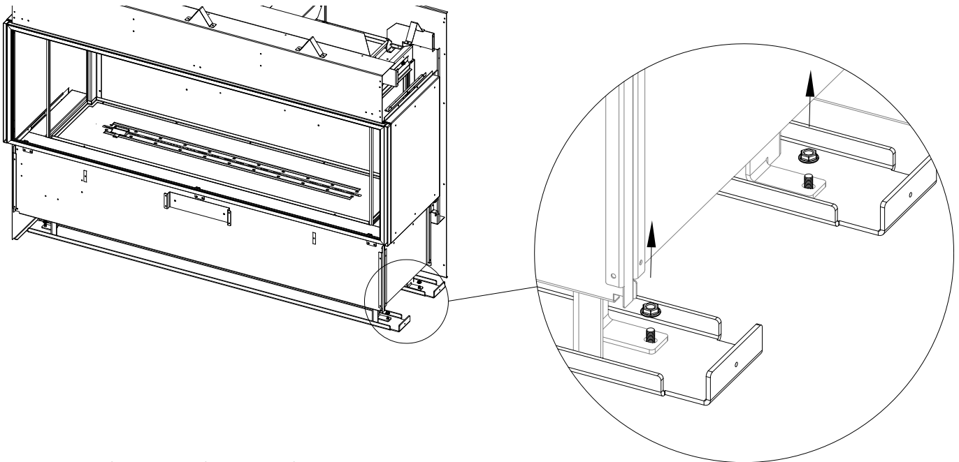
Figure 1.2 - Shipping Bracket Removal
