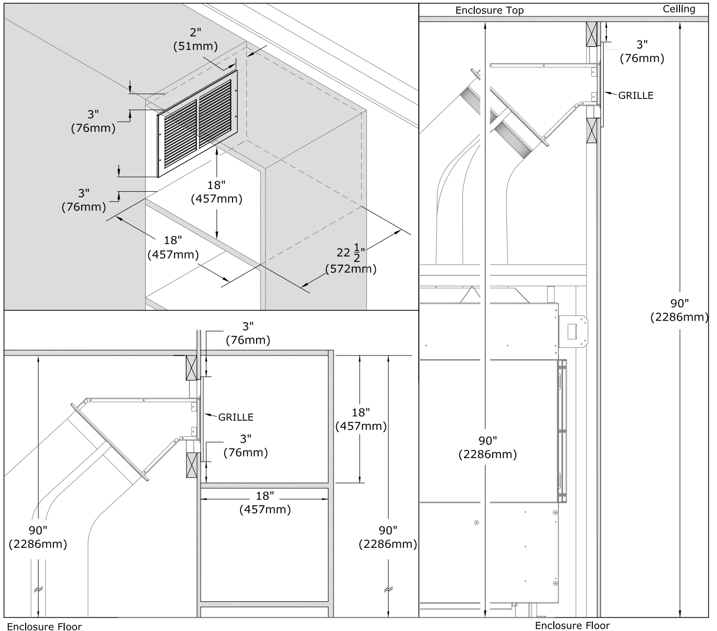
Figure 4.42 - Clearance to Sidewall
