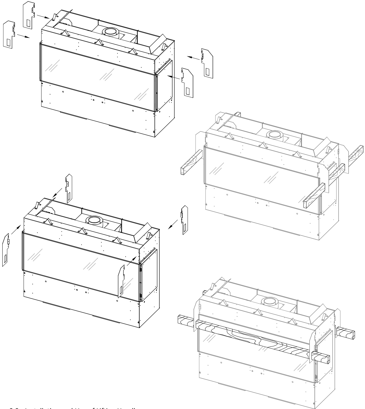
Figure 3.2 - Installation and Use of Lifting Handles
