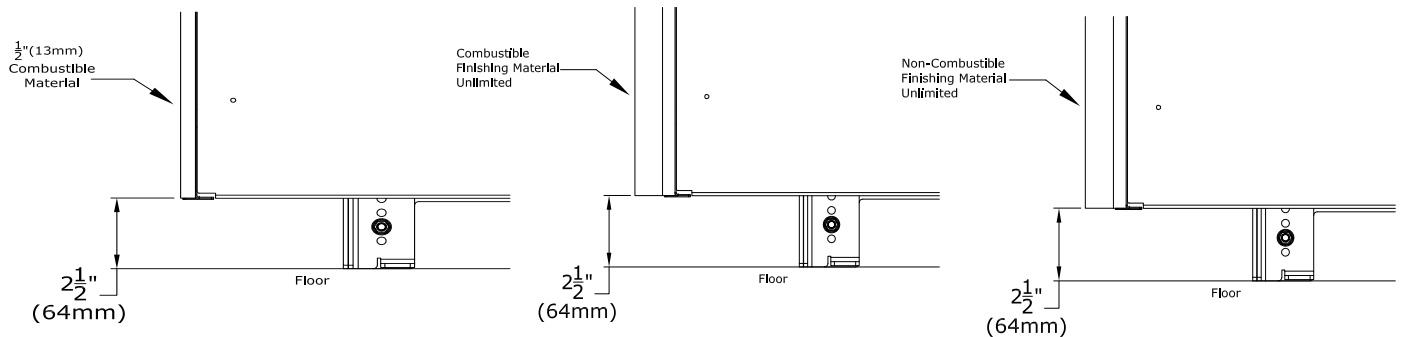
Figure 4.16 - KZK Air Intake Opening - Finishing Options
