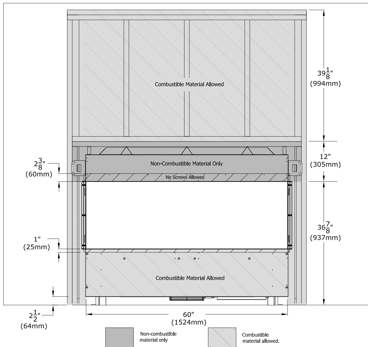
Figure 4.8 - Facing Material Requirements
