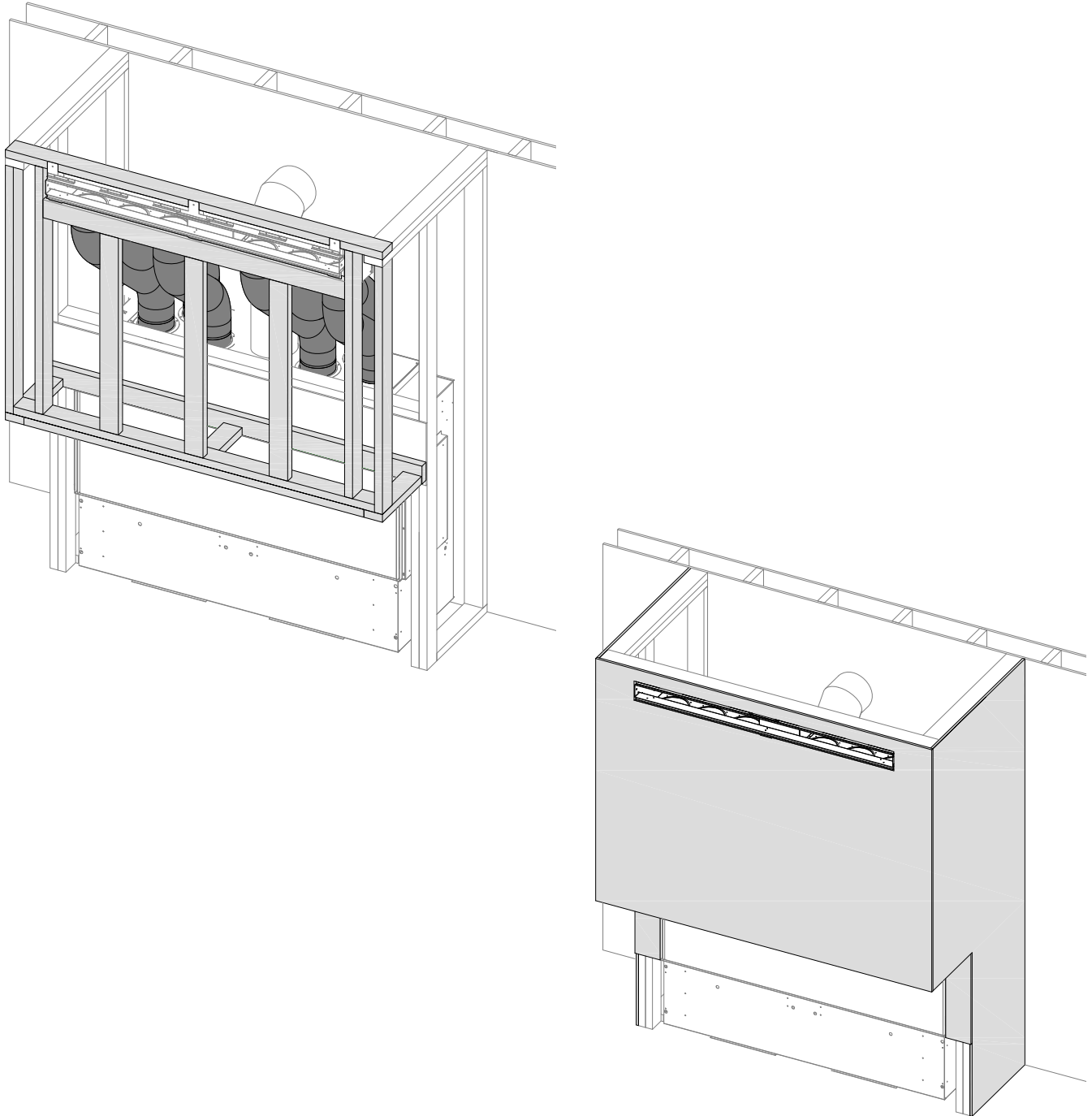
Figure 4.35 - Constructing KZK Projection
