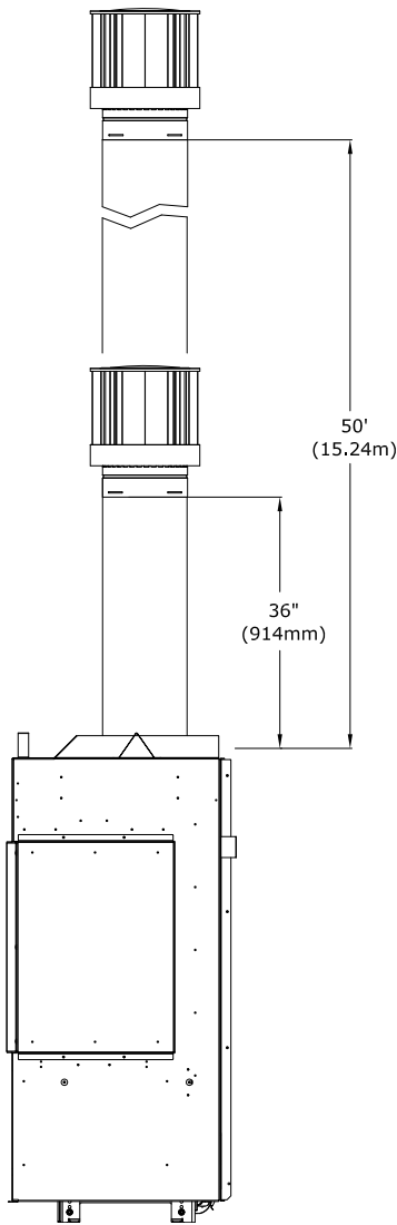
Figure 6.5 - 5"x8" Vertical
