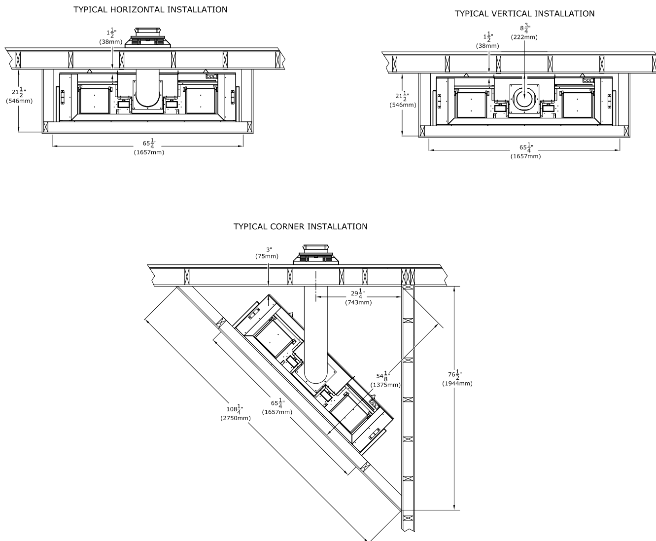
Figure 3.1 - Typical Installation
