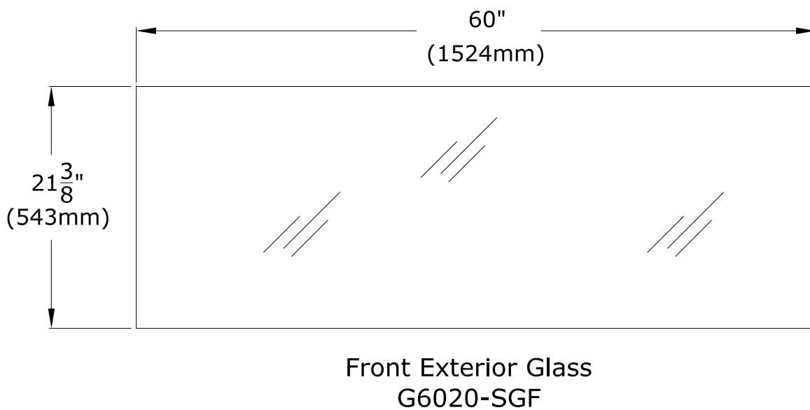
Figure 2.2 - Glass Safety Barrier Dimensions
