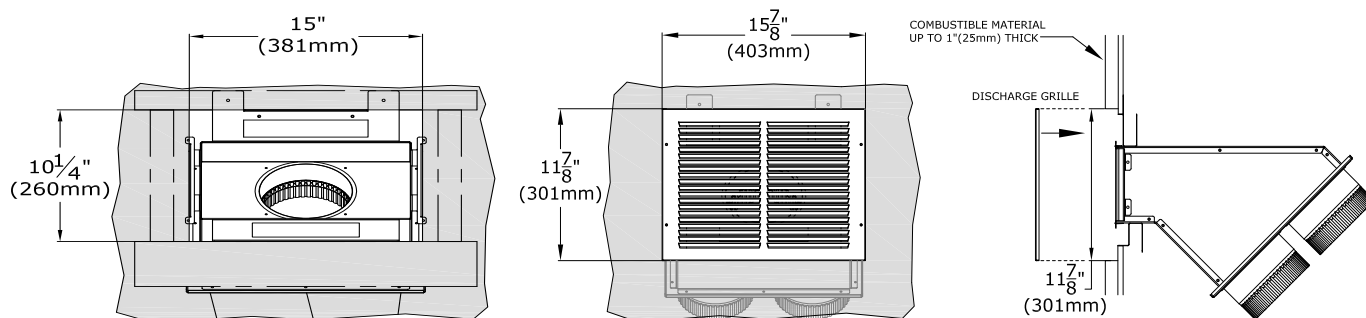
Figure 4.22 - KZK Grille - Finishing Options
