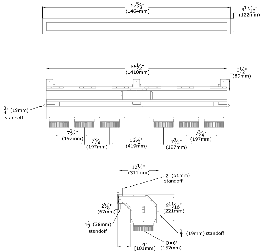
Figure 4.12 - KZK Overview
