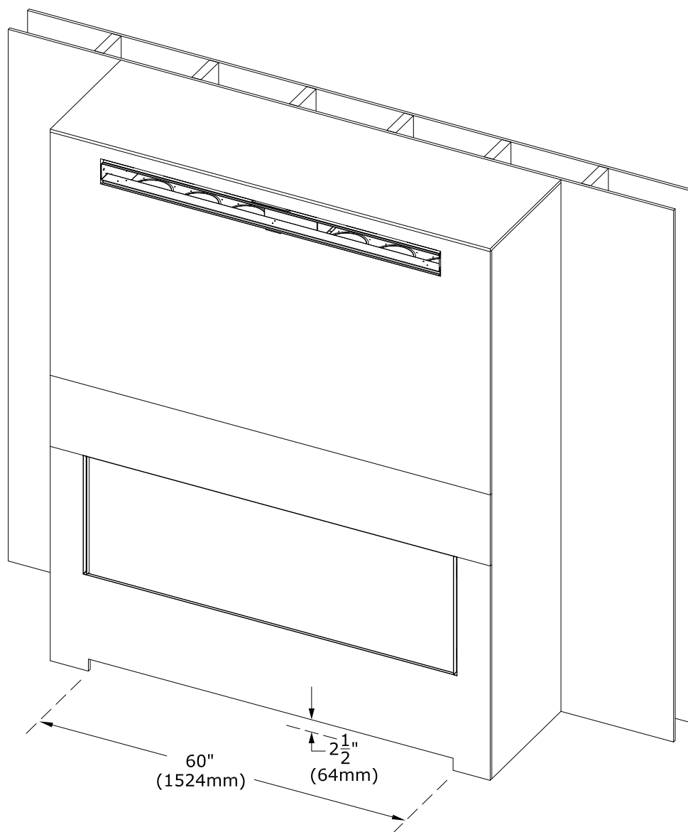
Figure 4.15 - Minimum Air Intake Opening
