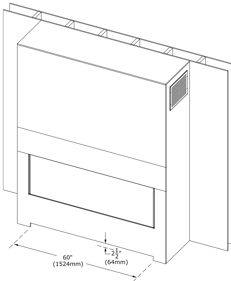
Figure 4.21 -Minimum Air Intake Opening
