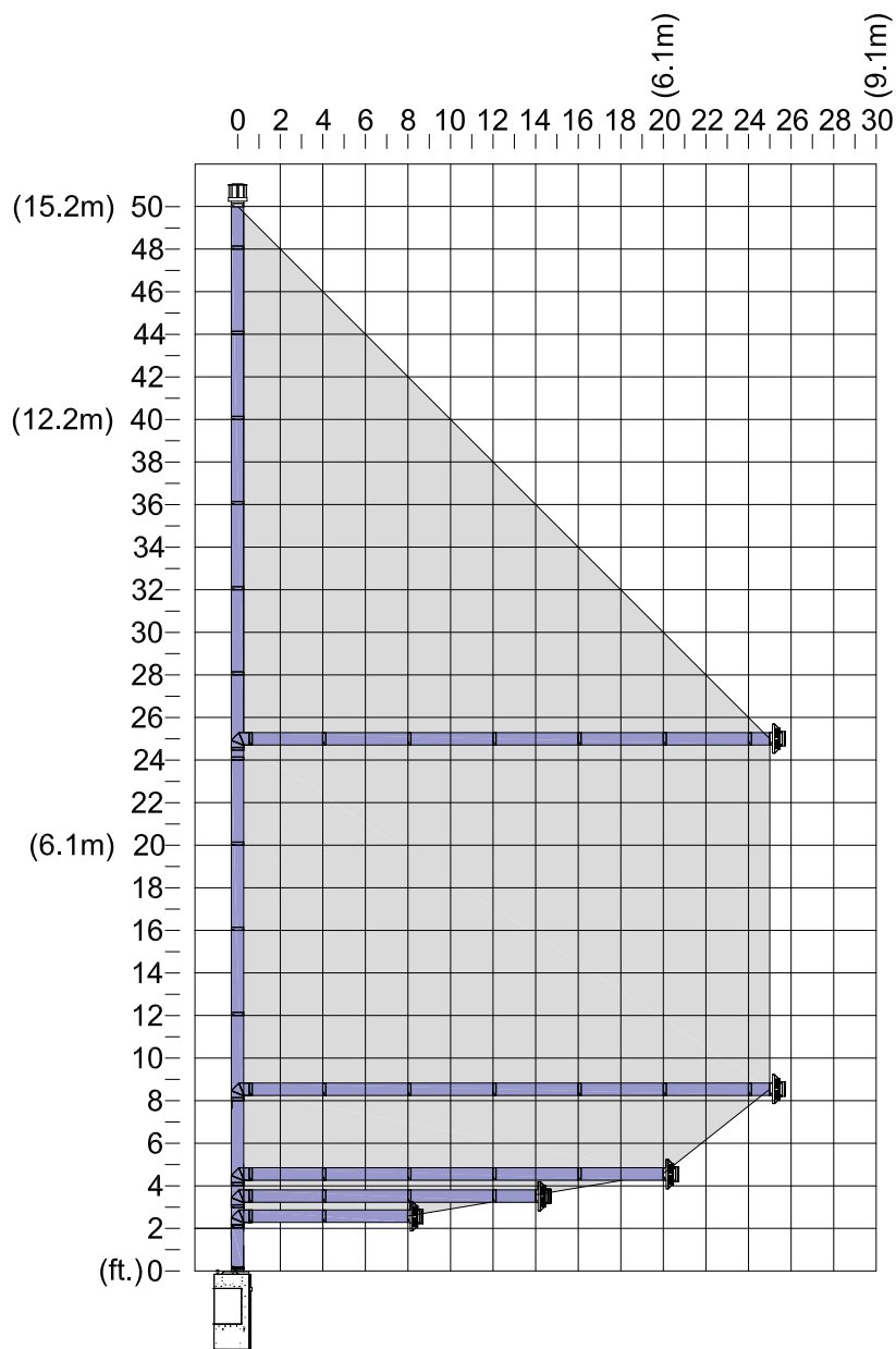
Figure 6.9 - Combination Venting
