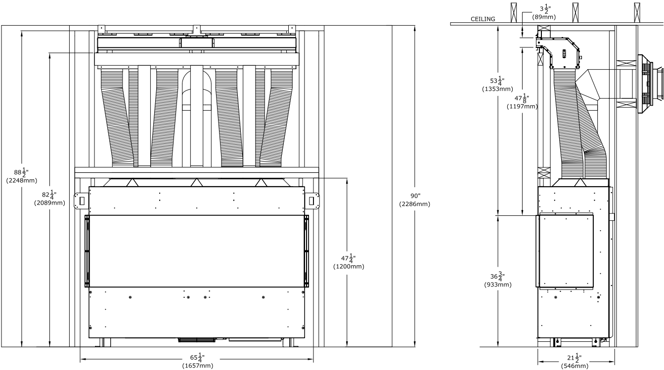
Figure 4.14 - Minimum Chamber Height Plenum Framing
