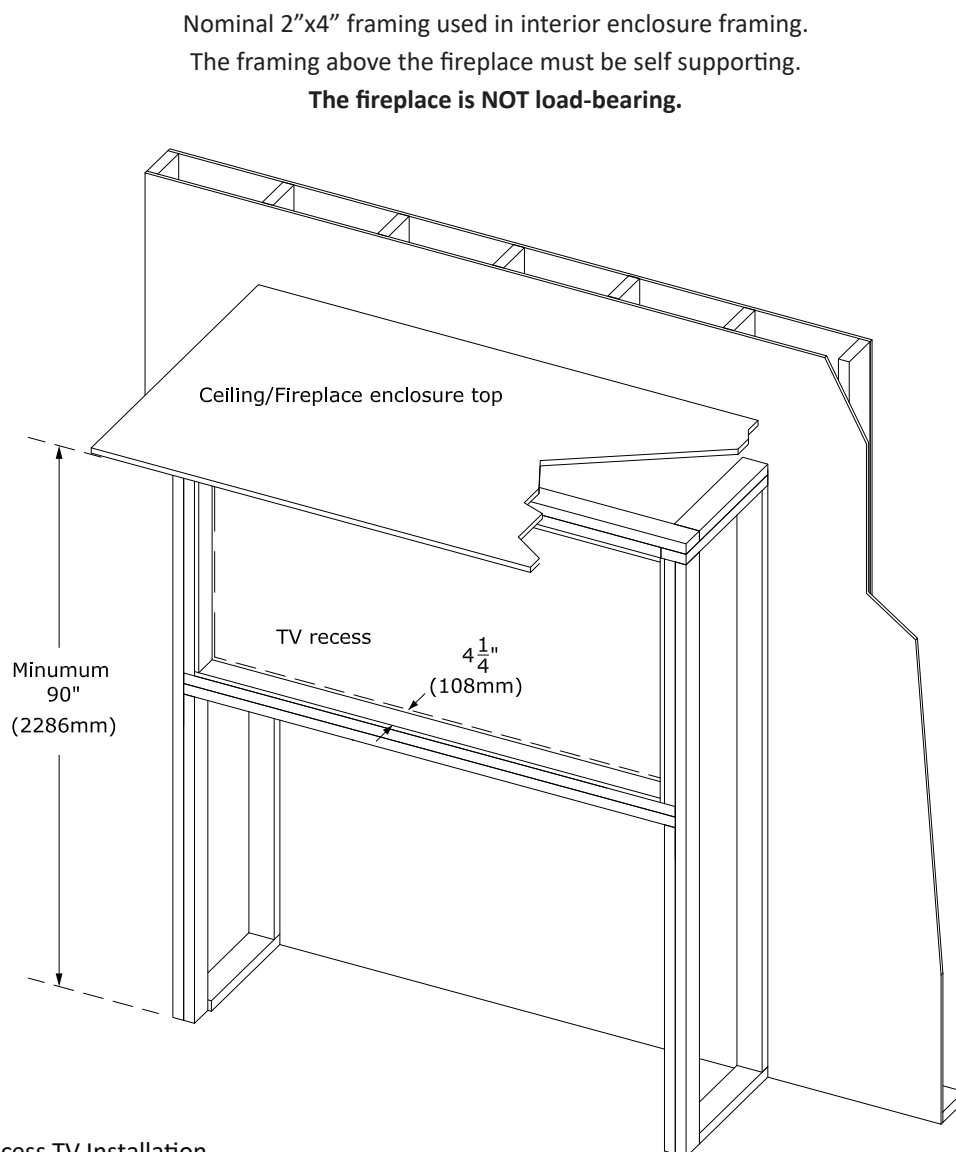
Figure 4.2 - Recess TV Installation
