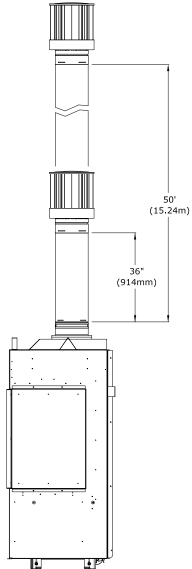
Figure 6.6 - 4"x6-5/8" Vertical
