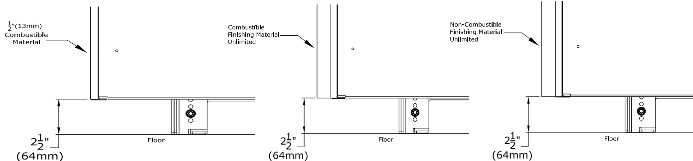
Figure 4.23 - KZK Air Intake Opening - Finishing Options
