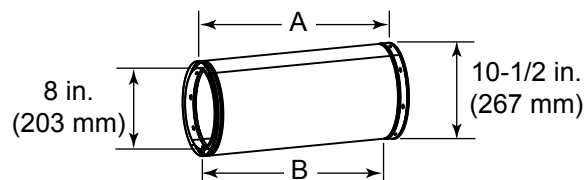
Chimney Sections
