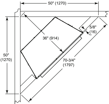
BASIC CORNER INSTALLATION
