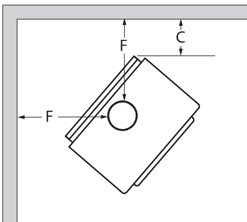
Figure 11: Clearances - Corner
