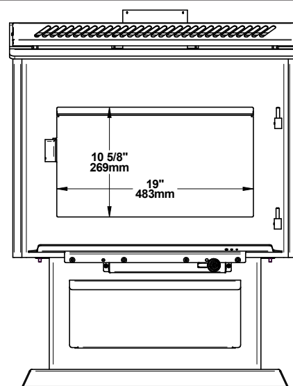
Figure 6: Door opening
