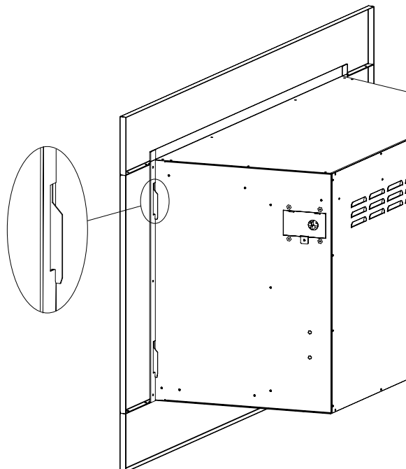
Figure 13: Surround Panel Hooks Installed
