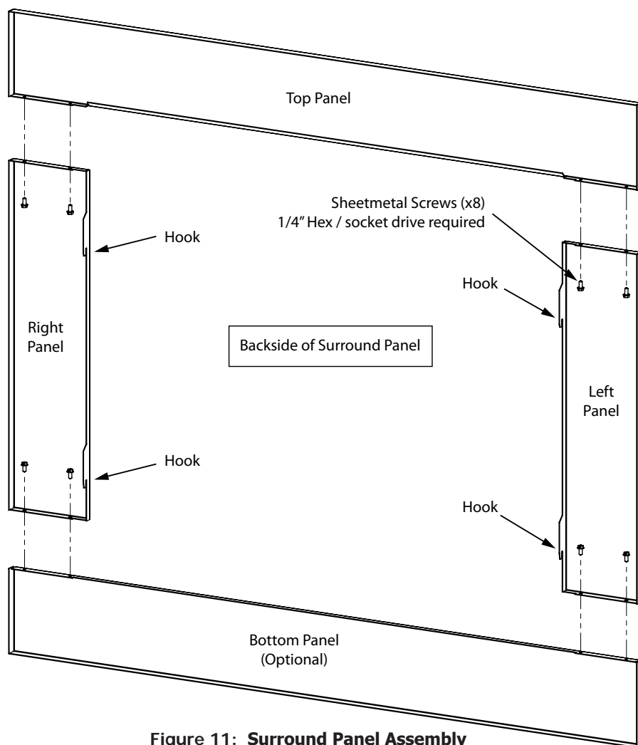
Figure 11: Surround Panel Assembly
