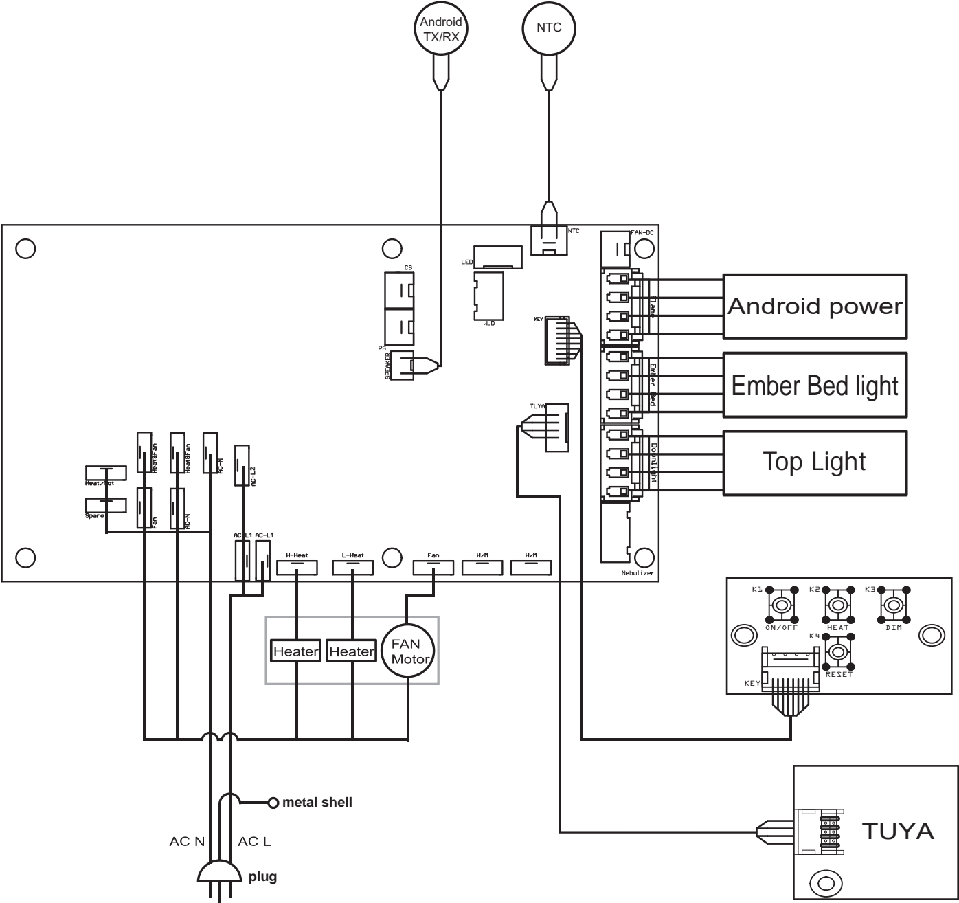
Figure 31: Wiring Diagram
