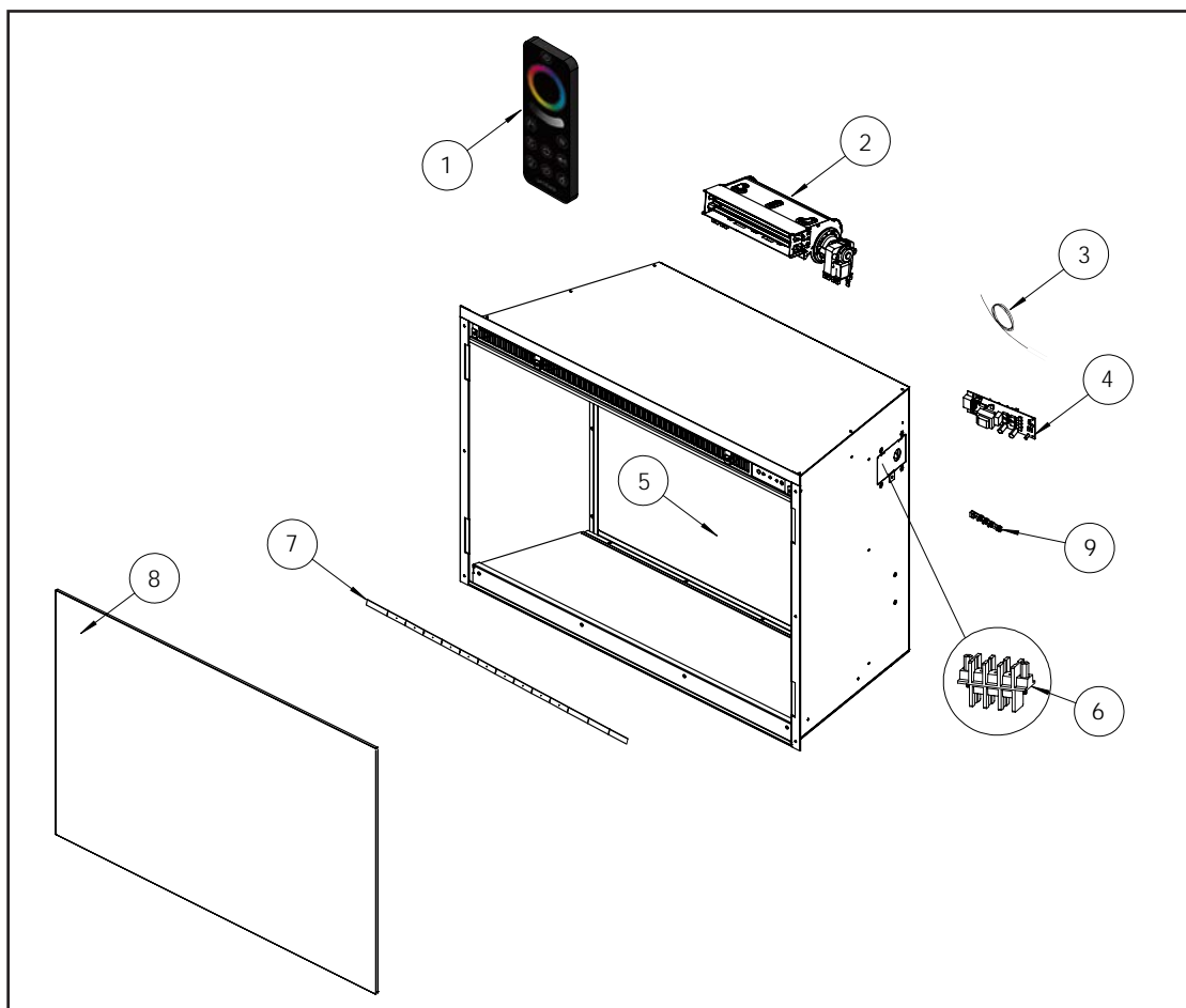
Figure 32: Parts Diagram
