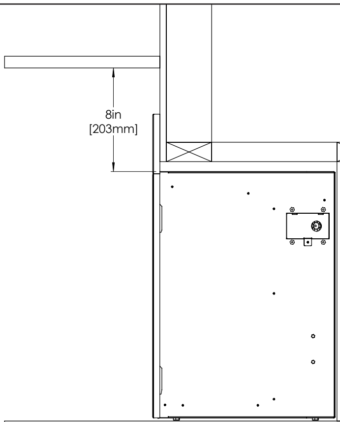
Figure 7: Mantle Clearance
