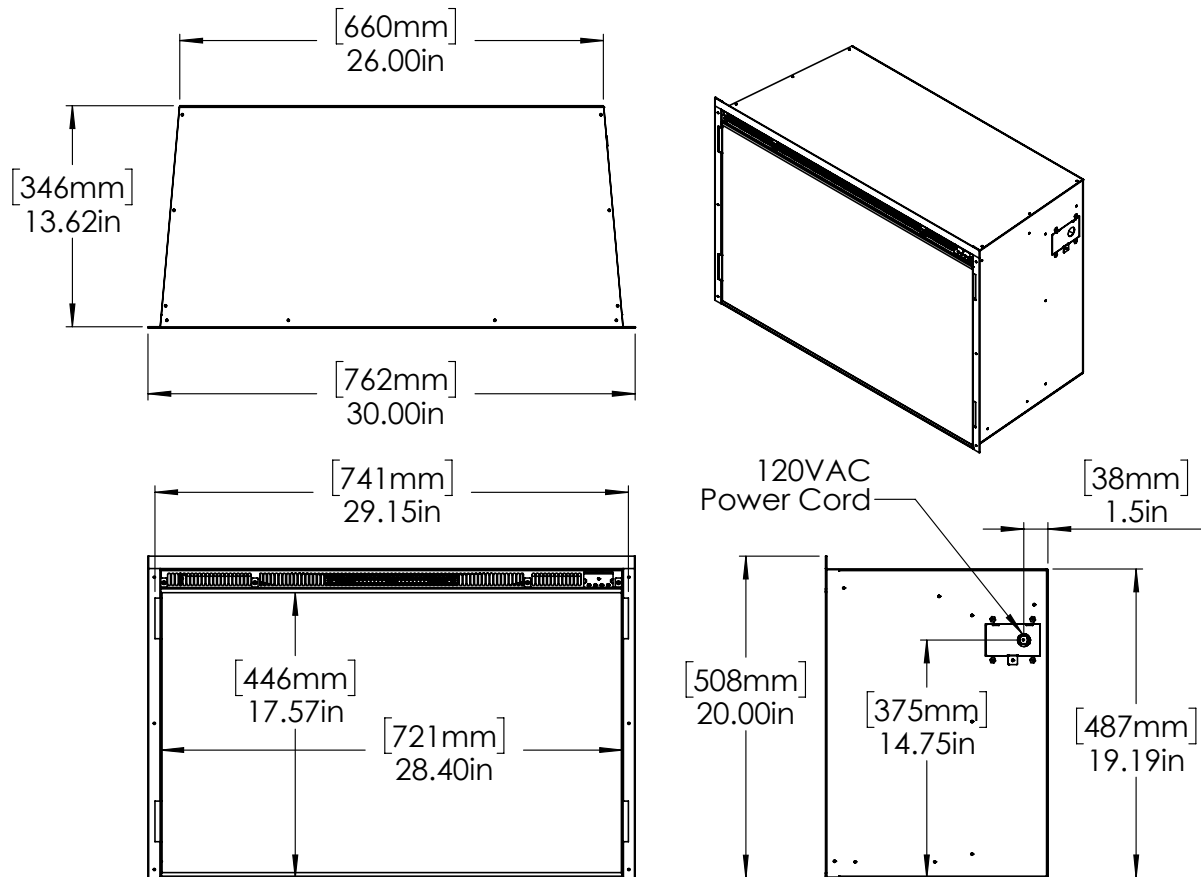
Figure 1: Fireplace Dimensions
