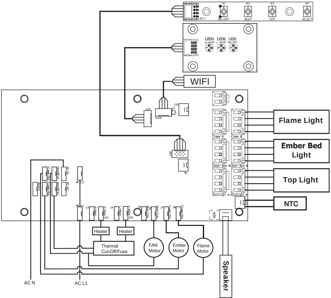
Figure 30: Wiring Diagram
