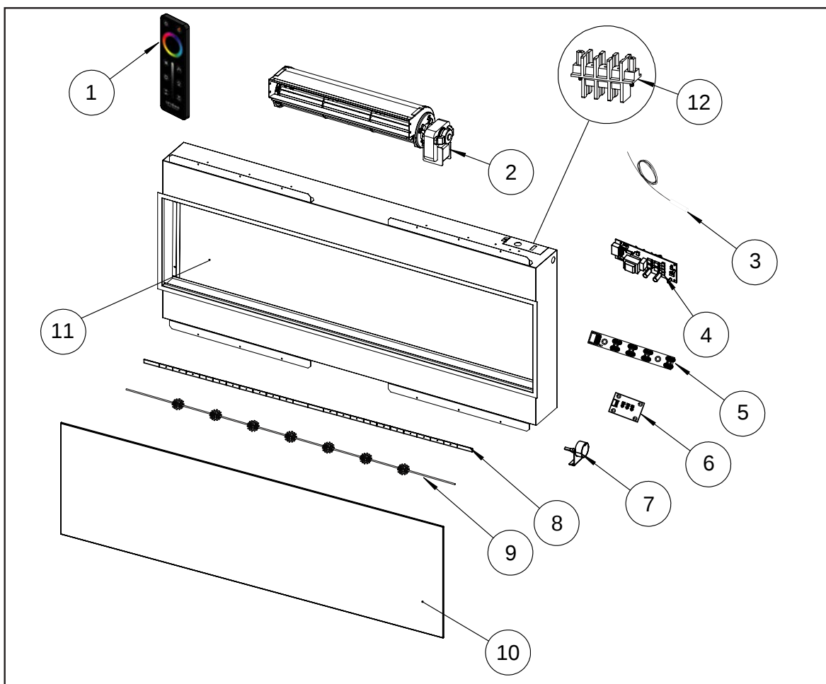
Figure 31: Parts Diagram
