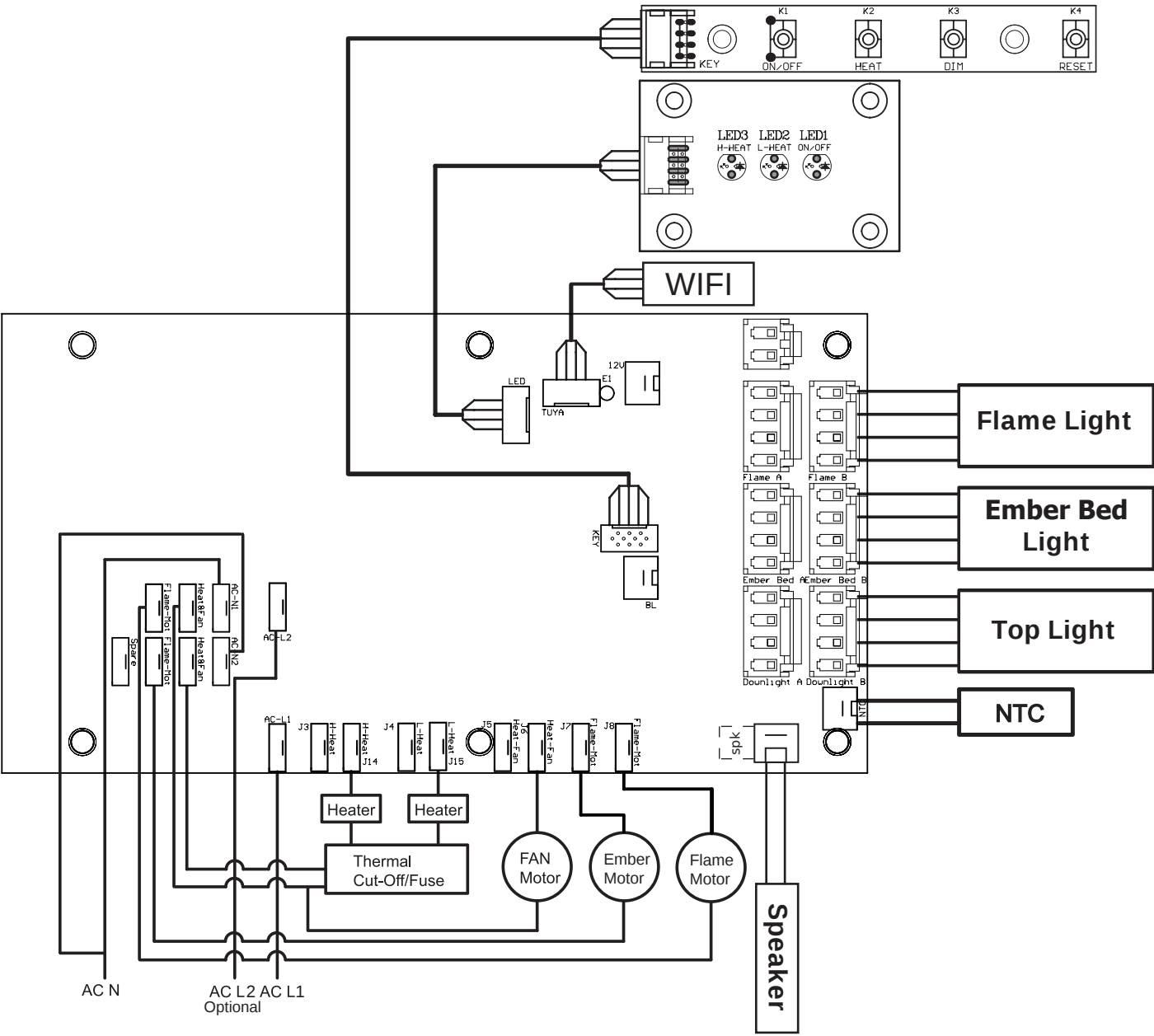
Figure 43: Wiring Diagram
