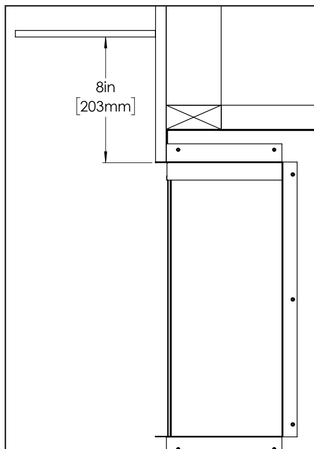
Figure 18: Mantel Clearance
