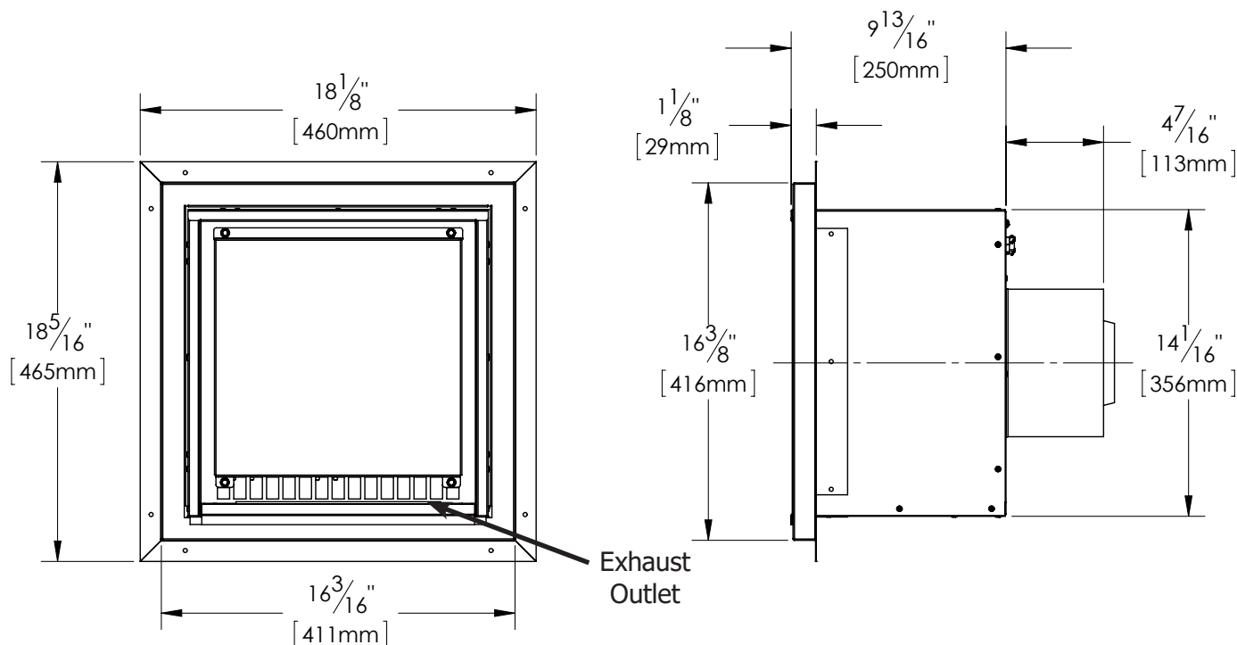
Figure 1: Power Vent Dimensions
