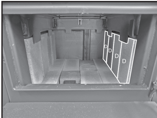
Figure 17: Bricks on right side wall in place.
