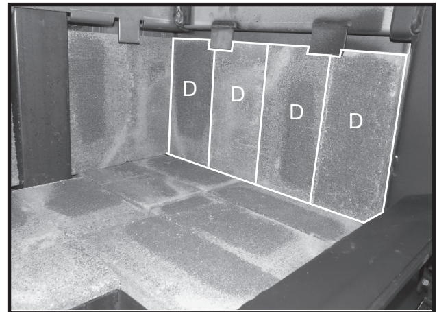
Figure 18: Side wall brick placement.
