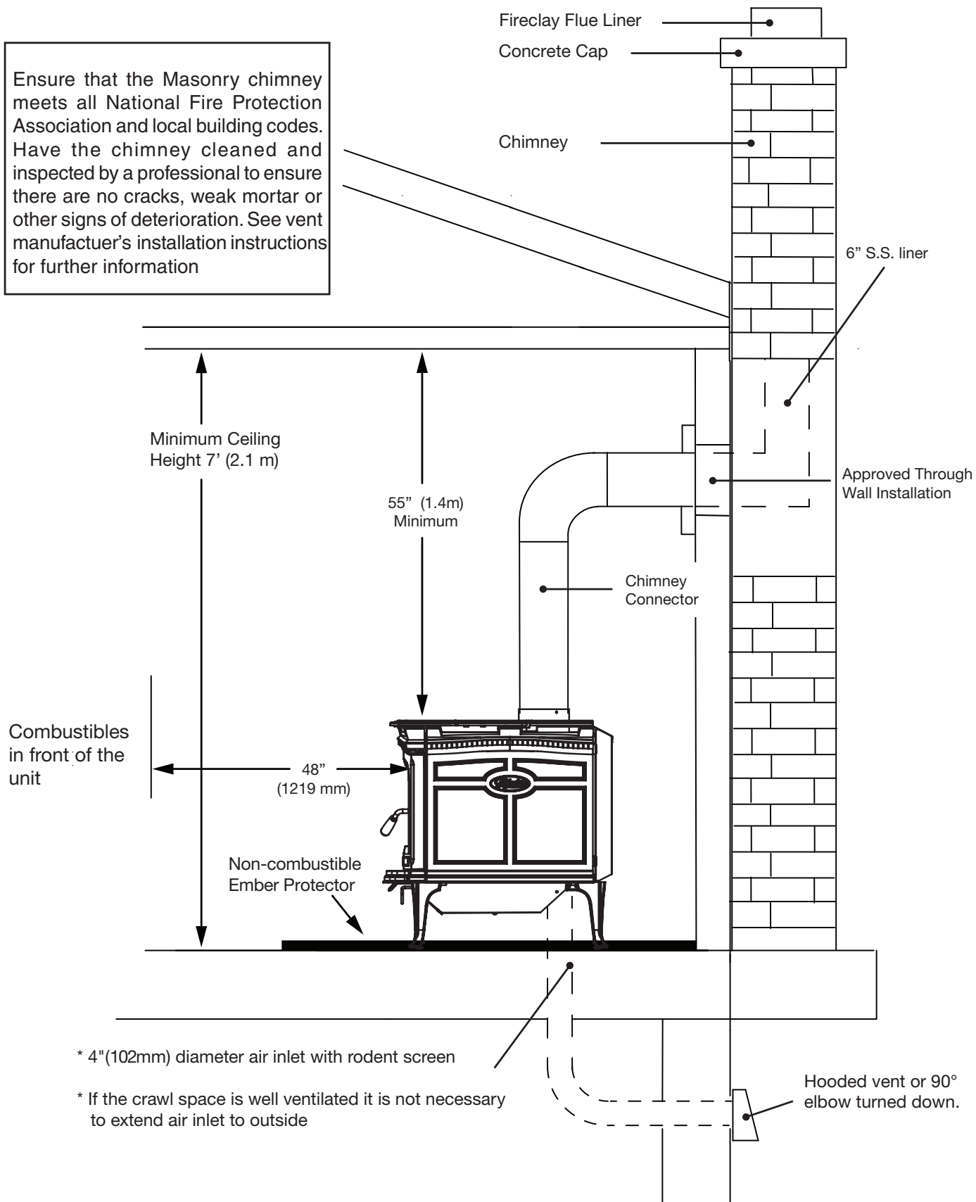
Figure 7: T6 Venting to a masonry chimney.
