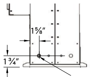
Figure 9.b gas line access
