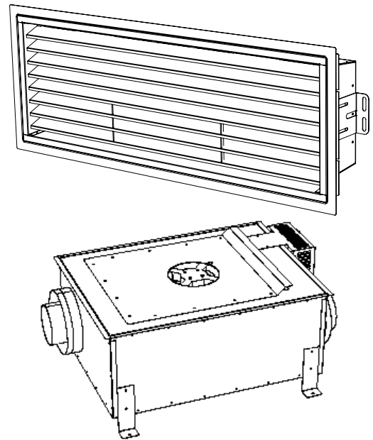
Figure 15.d PVHIN58-300 Inline power vent with TMHIN58-40 Termination (with vanity ring)
