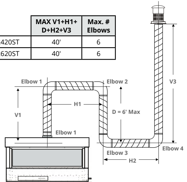
Figure 6.c Multi-Elbow with downward vent run, Top or Rear Vent, Roof mounted power vent.
