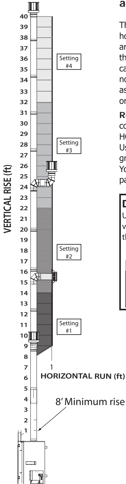
Figure 63: 5" x 8" LP Vent Graph
