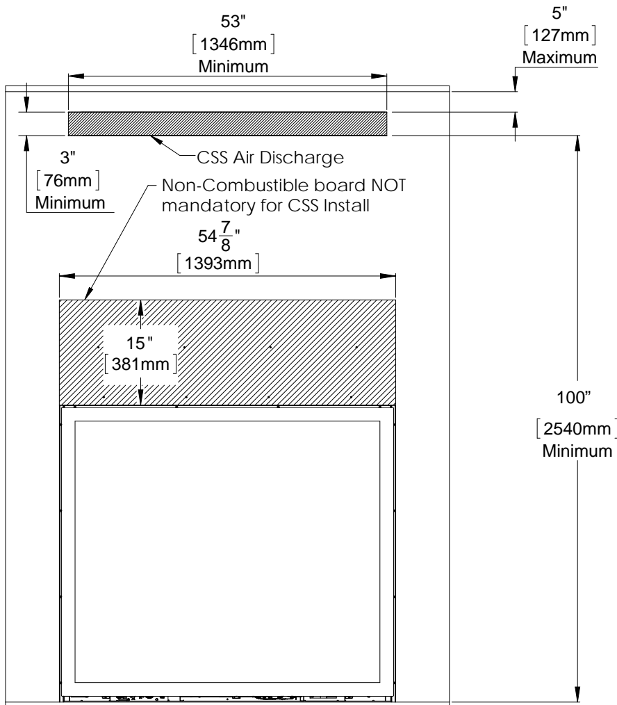
Figure 41: Framing Option 1
