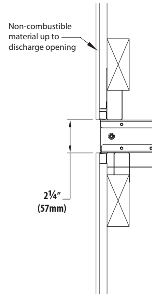
Figure 3.7, Non-combustible Material Trim Finish
