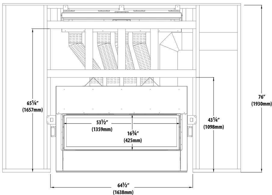
Figure 2.9, #KZK-054 and CLW-ST Framed Opening and Clearances
