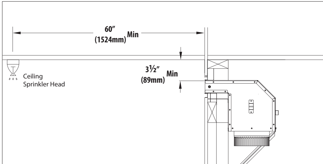
Figure 2.1, KZK Clearance to Sprinkler
