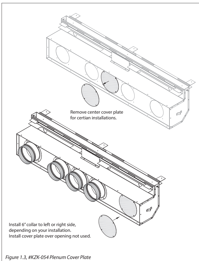
Figure 1.3, #KZK-054 Plenum Cover Plate
