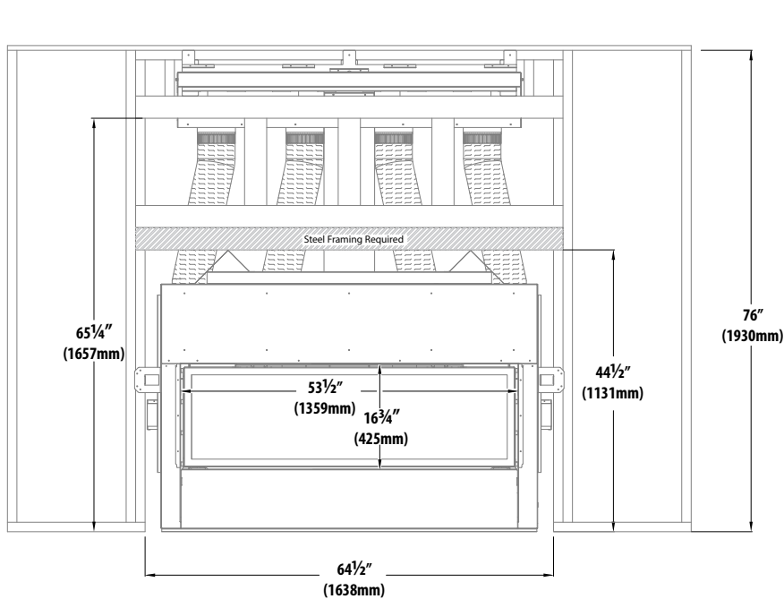
Figure 2.8, #KZK-054 and CLW-50 Framed Opening and Clearances
