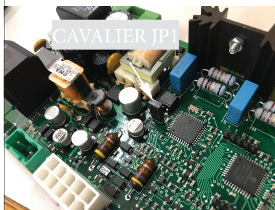
Figure 4.2, Cavalier JP1
