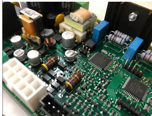
Figure 4.3, Plastic Jumper Removed
