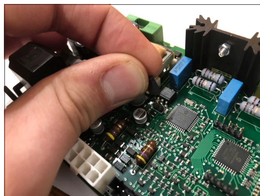
Figure 4.2, JP1 Jumper
