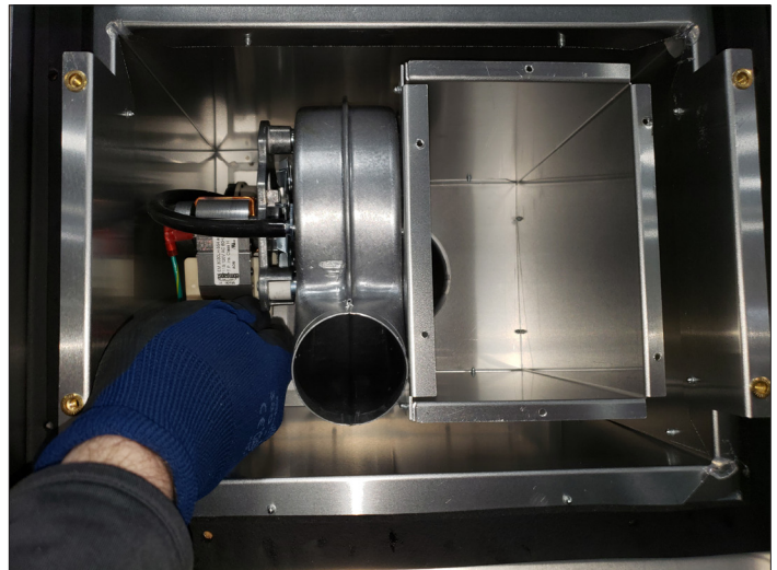
Figure 5.4, Remove Hot, Neutral and Ground wire
