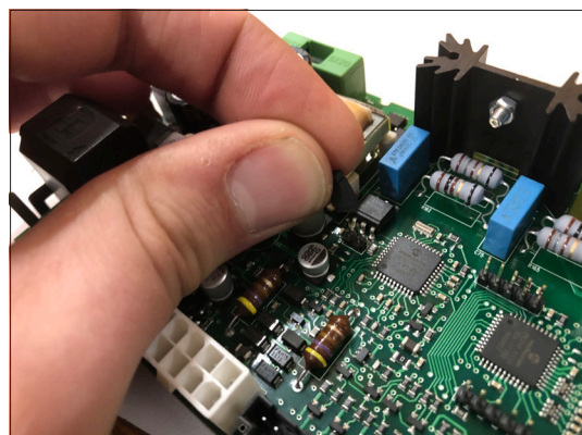
Figure 4.2, Cavalier JP1
