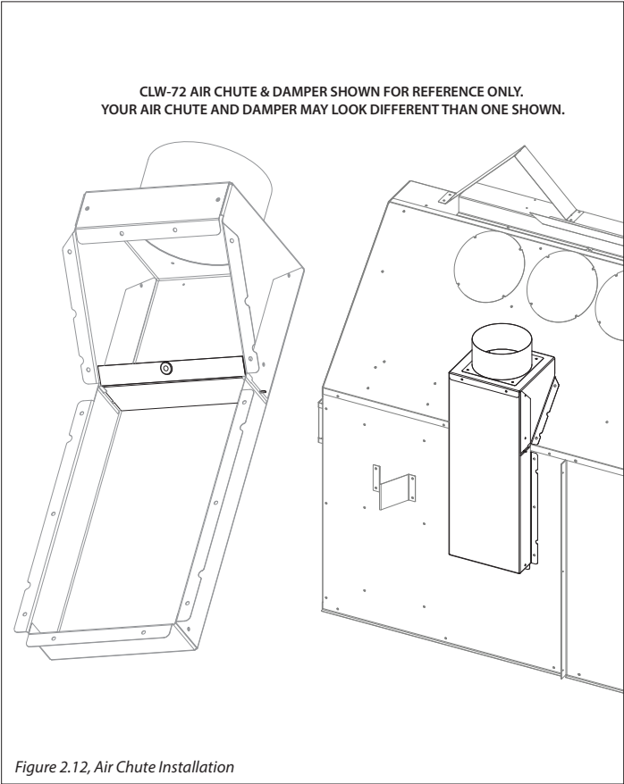
Figure 2.12, Air Chute Installation
