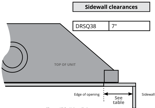
Figure 17.b Sidewall clearances
