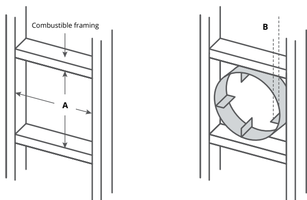
Figure 15.a Heat Shield Installation. (Install by sliding over vent pipe where it passes through the combustable construction).
