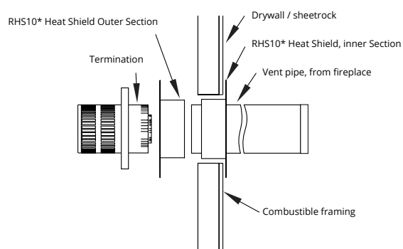
Figure 11.b RHS10* Installation. (Install by sliding Outer Section over vent pipe where it passes through the combustable construction).
