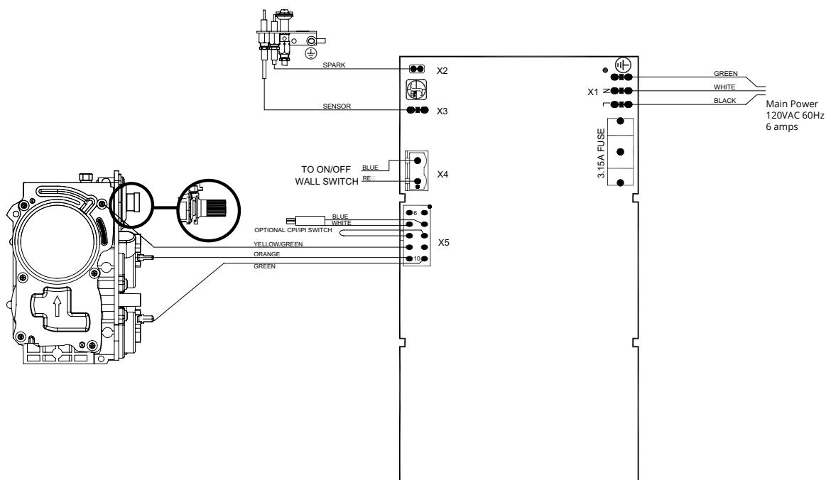
Figure 15. Wiring diagram for DRSQ38*I with SIT Proflame Electronic Ignition
