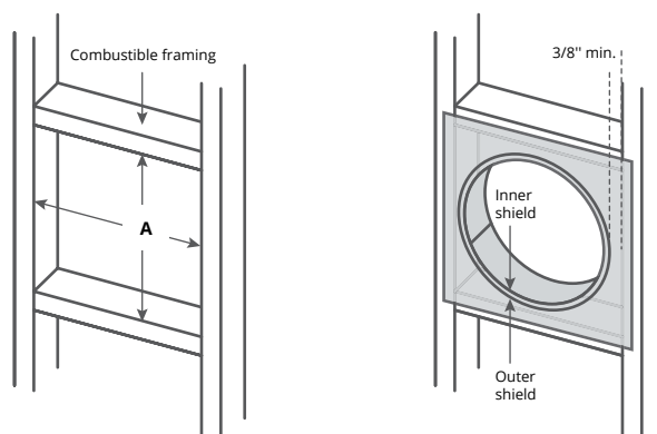
Figure 11. RHS10* Installation. (Install by sliding over vent pipe where it passes through the combustable construction).
