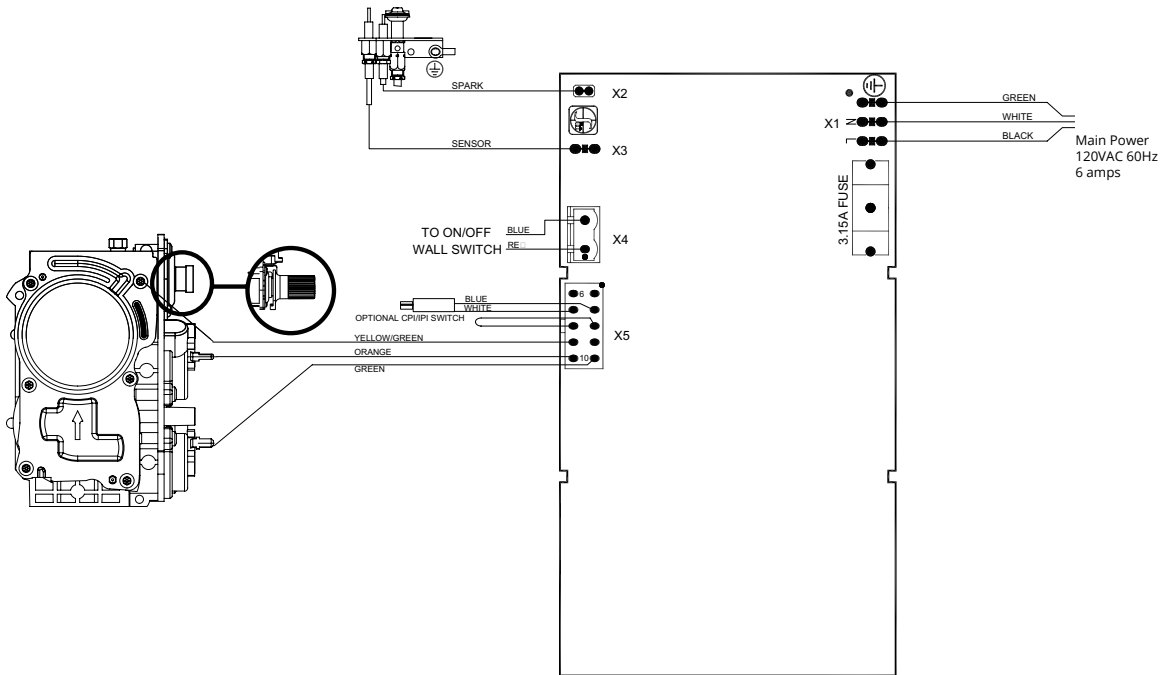
Figure 15. Wiring diagram for DRSQ38* 1 with SIT Profame Electronic Ignition
