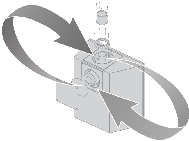
Figure 7. Flue cover and collar removal and install, Top Vented fireplace.
