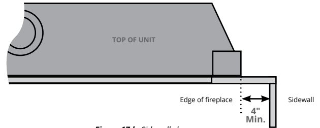
Figure 17.b Sidewall clearances
