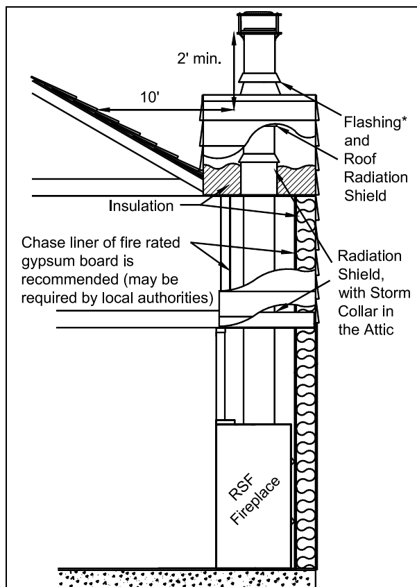
Figure 15 Chimney Installed with a Chase Enclosure Example
