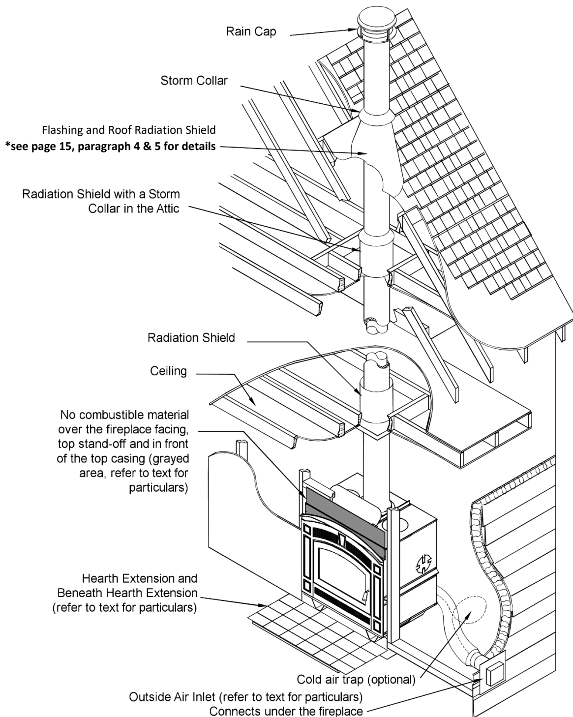
Figure 3 PEARL 3600 General Installation
