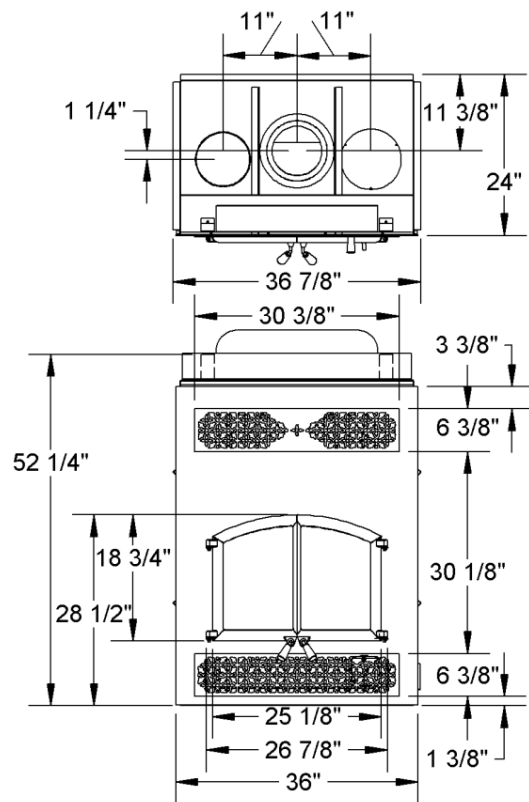
OPEL2 with Decorative Grills
