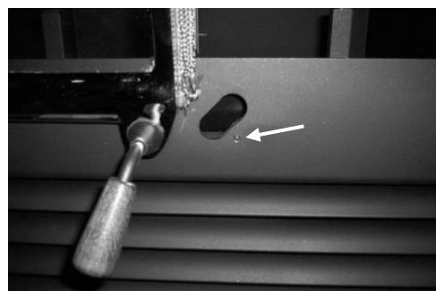
Figure 3 Door Latch Adjustment
