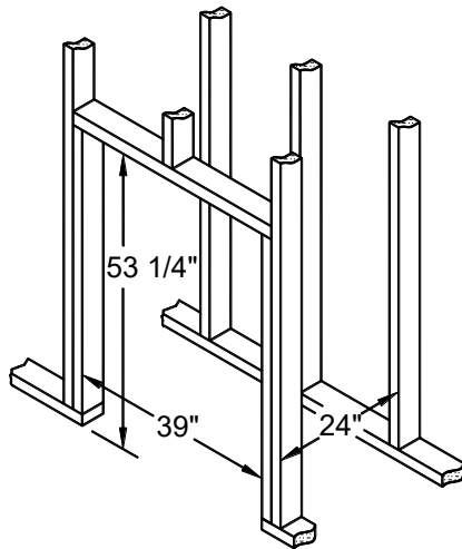
Figure 6 Louvered OPEL+ KEYSTONE Framing Examples
