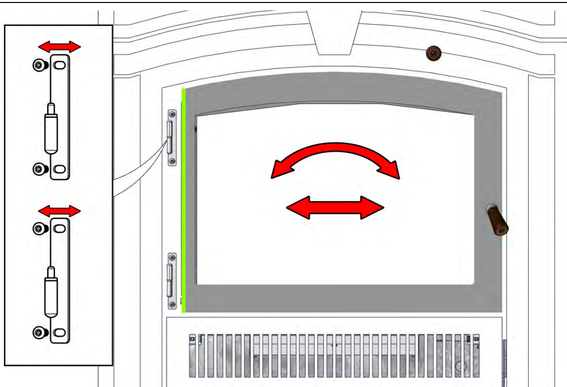
Figure 5 Door Adjustment
