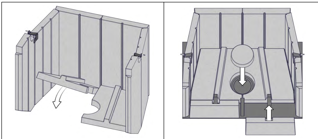
Figure 18 Refractory Brick Installation
