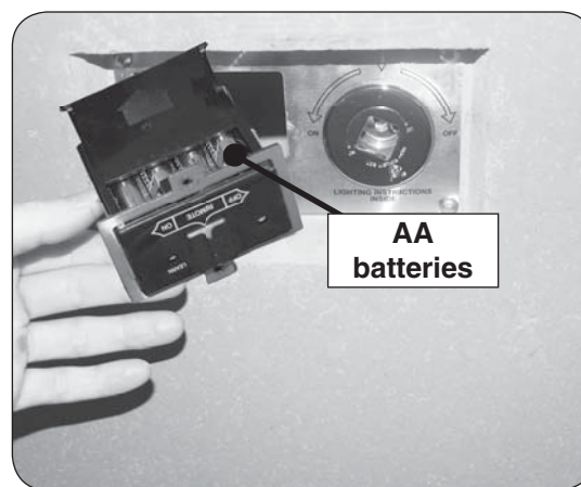
Fig. 45-3 Remote receiver batteries
