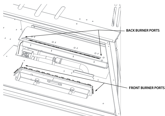
Figure 14.1, Burner System
