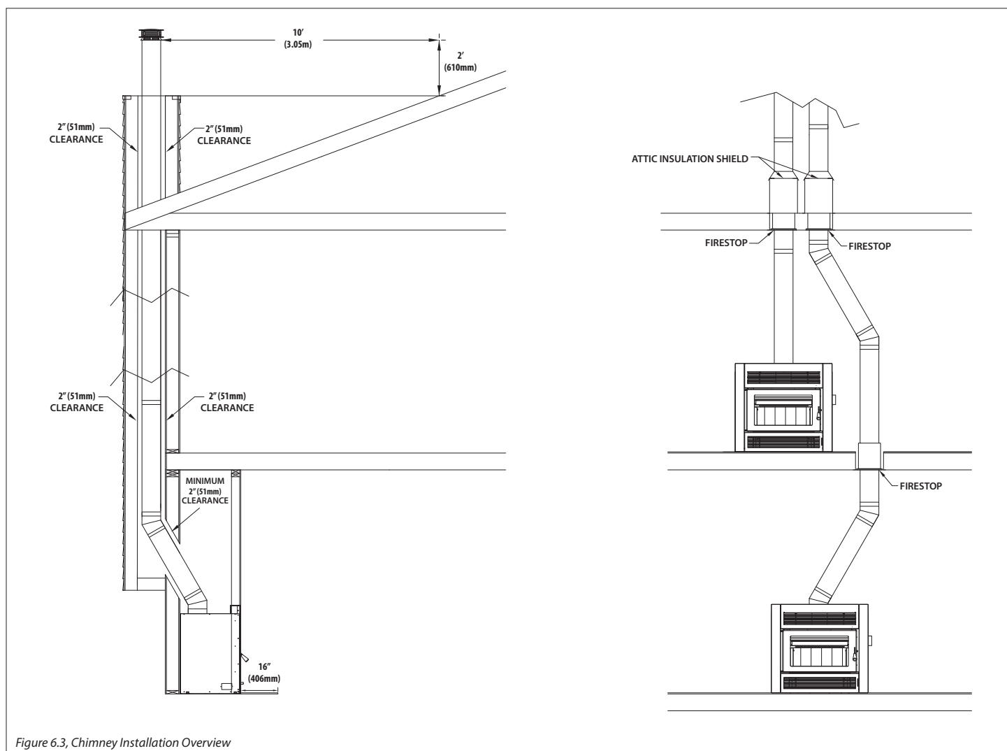
Figure 6.3, Chimney Installation Overview
