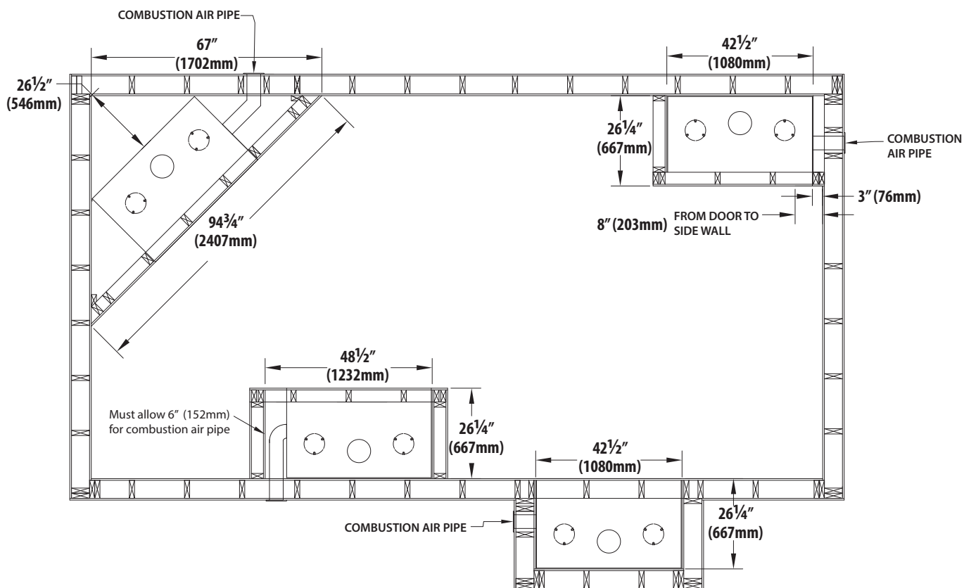
Figure 3.2, Typical Installation Options
