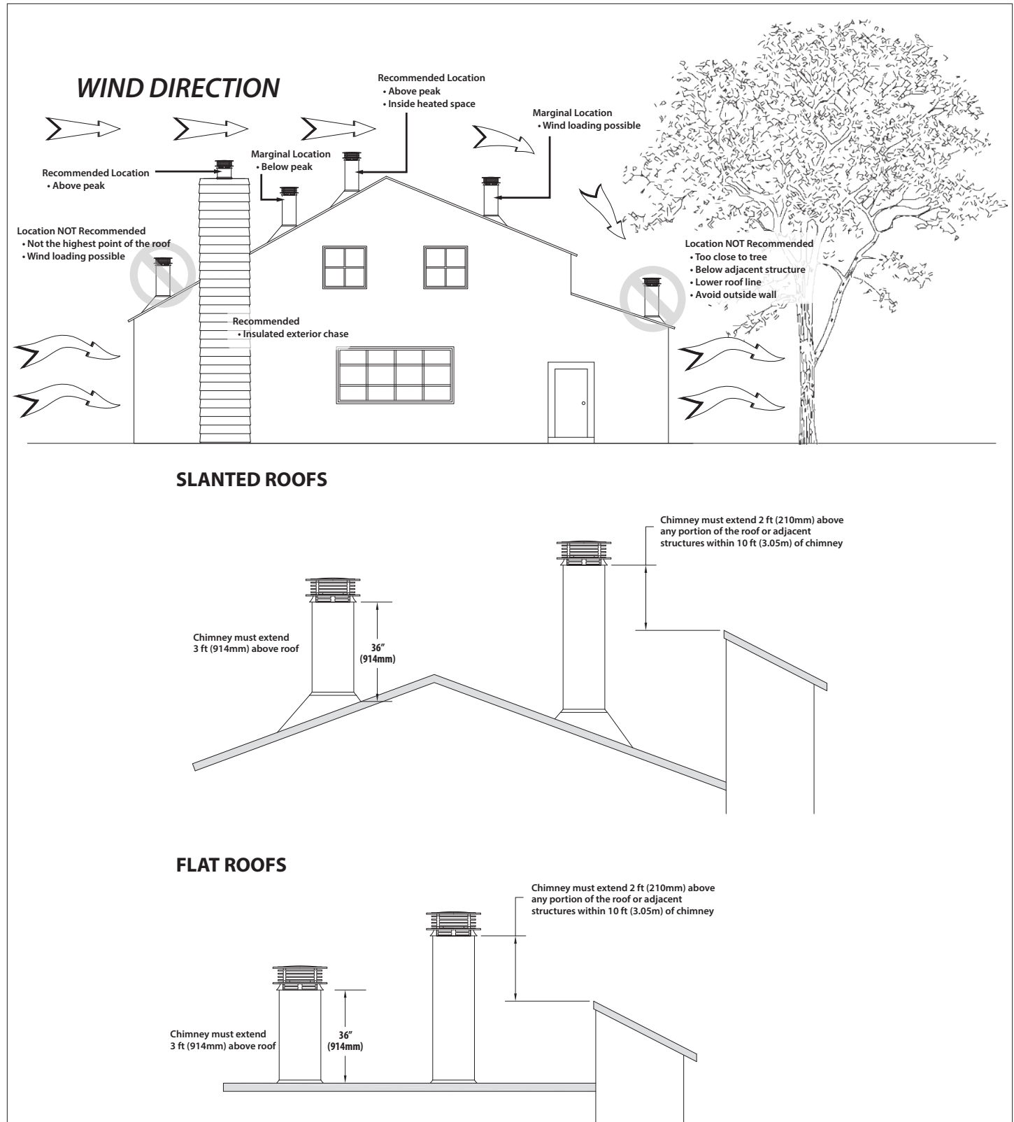
Figure 6.2, Chimney Locations for Roof Types
