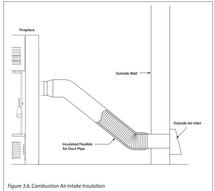
Figure 3.6, Combustion Air Intake Insulation
