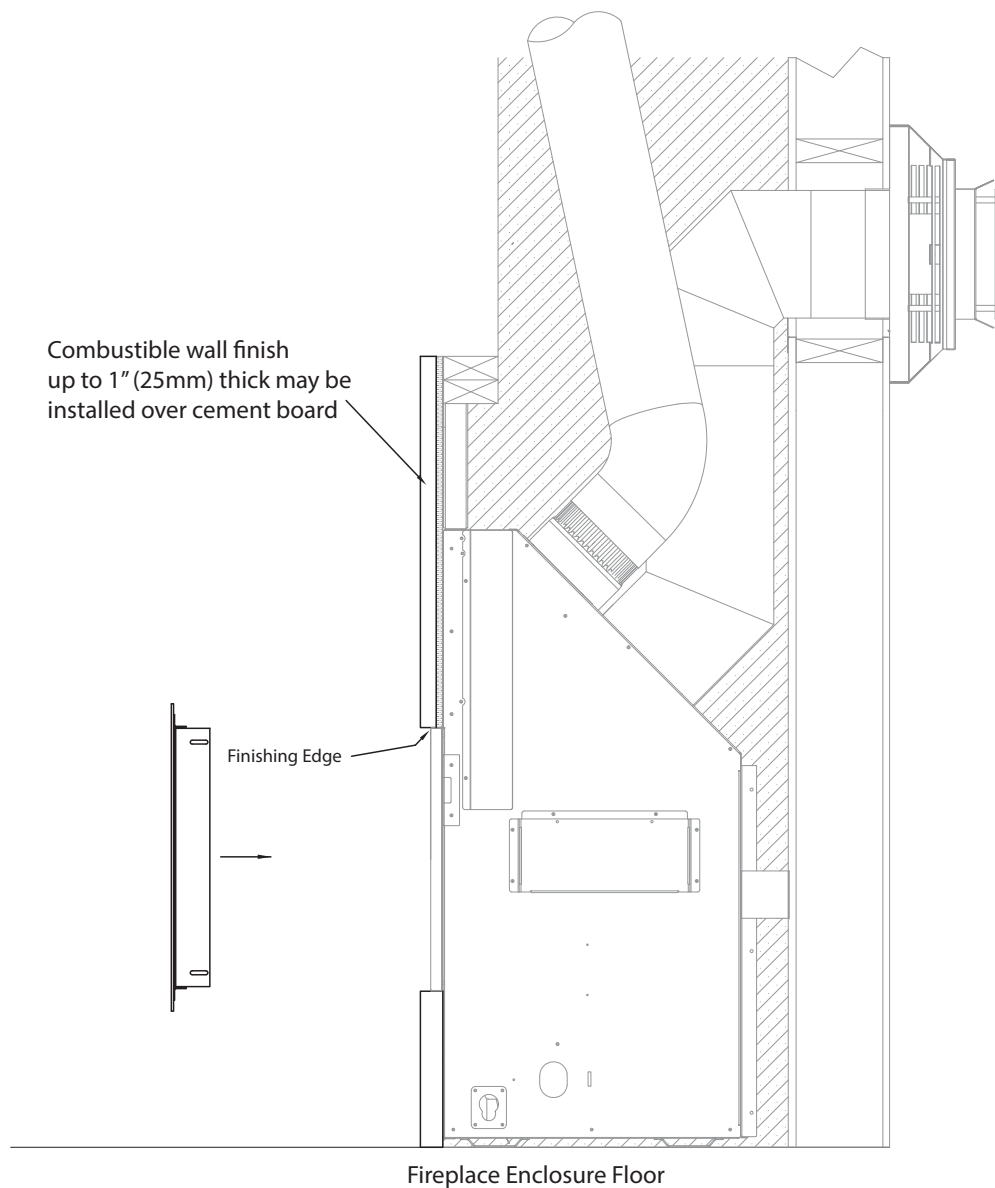
Figure 3.4, KZK-158A Combustible Wall Finish with Surround
