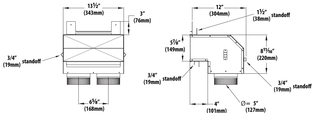
Figure 1.4, KZK-158A Dimensions
