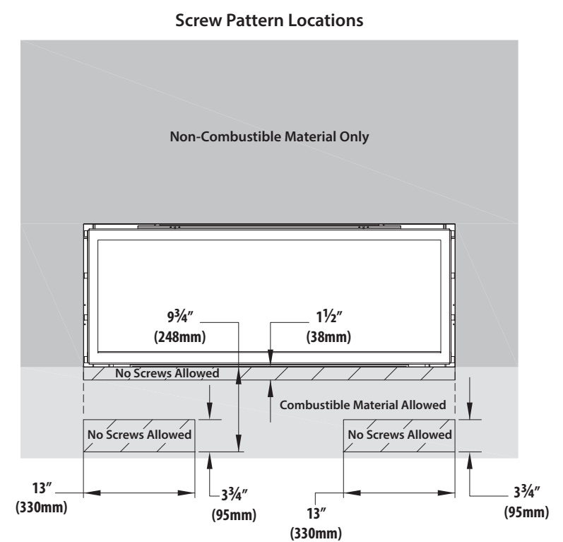
Figure 3.2, Minimum Non-combustible Finishing Dimensions Screw Locations
