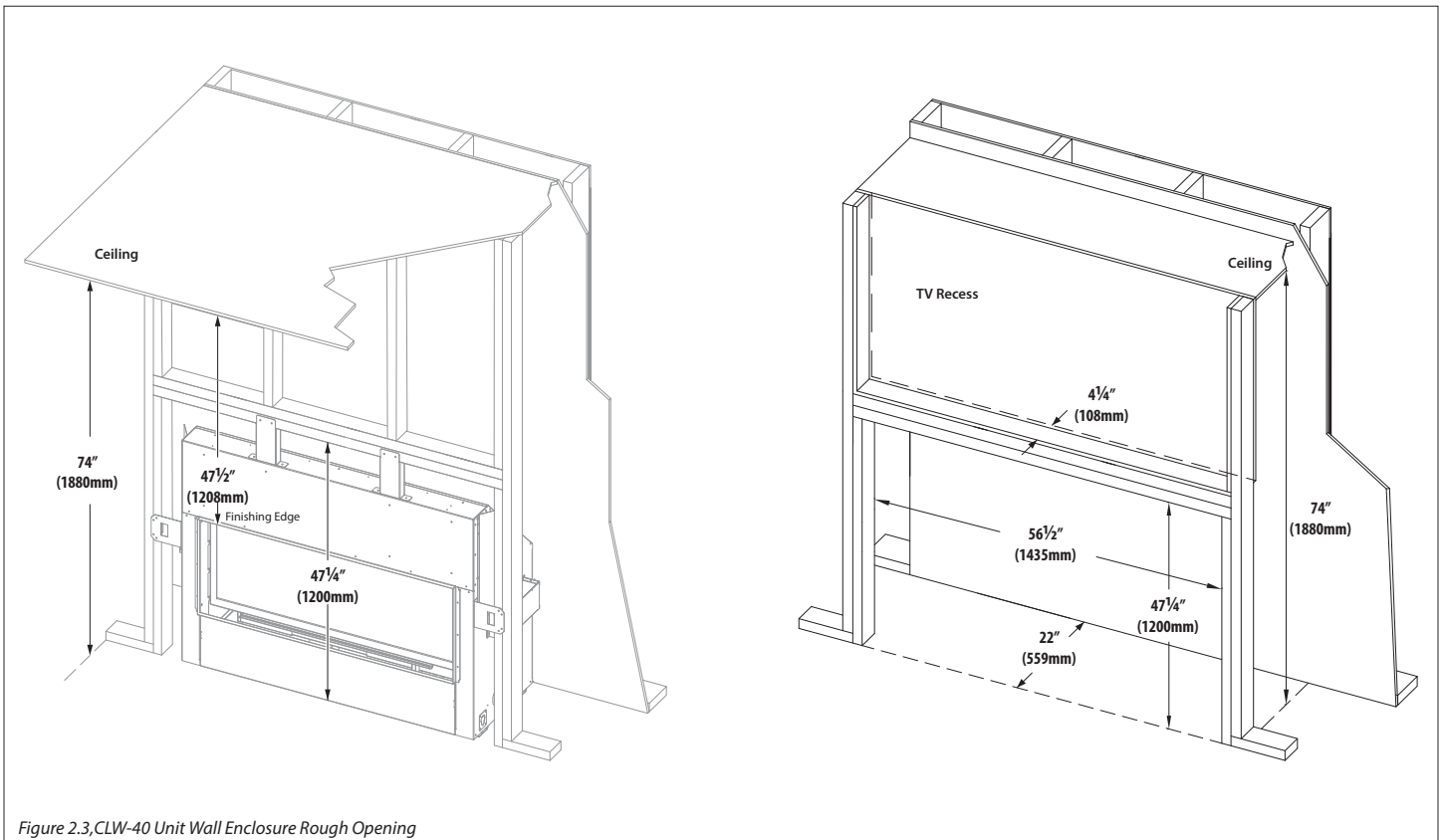
Figure 2.3, CLW-40 Unit Wall Enclosure Rough Opening
