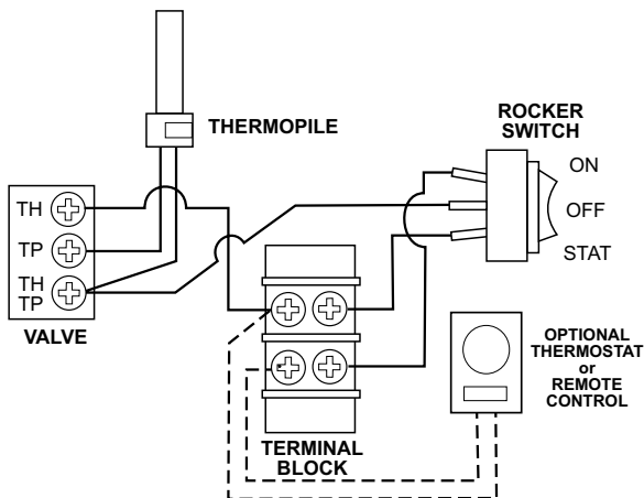
Figure 39. Accessory wiring diagram.
