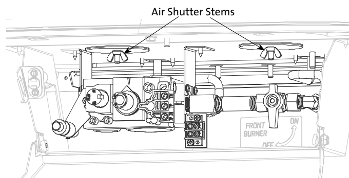
Figure 50. Pull the shutter forward to increase primary air. Push back to restrict air.
