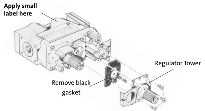
Figure 29. Regulator assembly.
