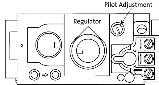
Figure 49. Pilot adjustment at the valve.
