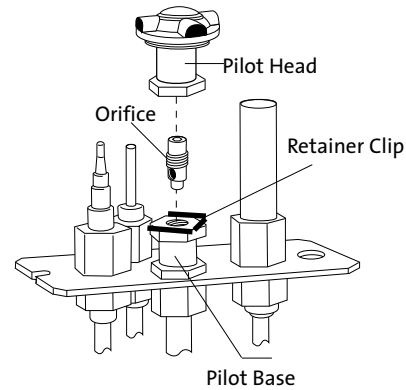
Figure 28. Pilot orifice removal and replacement.
