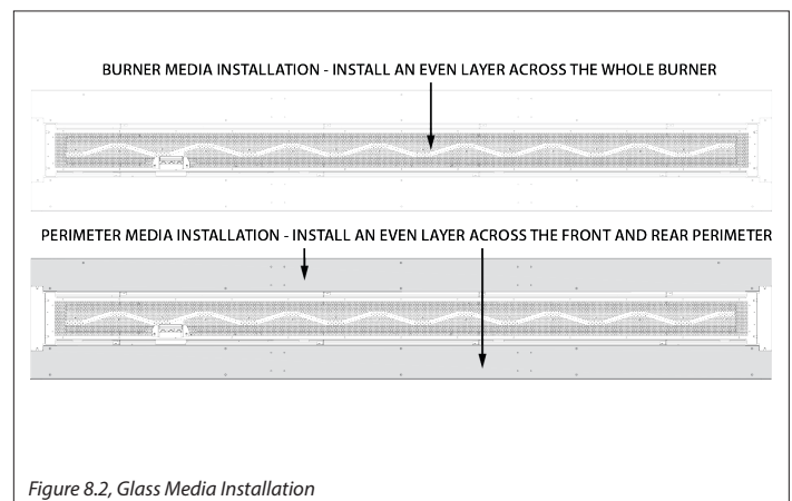
Figure 8.2, Glass Media Installation
