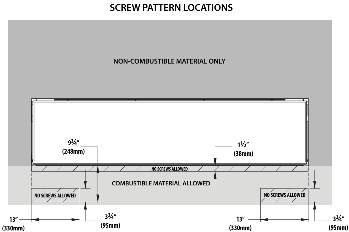
Figure 4.5, Minimum Non-Combustible Finishing Dimensions Screw Locations
