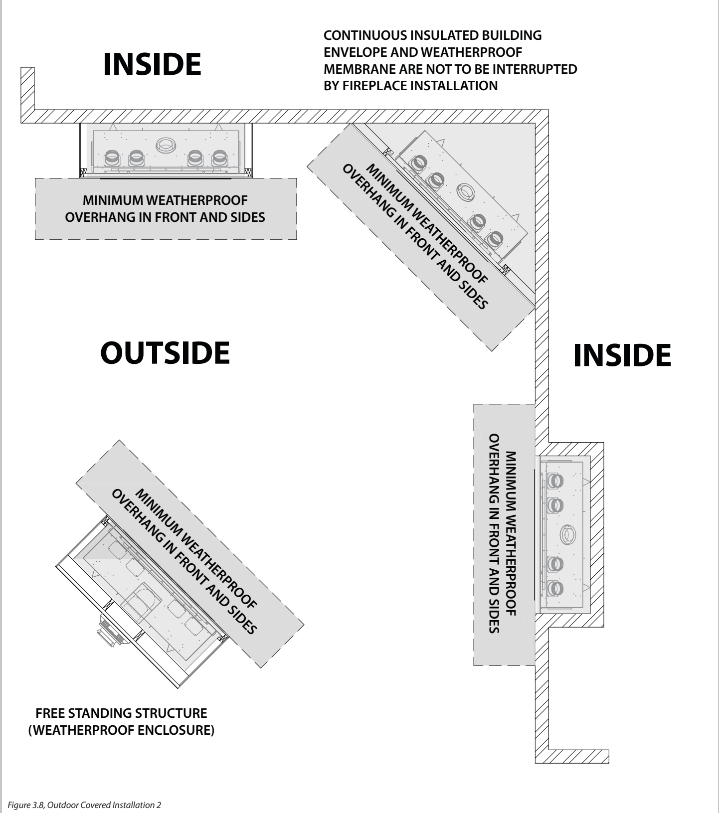
Figure 3.8, Outdoor Covered Installation 2
