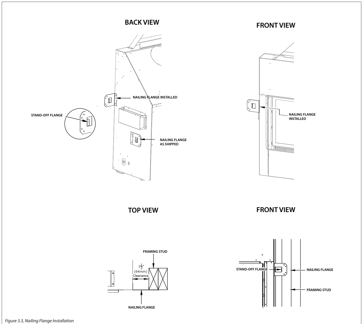
Figure 3.3, Nailing Flange Installation
