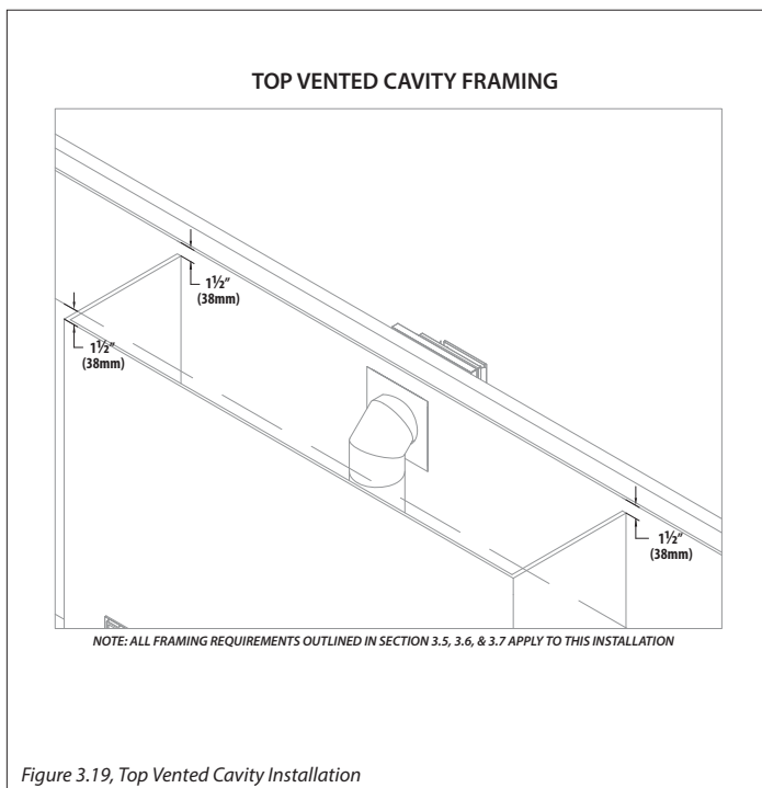
Figure 3.19, Top Vented Cavity Installation
