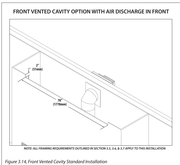
Figure 3.14, Front Vented Cavity Standard Installation
