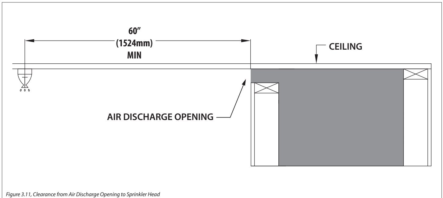
Figure 3.11, Clearance from Air Discharge Opening to Sprinkler Head
