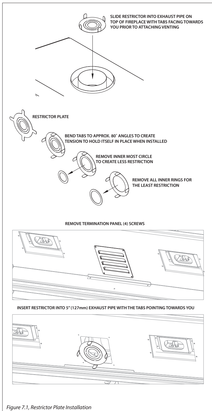
Figure 7.1, Restrictor Plate Installation
