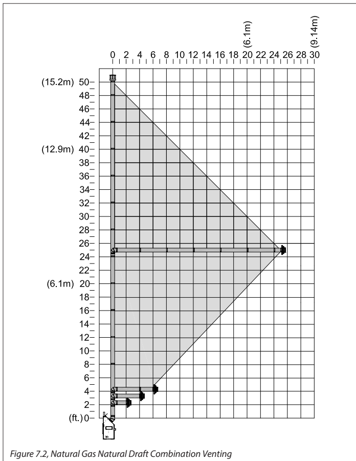
Figure 7.2, Natural Gas Natural Draft Combination Venting
