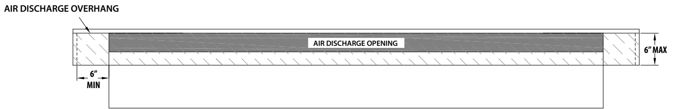
Figure 3.21, Top Vented Cavity Alternative Installation with Overhang
