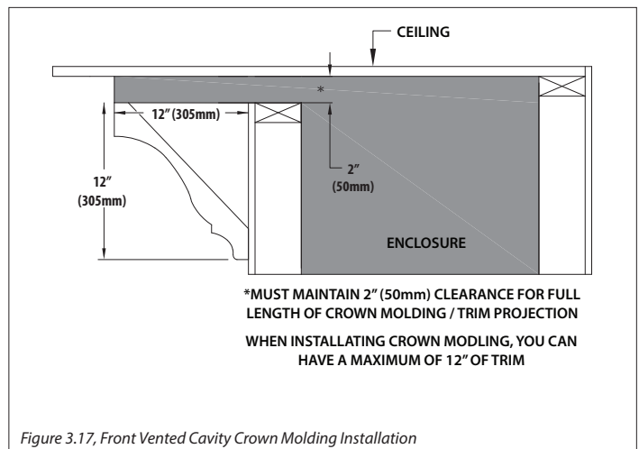
Figure 3.17, Front Vented Cavity Crown Molding Installation
