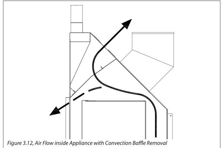
Figure 3.12, Air Flow inside Appliance with Convection Baffle Removal
