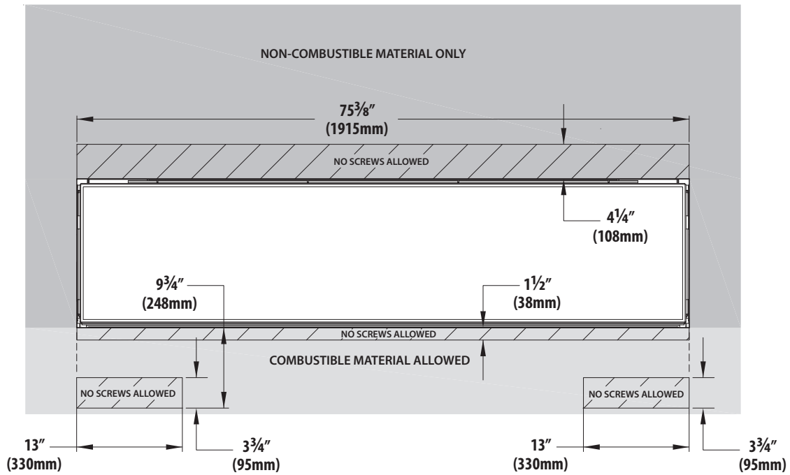
Figure 4.5, Minimum Non-Combustible Finishing Dimensions Screw Locations
