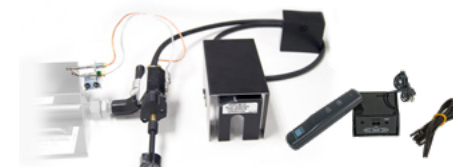
APK-17(M)(P) Low Profile, Automatic Safety Pilot System
