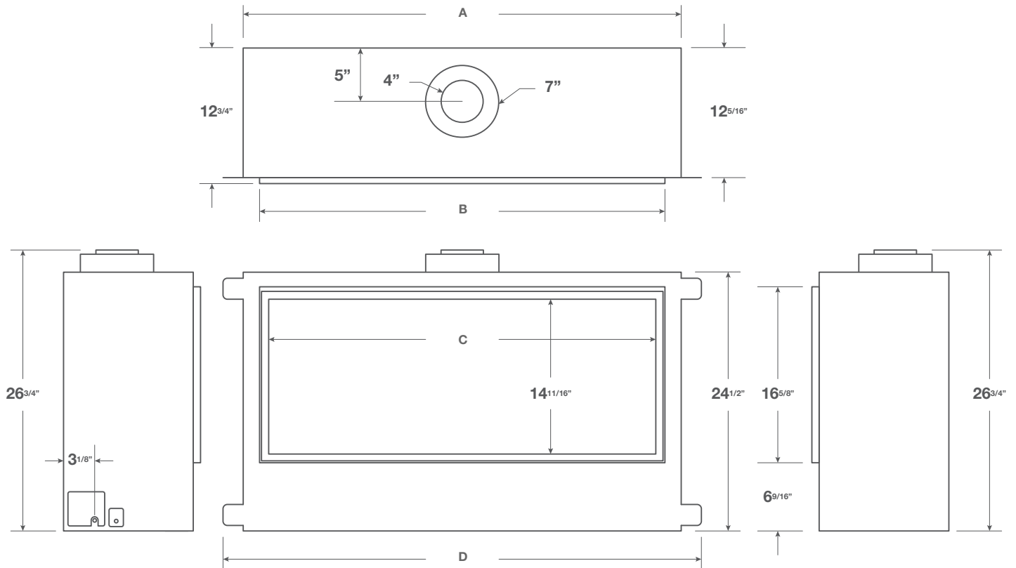
Figure 2. DeRay Fireplace dimensions (Tolerance \pm \frac{1}{16}" ).
