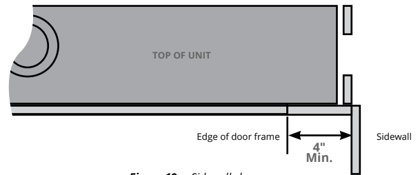
Figure 19.c Sidewall clearances
