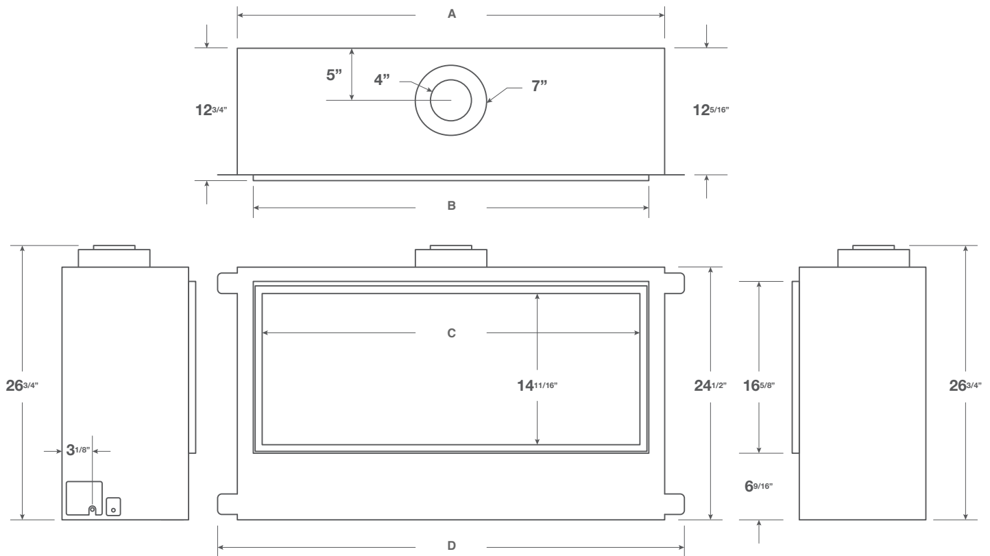
Figure 2. DeRay Fireplace dimensions (Tolerance \pm \frac{1}{16}" ).
