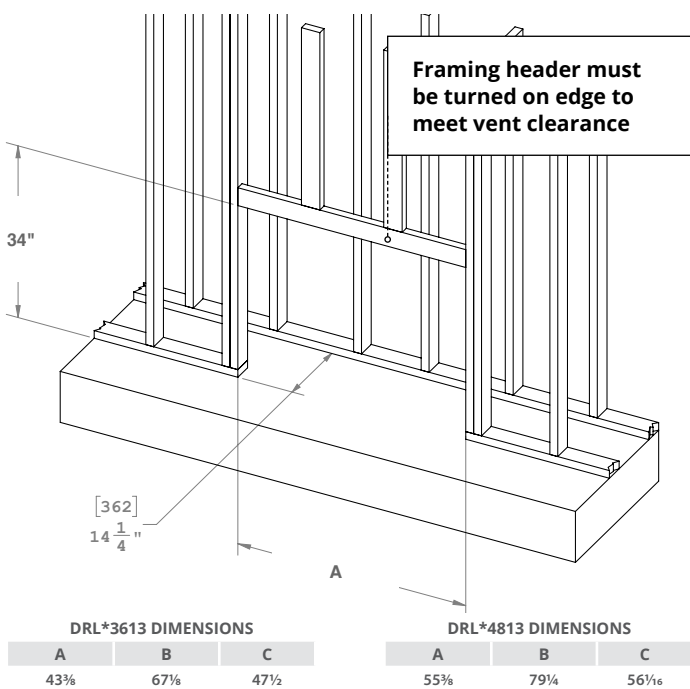
Figure 3.a Framing dimensions table
