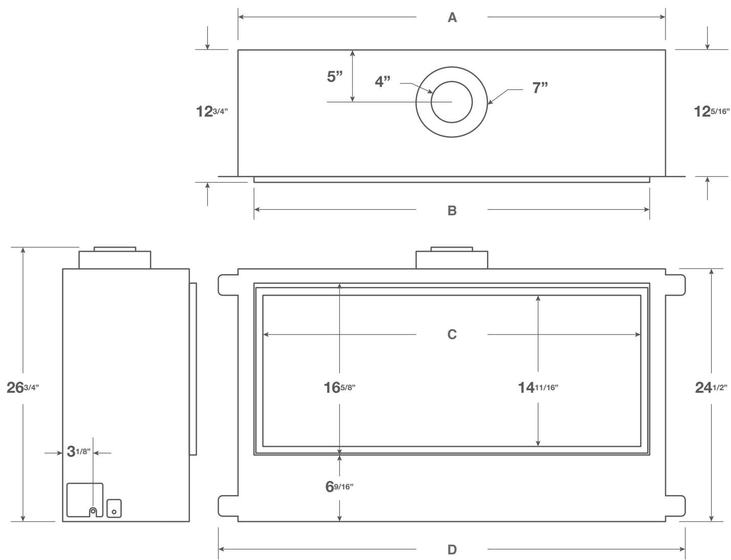
Figure 2. DelRay Fireplace dimensions (Tolerance \pm \frac{1}{16}" ).
