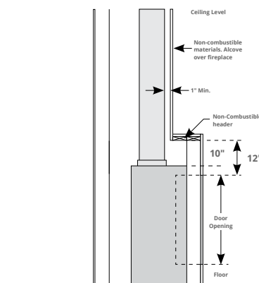
Figure 3.d Non-combustible Framing for shelves over the fireplace
