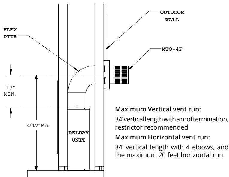
Figure 4.bb Minimum Horizontal vent run (Flex)
