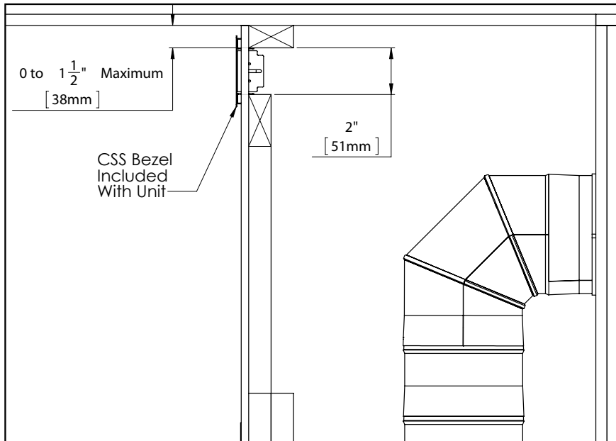
Figure 39A: Option 3 Bezel
