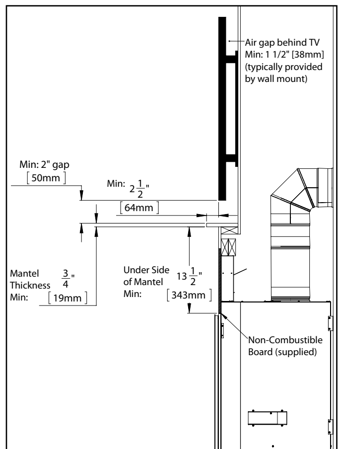
Figure 49. Recess Minimum TV Install
