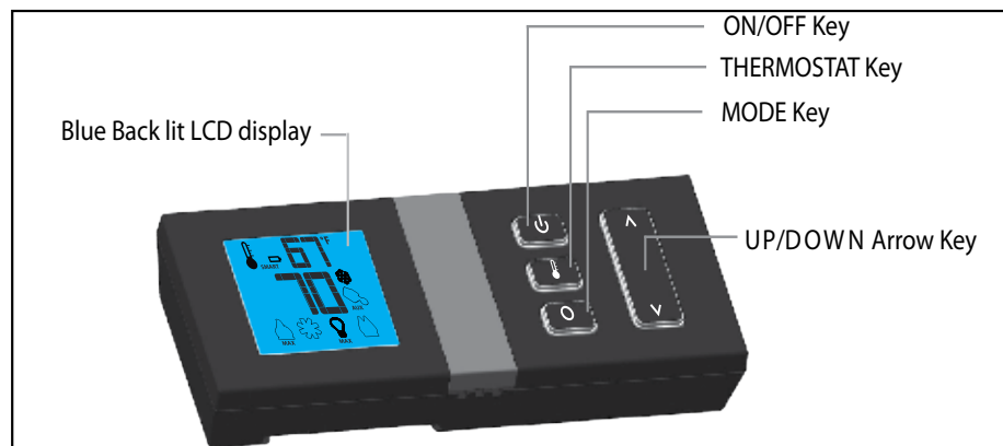
Figure 3: Proflame 2 Transmitter.
