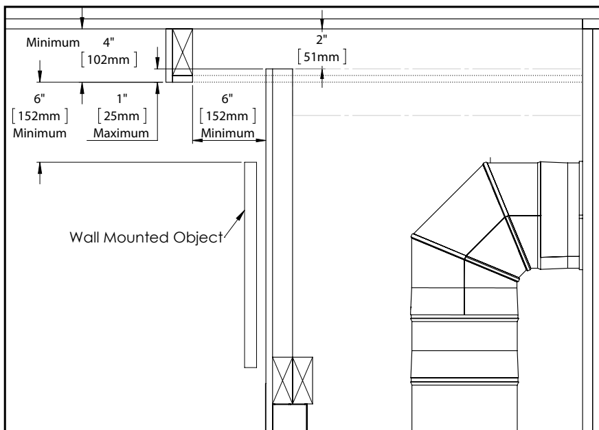
Figure 38A: Valance Install
