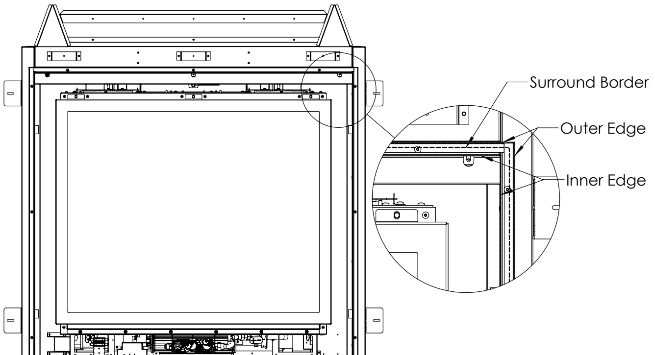
Figure 32: Finishing edges
