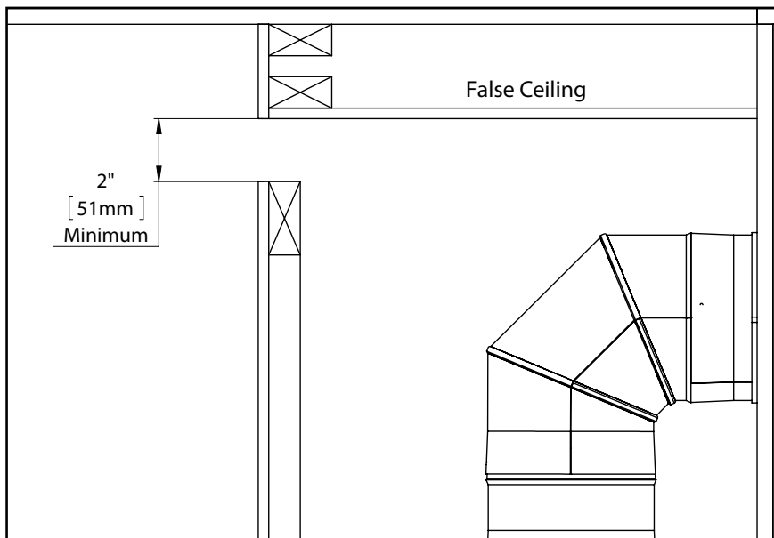
Figure 40A: False Ceiling
