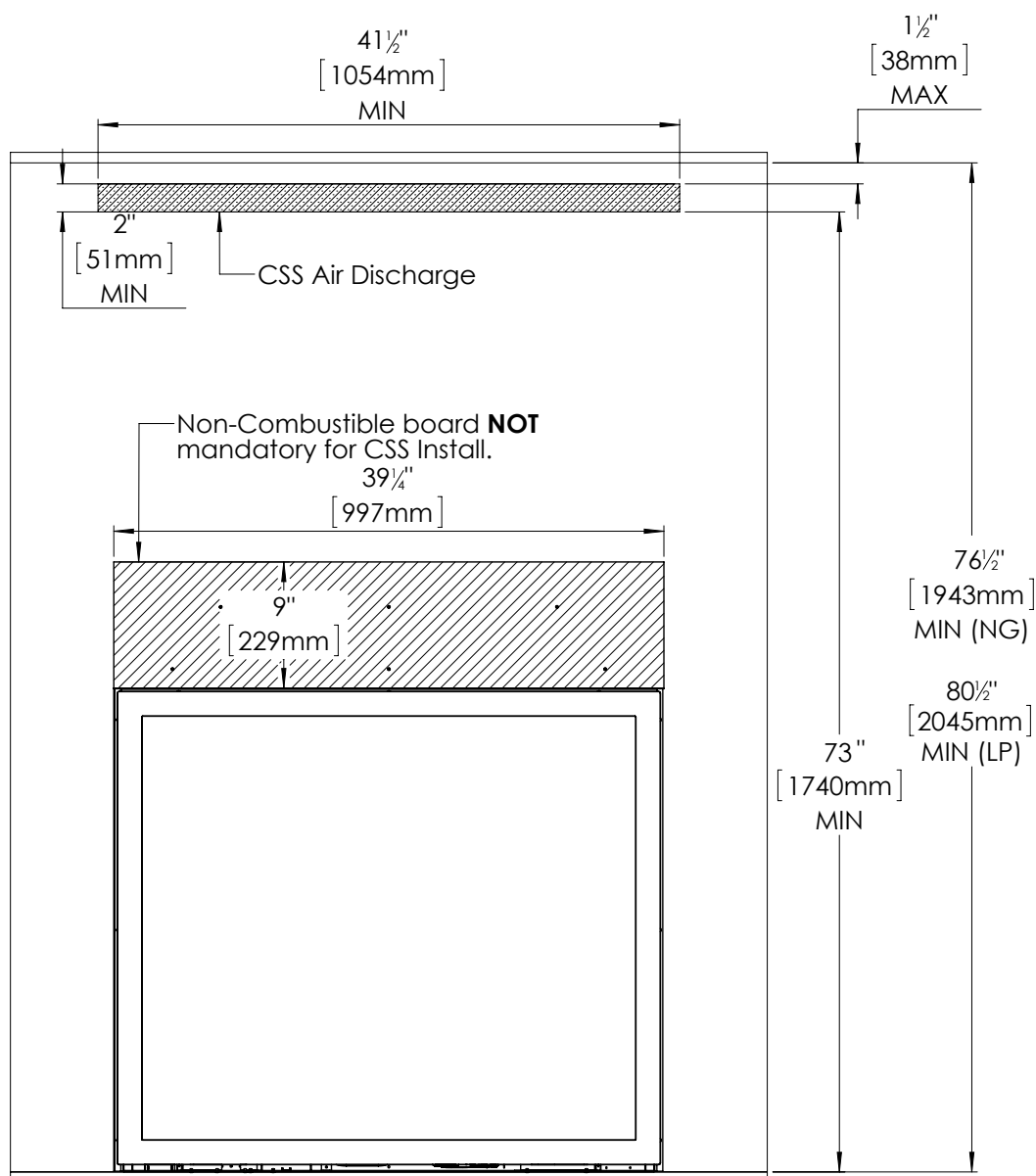
Figure 36: CSS Front Discharge
