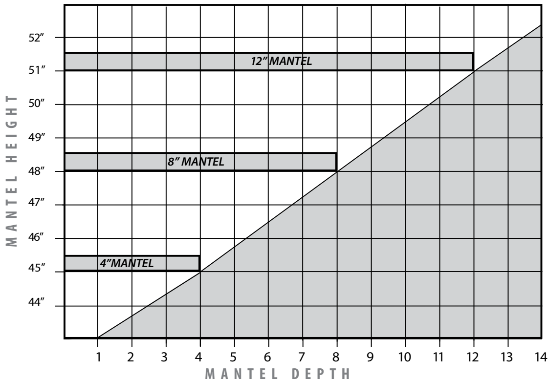
Diagram 2: Mantel Graph
