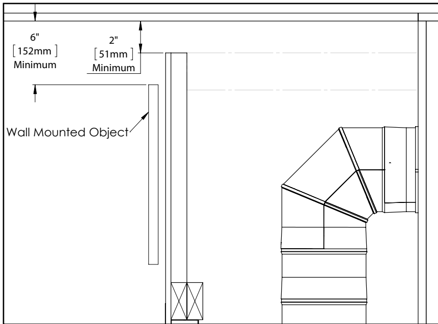
Figure 37A: Option 2
