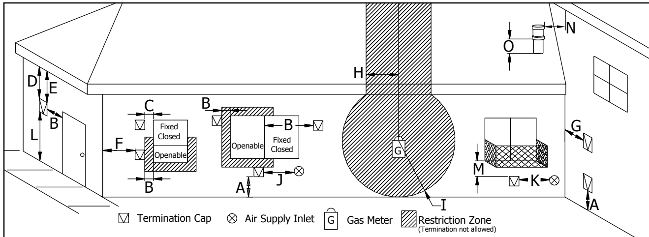
Figure 50. Vent Termination Restrictions, refer to Table 4
