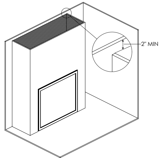
Figure 37B: Open Chase Iso View
