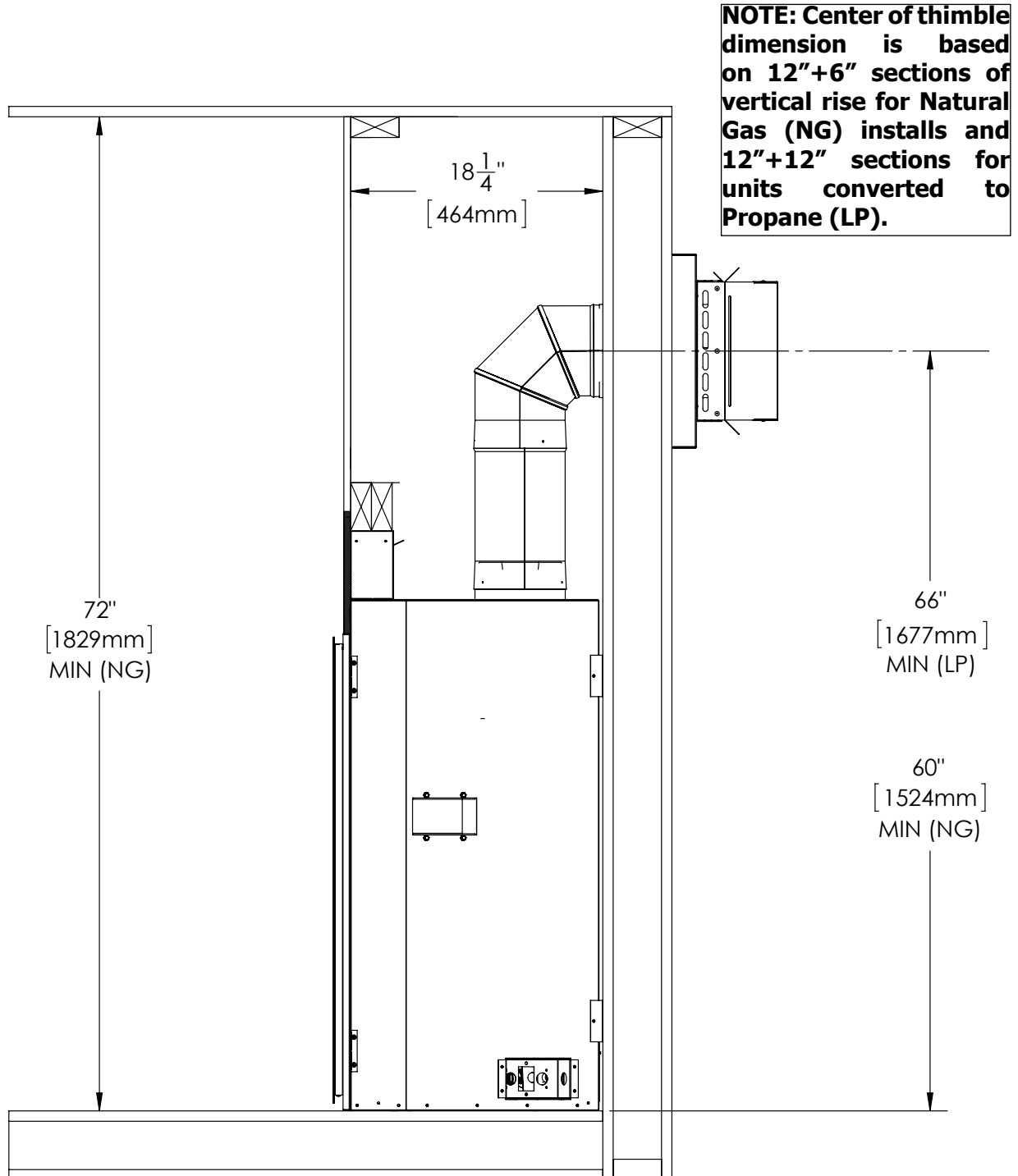
Figure 45: Minimum Vent (NG)
