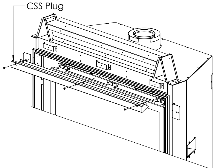
Figure 35: CSS Plug Removal
