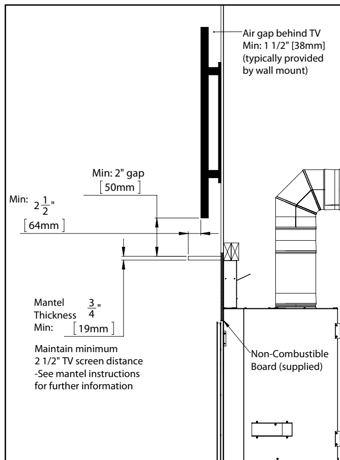
Figure 48. Minimum TV Install
