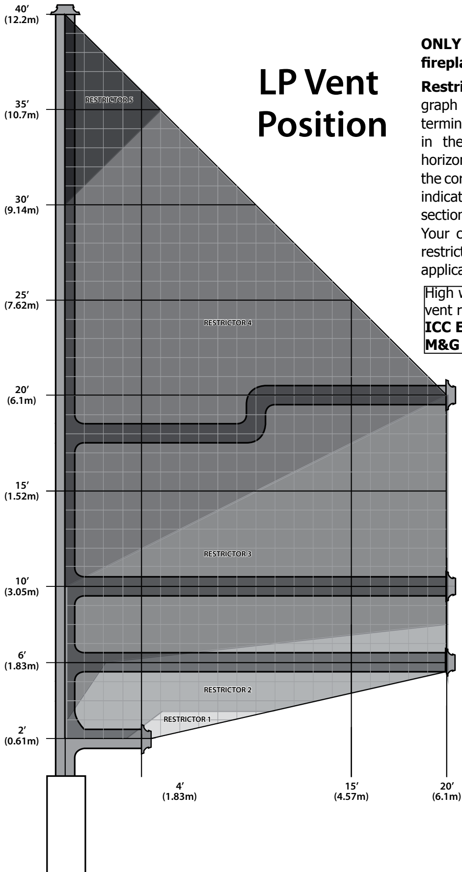
Figure 53. LP Vent Graph
