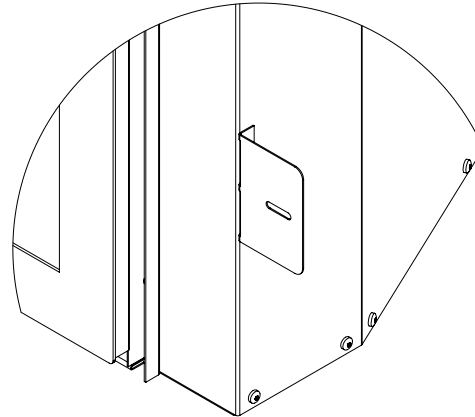
Figure 28: Nailing Flange Assembled
