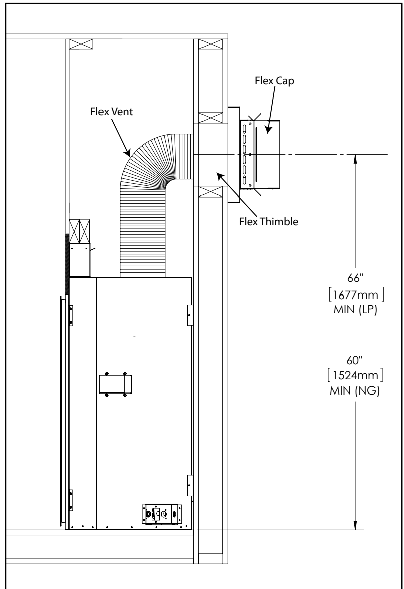
Figure 46. Flex Vent Install
