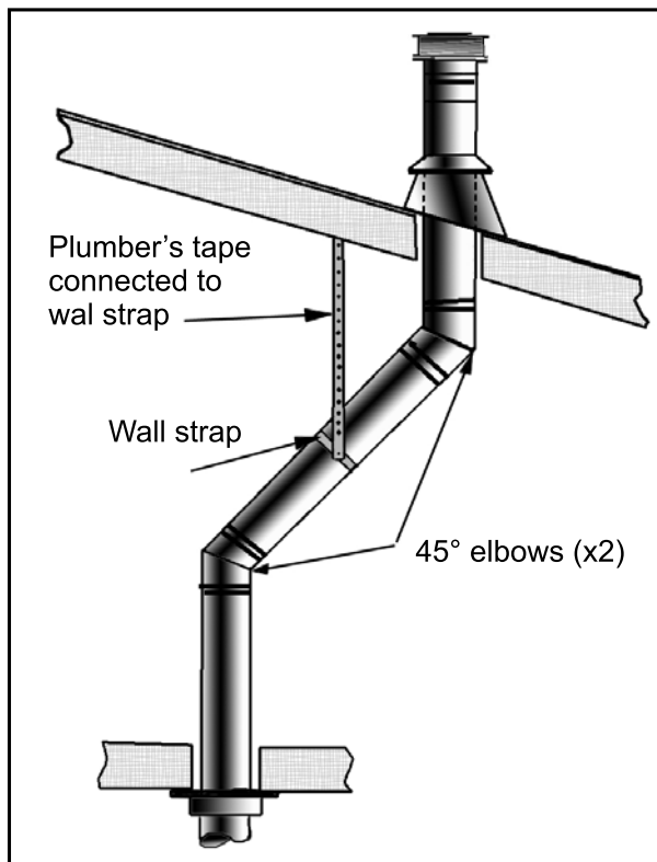
Figure 59: Multi-Story Vent Pipe Installation
