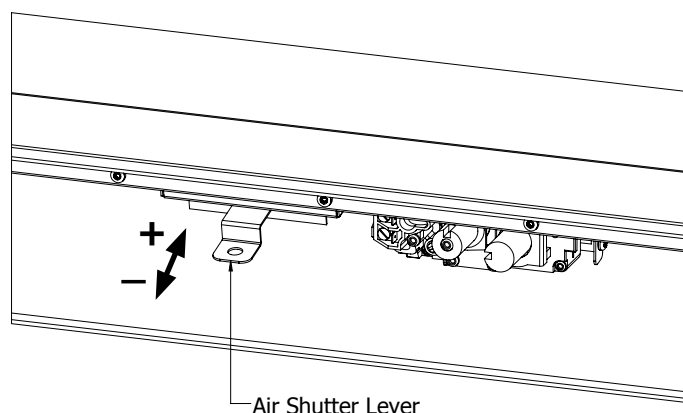
Figure 17. Air Shutter Location
