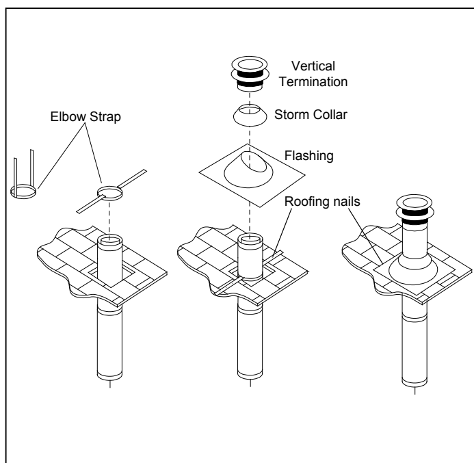
Figure 57. Vertical Vent Termination
