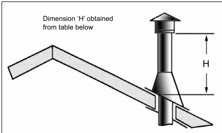
Figure 58: Height of Vertical Termination; Reference Table 8
