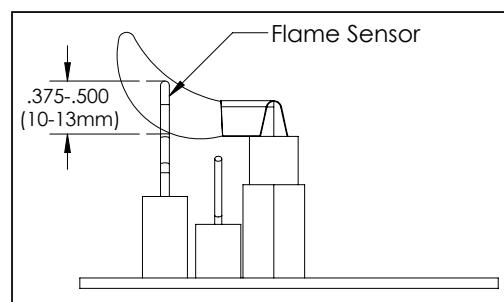
Figure 16. Pilot Light
