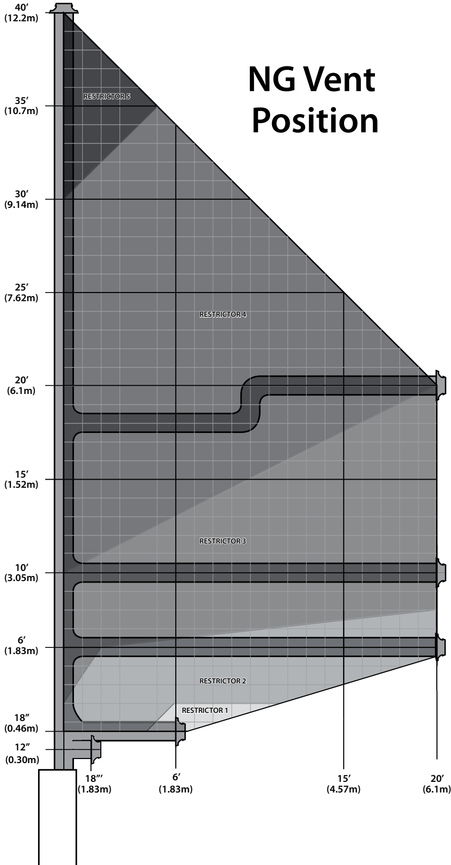
Figure 52. Natural Gas Vent Graph
