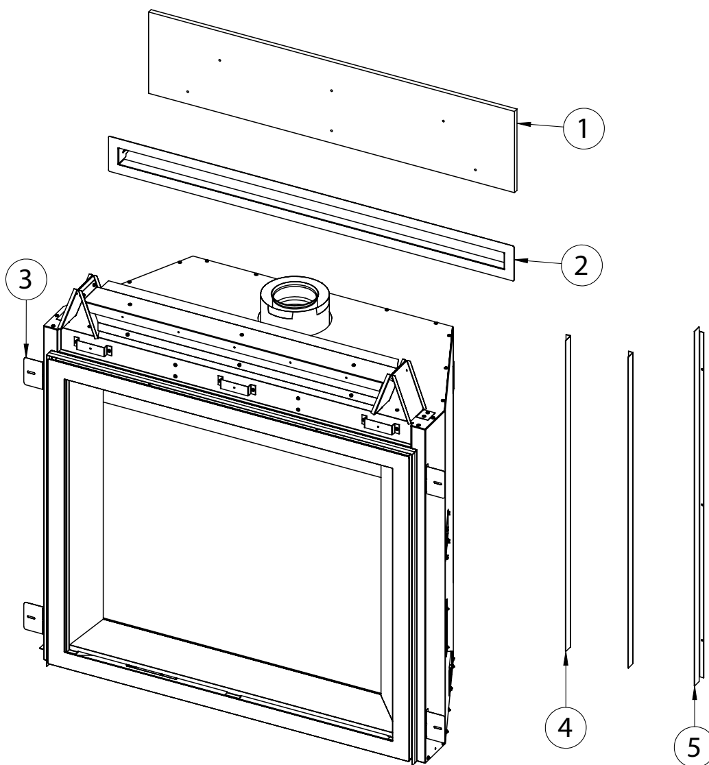
Diagram 1: Additional Parts
