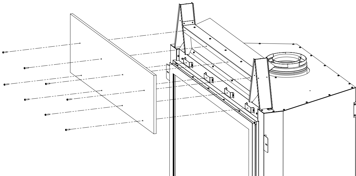
Figure 29: Non-combustible board
