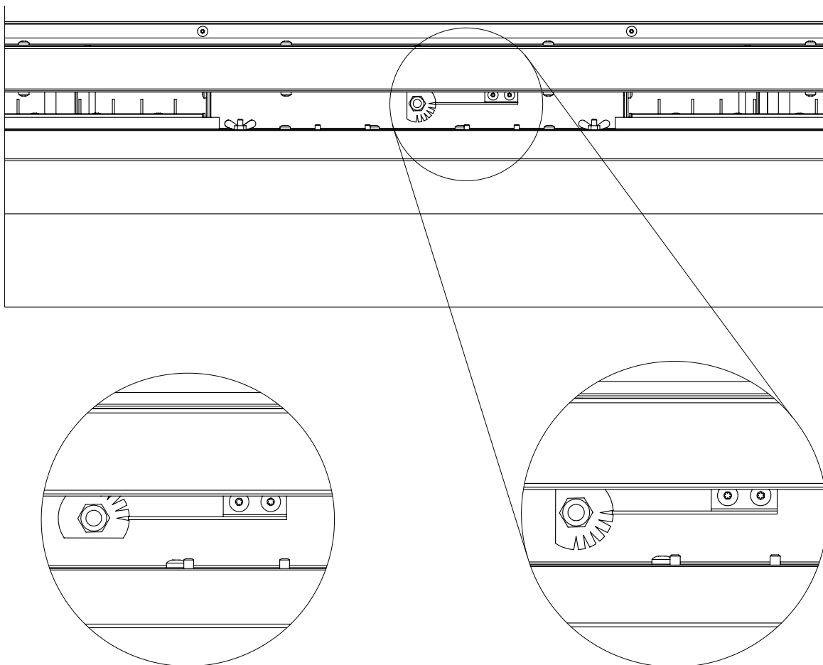
Figure 54. Restrictor Setting 6
