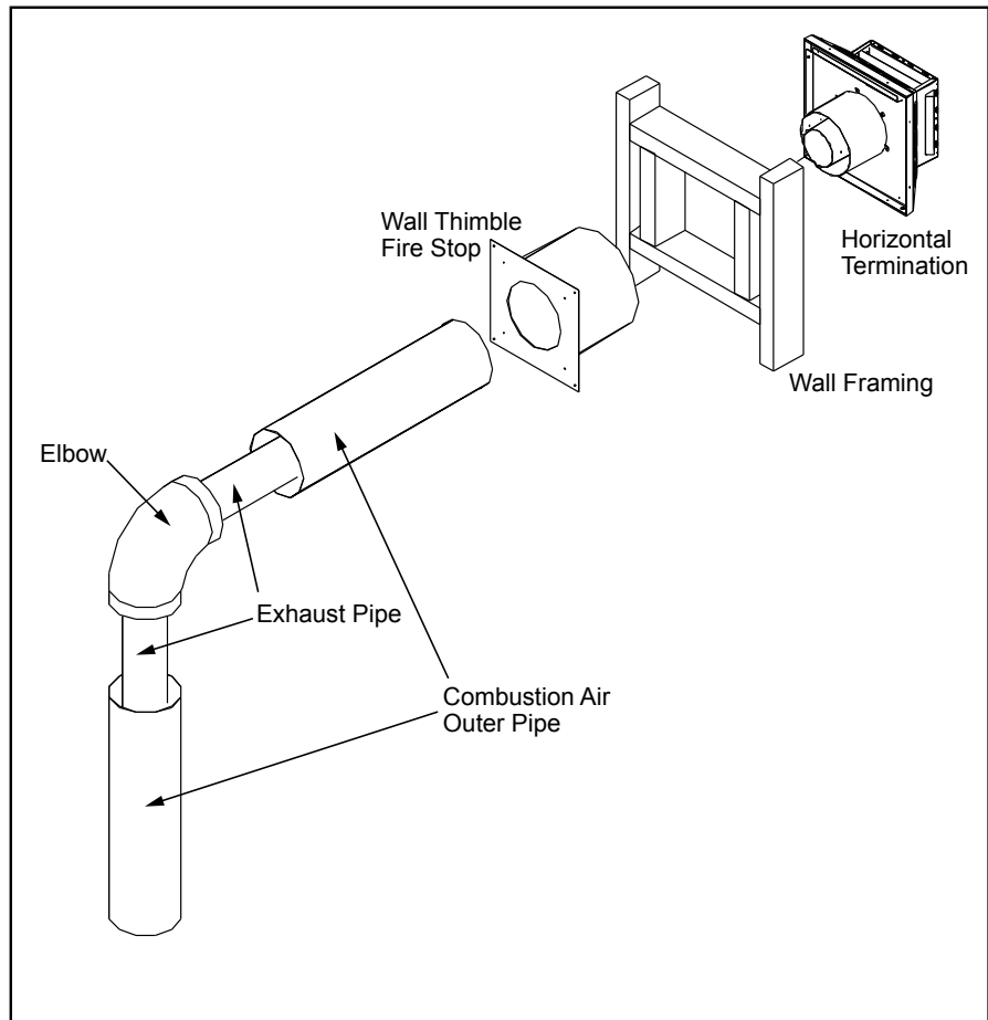
Figure 56. Horizontal Vent Termination
