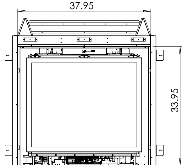
Figure 34: Inner Finishing Edge Dims
