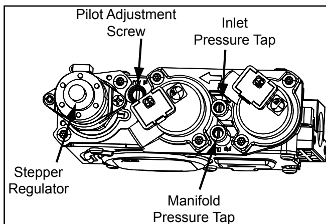
Figure 61: Fully Labeled Gas Valve.
