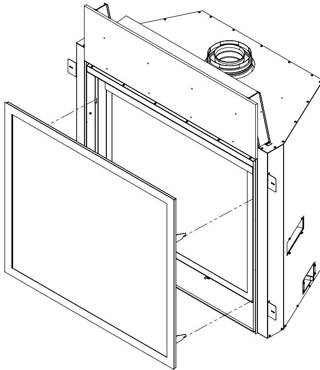
Figure 18. Surround Removal
