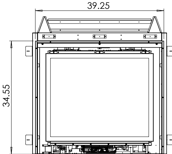
Figure 33: Outer Finishing Edge Dims
