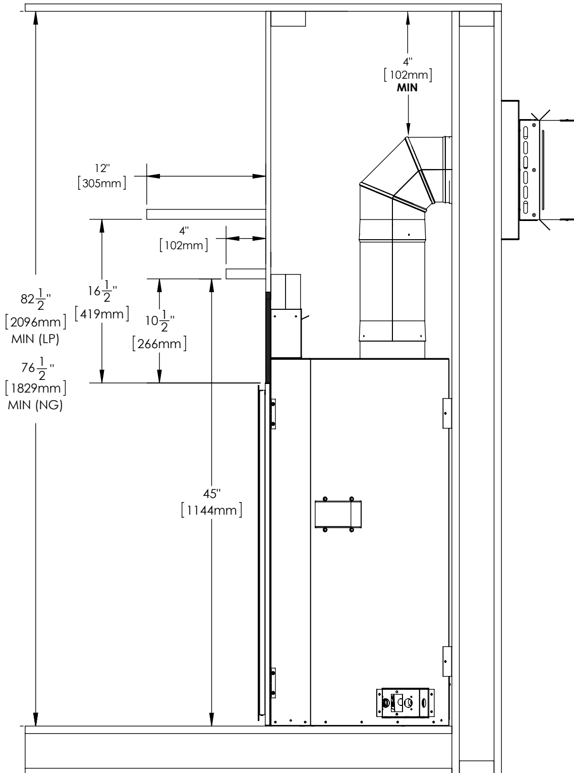
Figure 41: Flat Wall Installation
