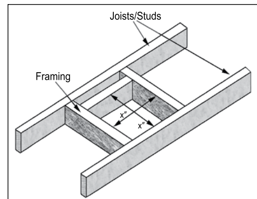
Figure 51. Thimble Framing
