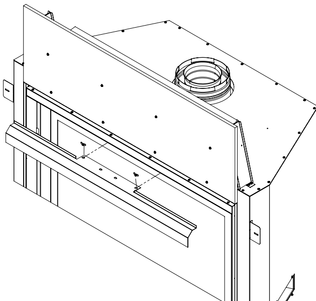
Figure 19. Door Cover Removal
