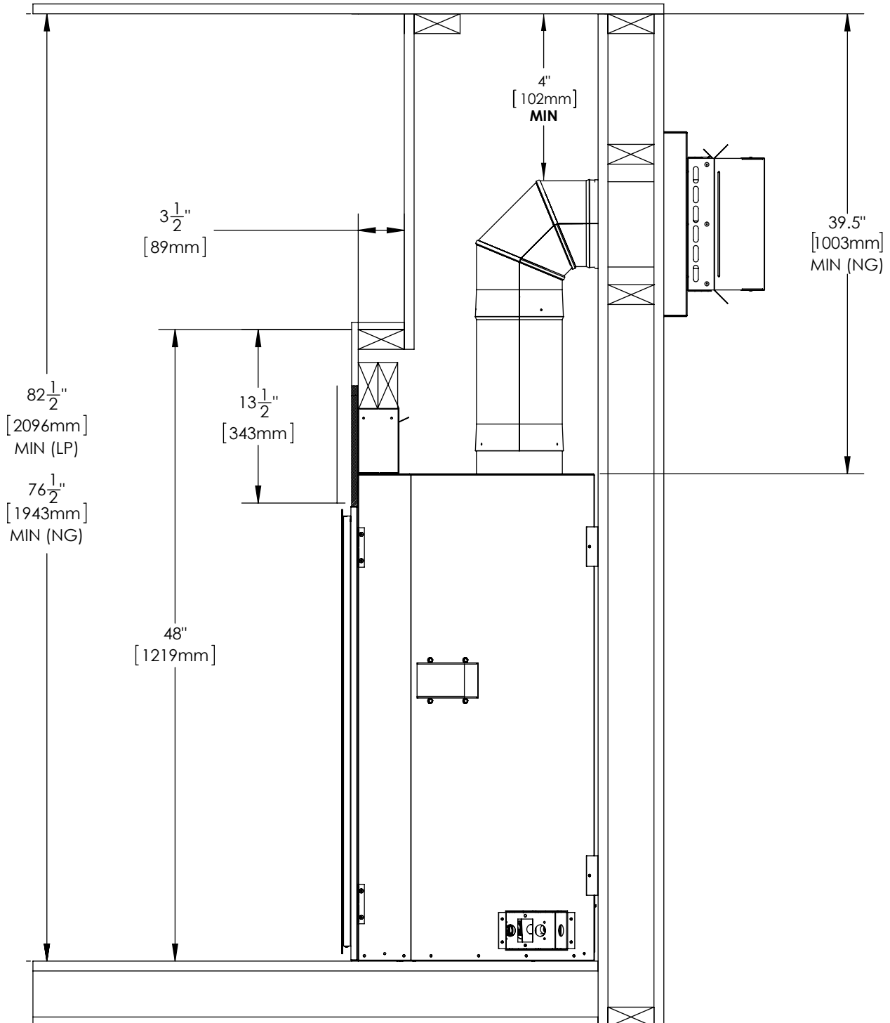
Figure 42: Recess Installation
