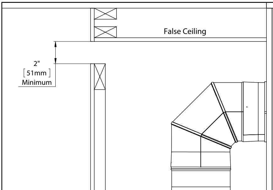
Figure 46A: False Ceiling
