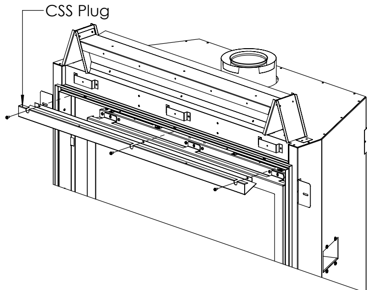
Figure 41: CSS Plug Removal
