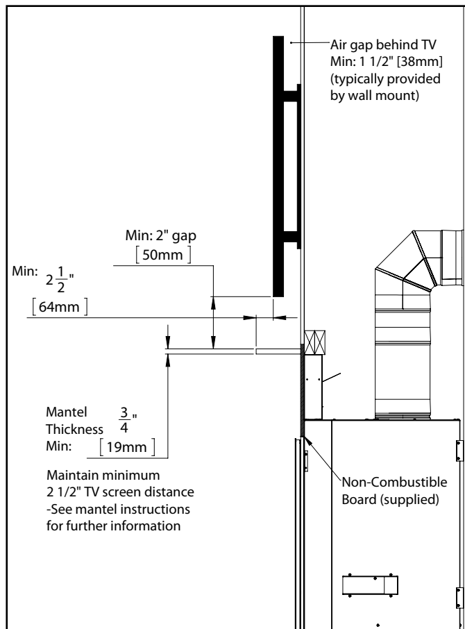
Figure 54. Minimum TV Install
