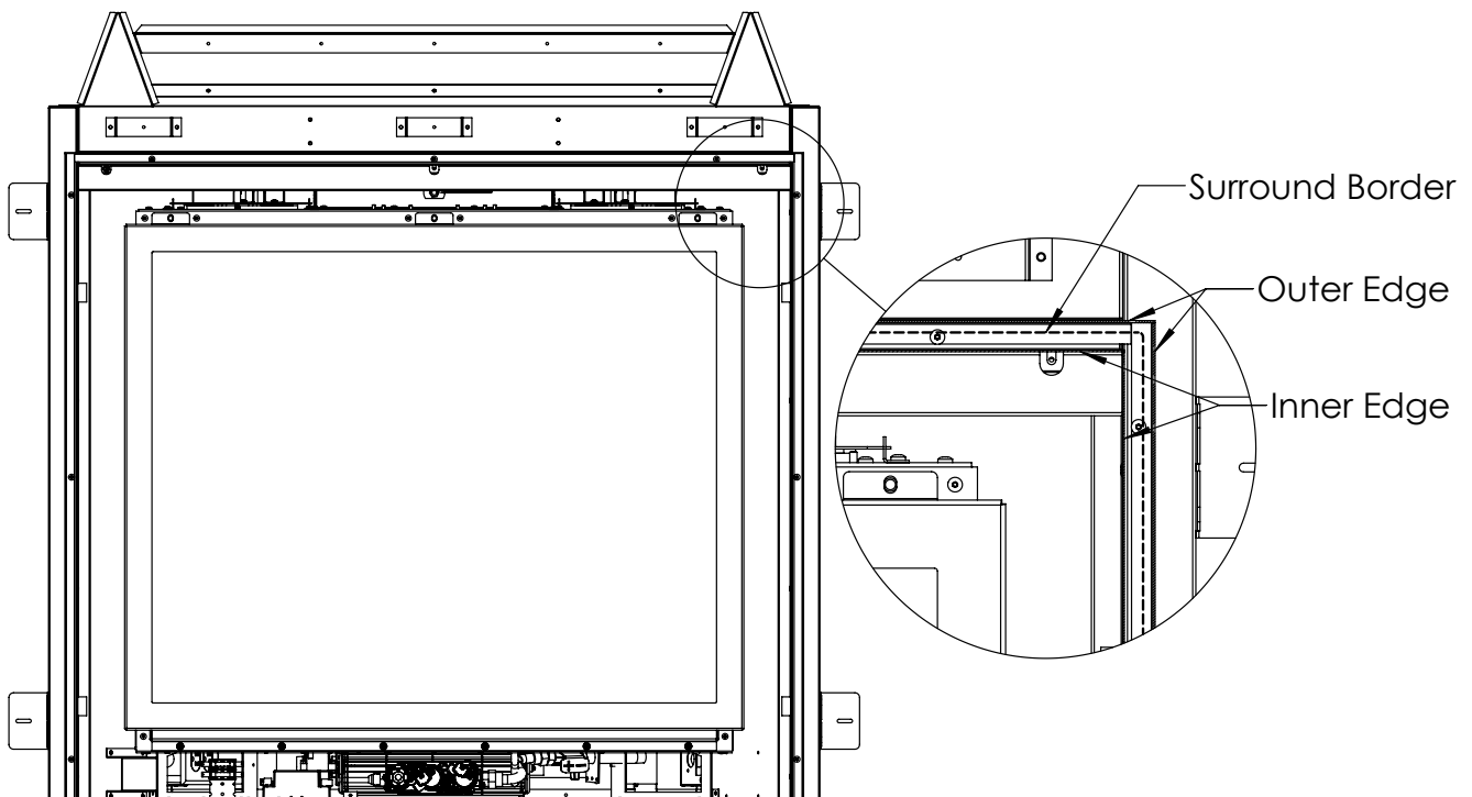
Figure 38: Finishing edges
