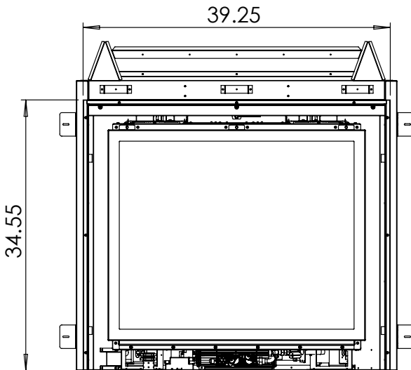
Figure 39: Outer Finishing Edge Dims
