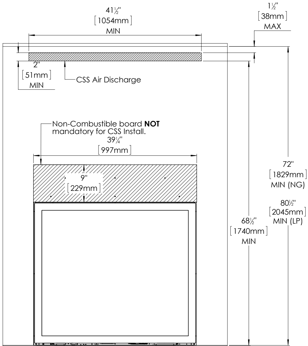
Figure 42: CSS Front Discharge
