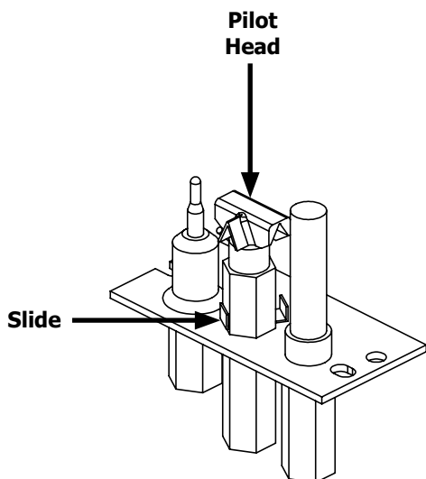
Figure 28: Pilot Assembly
