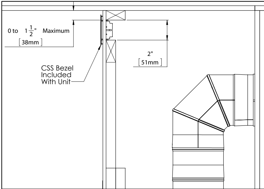
Figure 45A: Option 3 Bezel
