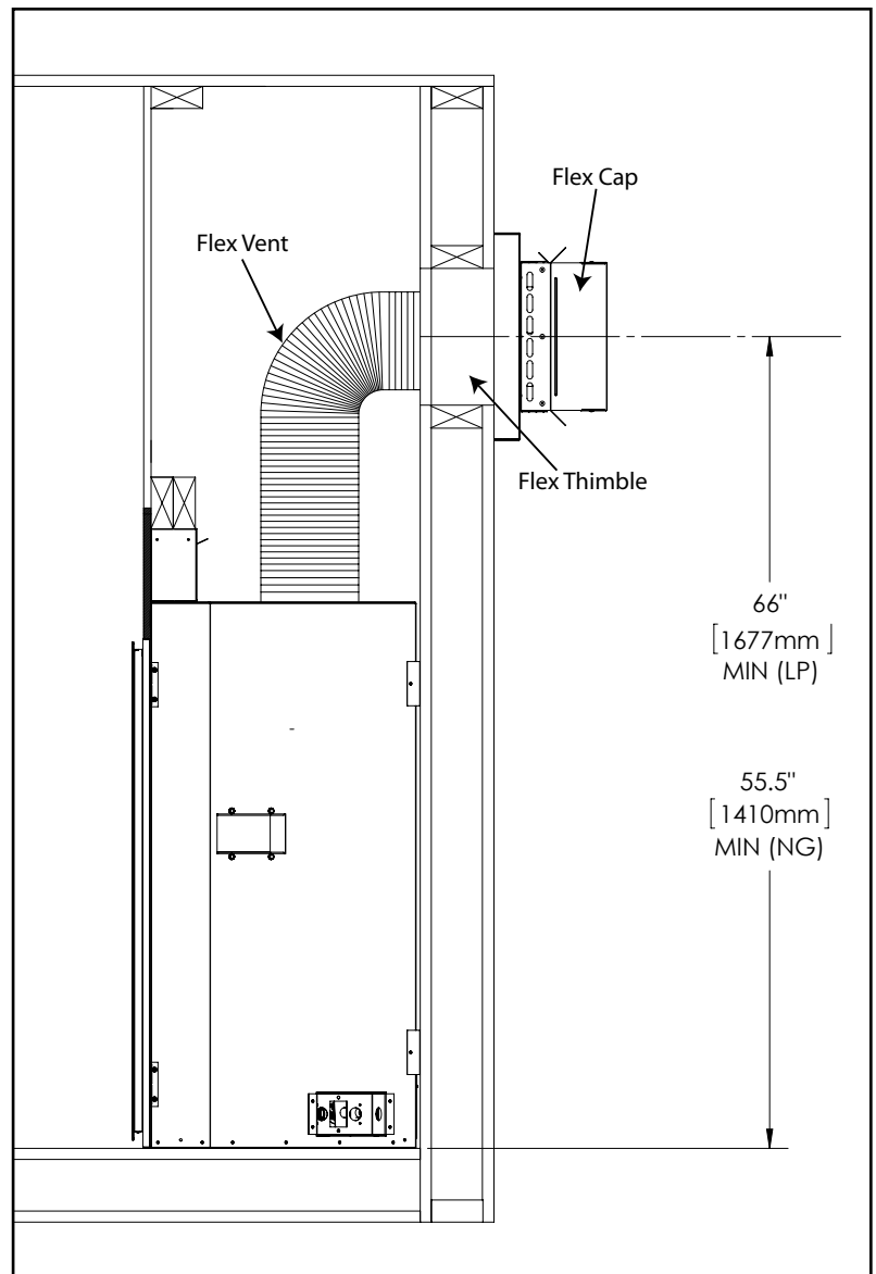
Figure 52. Flex Vent Install
