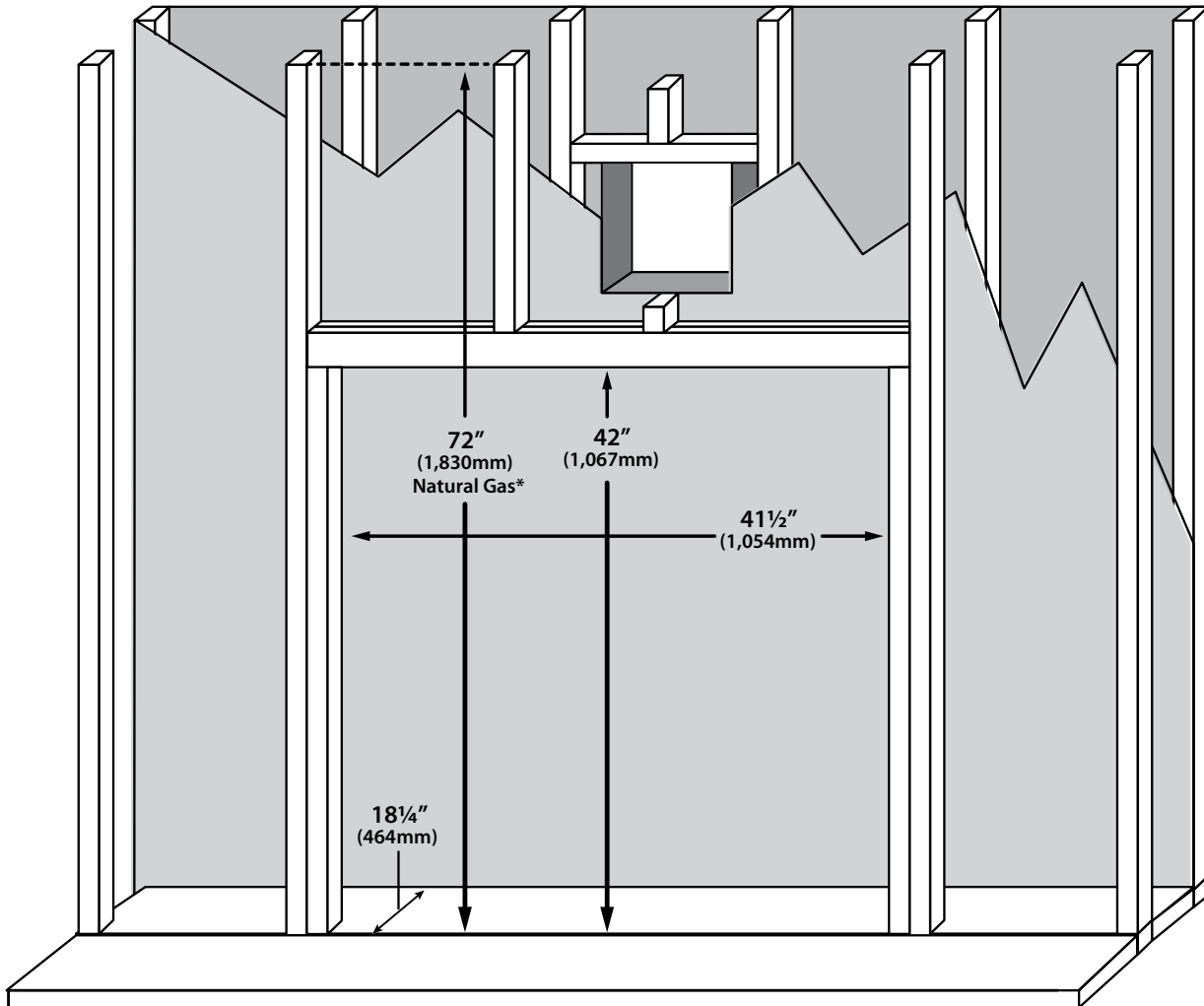
Figure 36: G39 Minimum Framing
