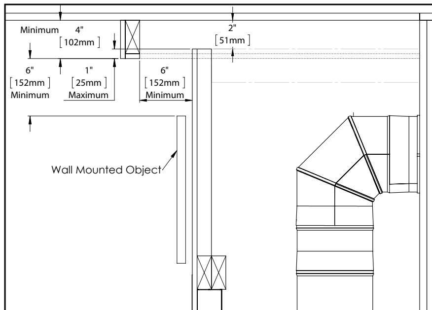
Figure 44A: Valance Install
