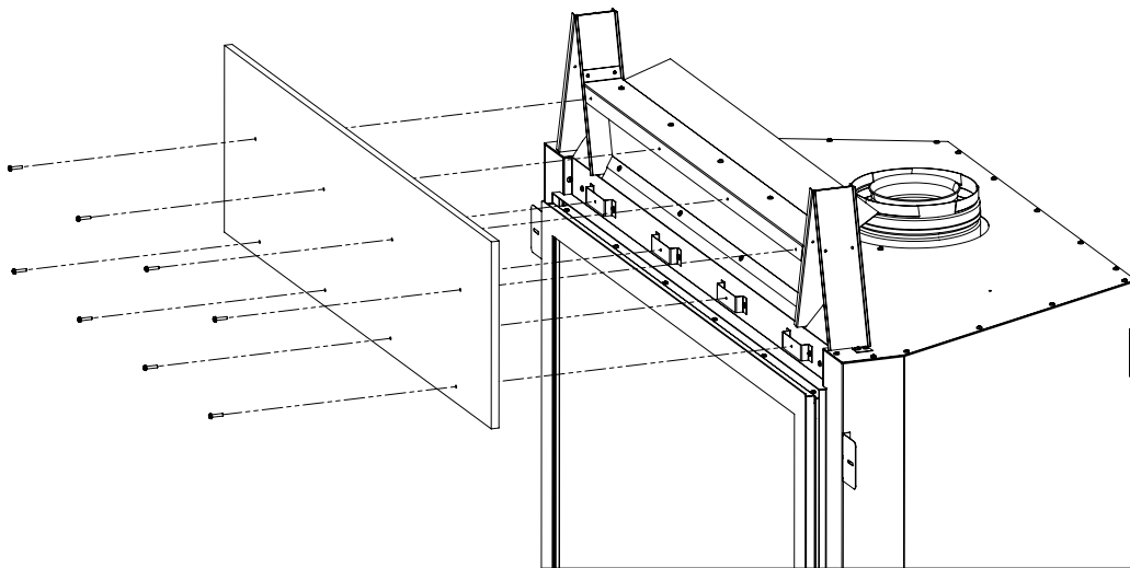
Figure 35: Non-combustible board
