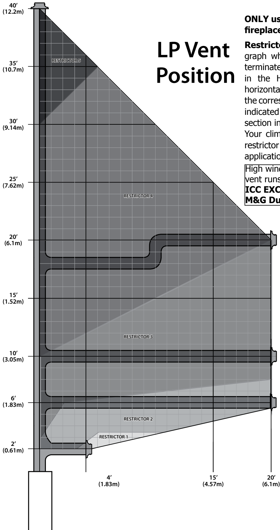
Figure 59. LP Vent Graph
