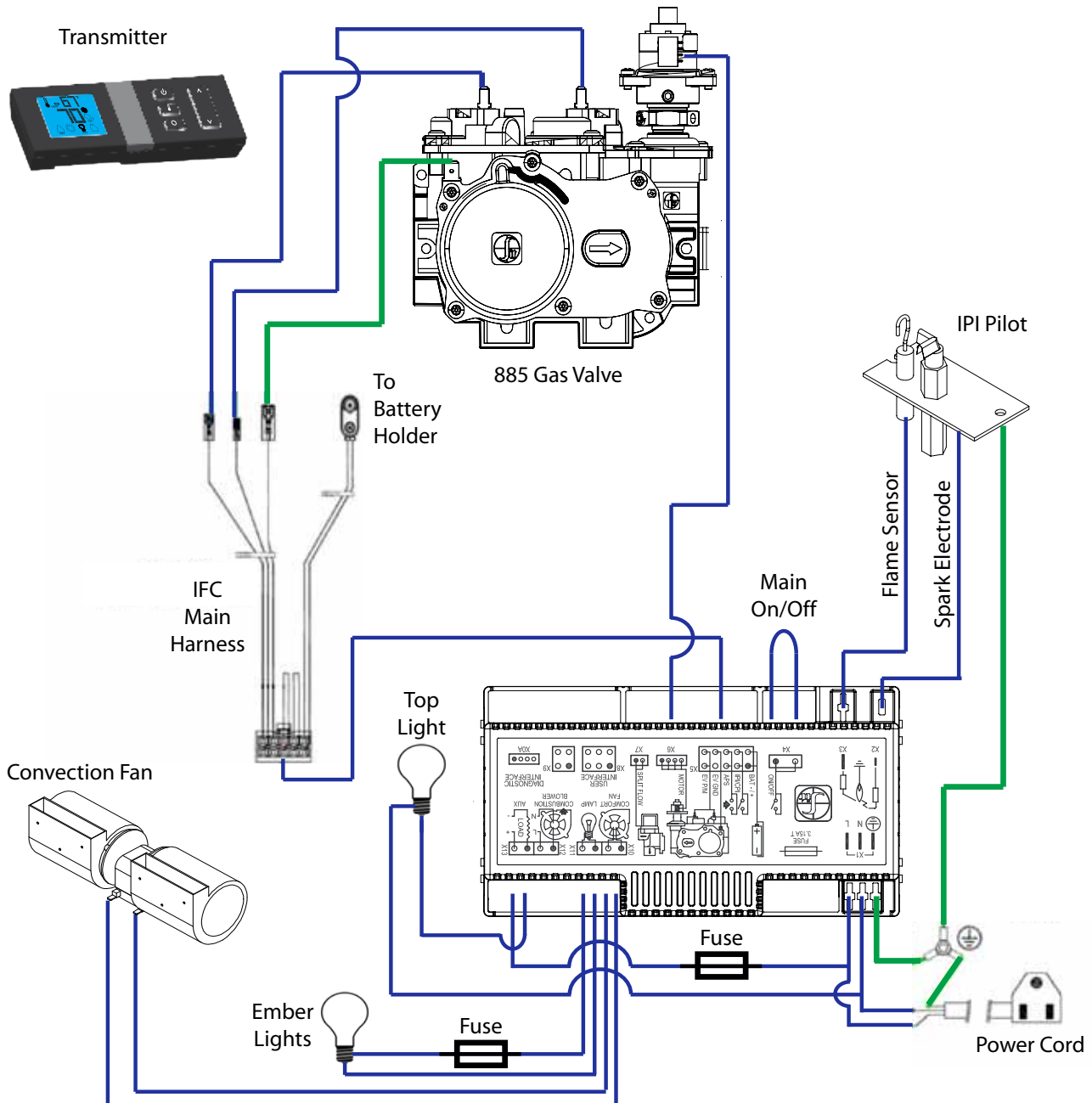
Figure 67: Proflame 2 Wiring Diagram
