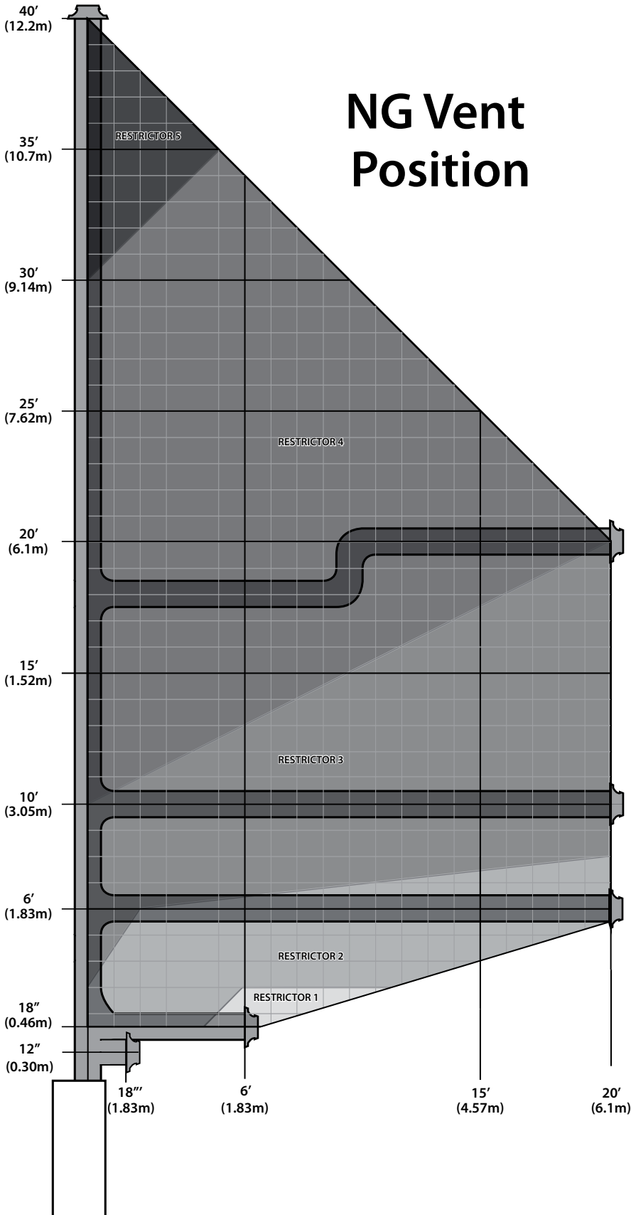
Figure 58. Natural Gas Vent Graph
