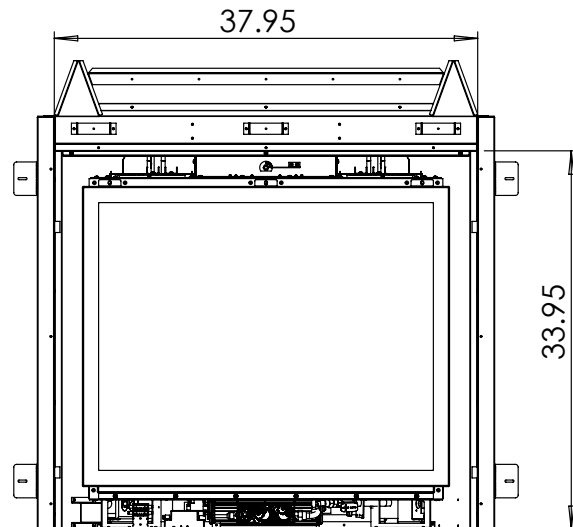
Figure 40: Inner Finishing Edge Dims
