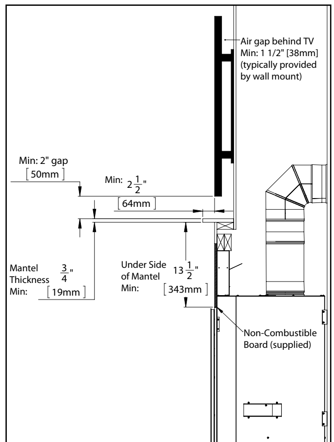
Figure 55. Recess Minimum TV Install
