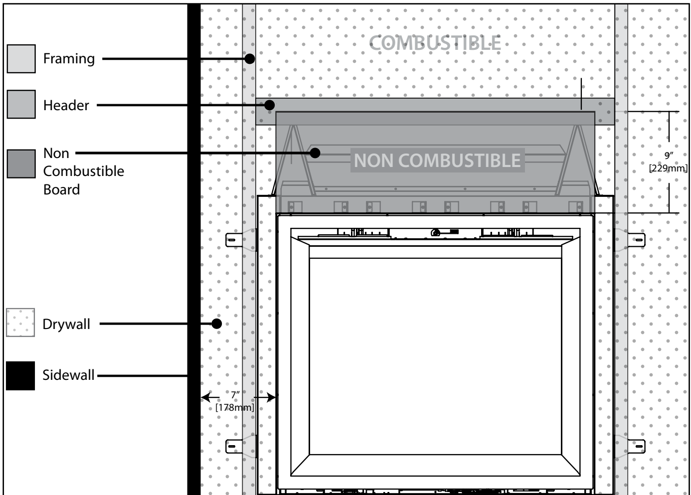
Figure 53. Typical Facing Layout
