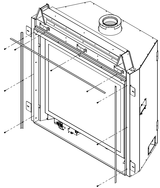
Figure 37: Outer finishing edge removal / replacement
