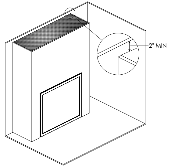
Figure 43B: Open Chase Iso View
