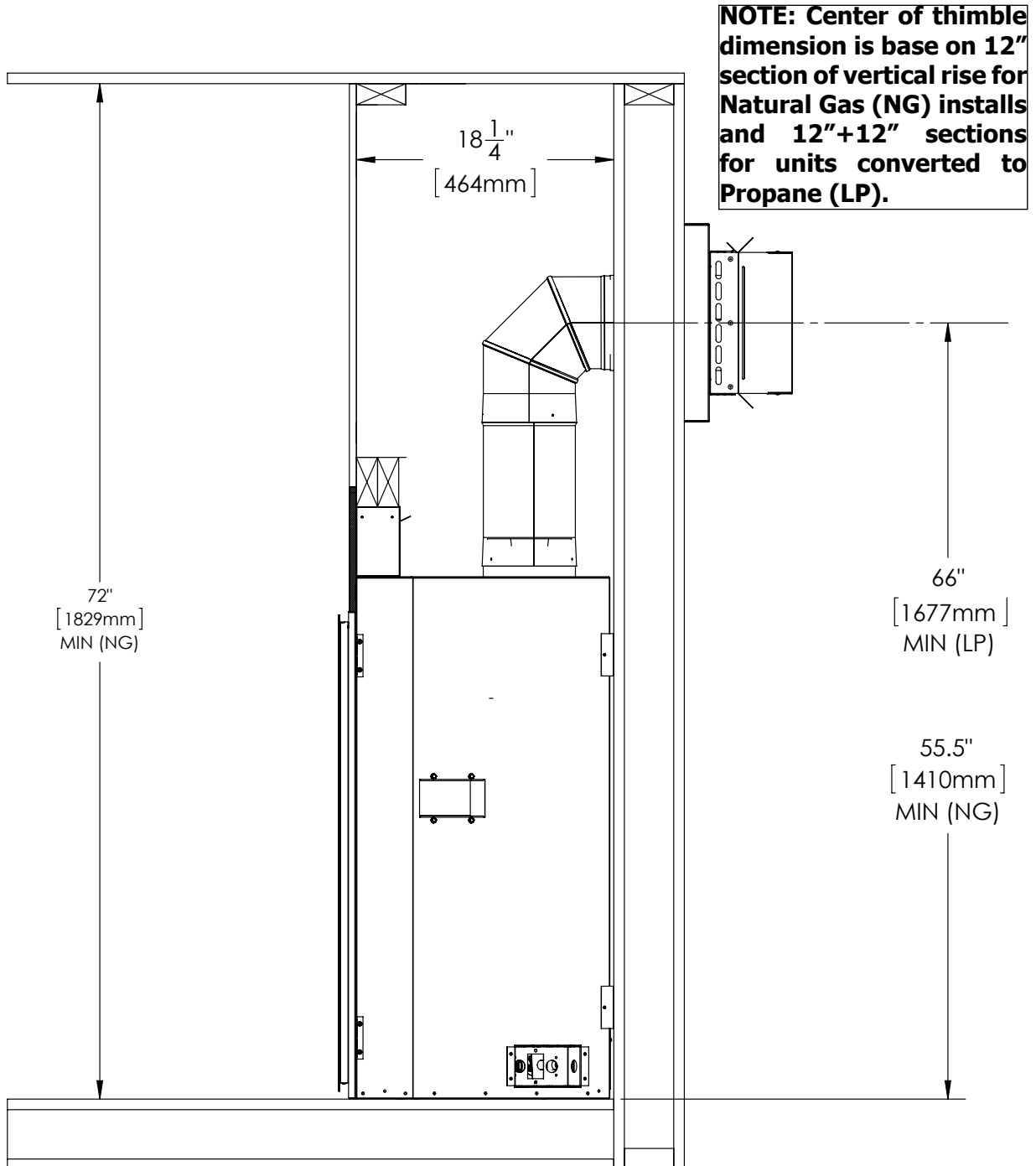
Figure 51: Minimum Vent (NG)
