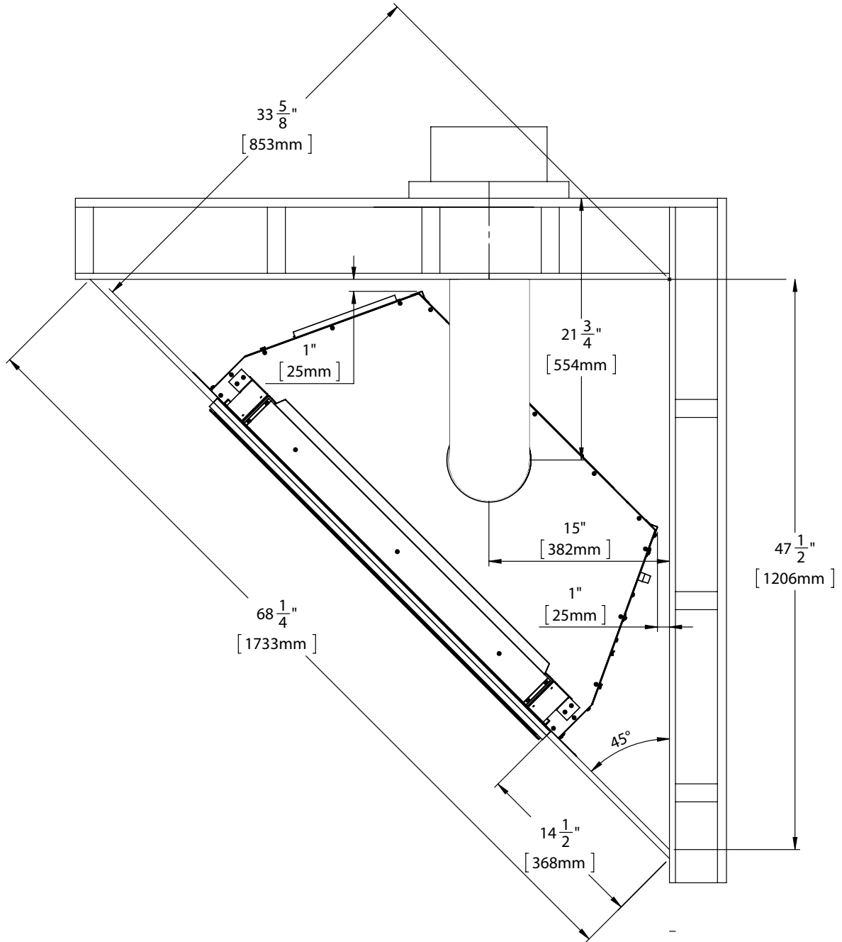
Figure 49. Corner Installation
