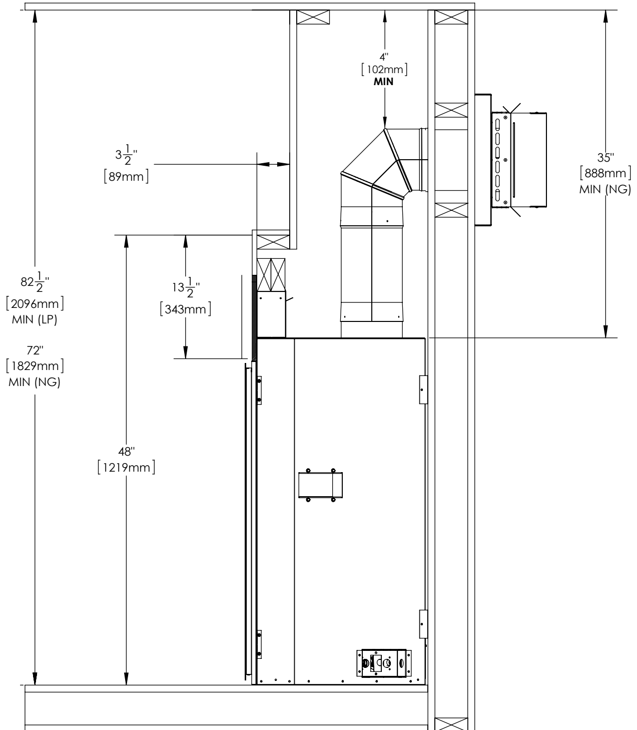
Figure 48: Recess Installation
