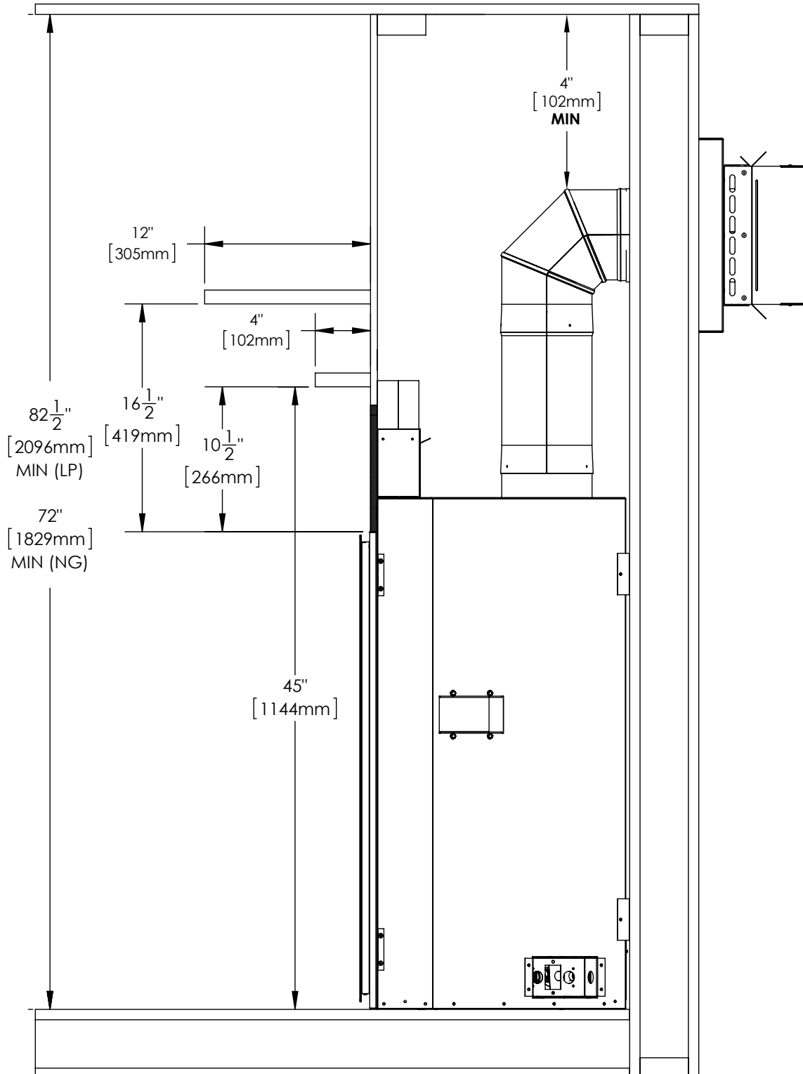
Figure 47: Flat Wall Installation
