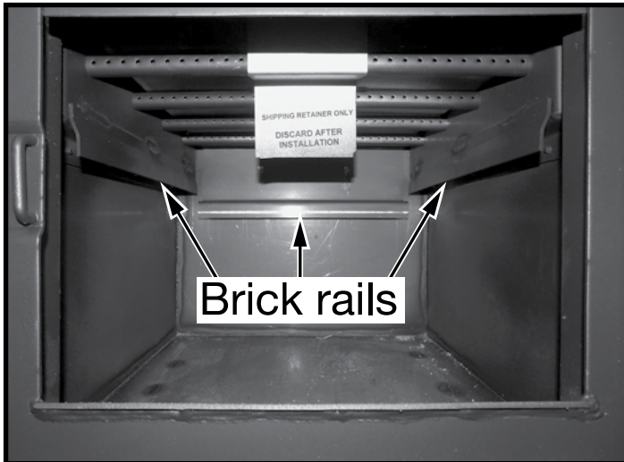
Figure 12: Firebox and brick rails.
