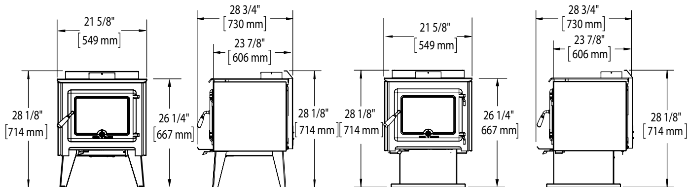
Figure 1: TN20B Dimensions.
