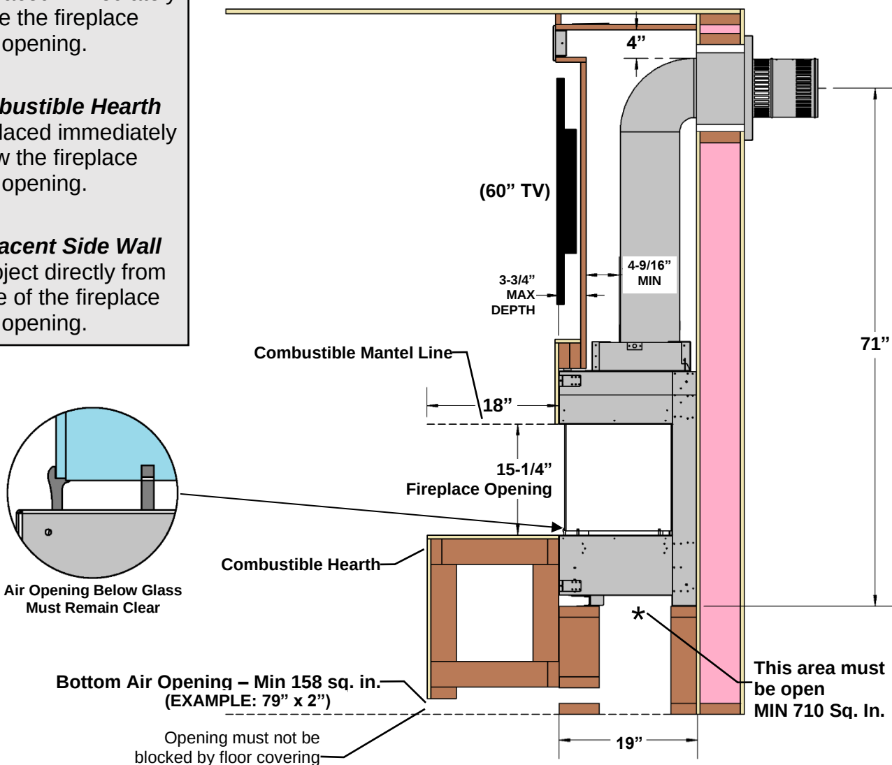
SIDE VIEW (MQVLBG72 Shown)
