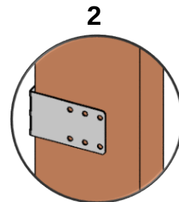
2 Rotate 180° for framing flush with fireplace face.
