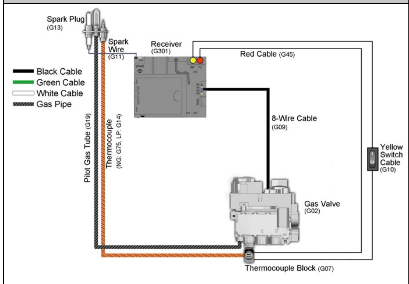
Wiring Diagram: Screen Fireplace (Batteries)
