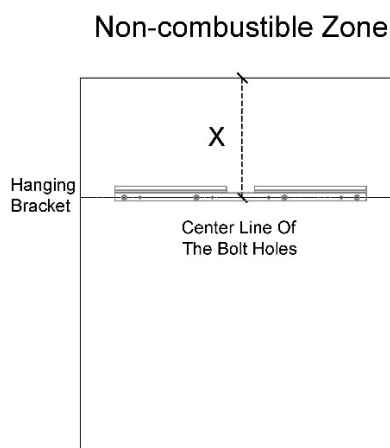
40TS Bracket
