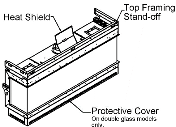
Zero-Clearance Stand-Offs (Isometric View)
