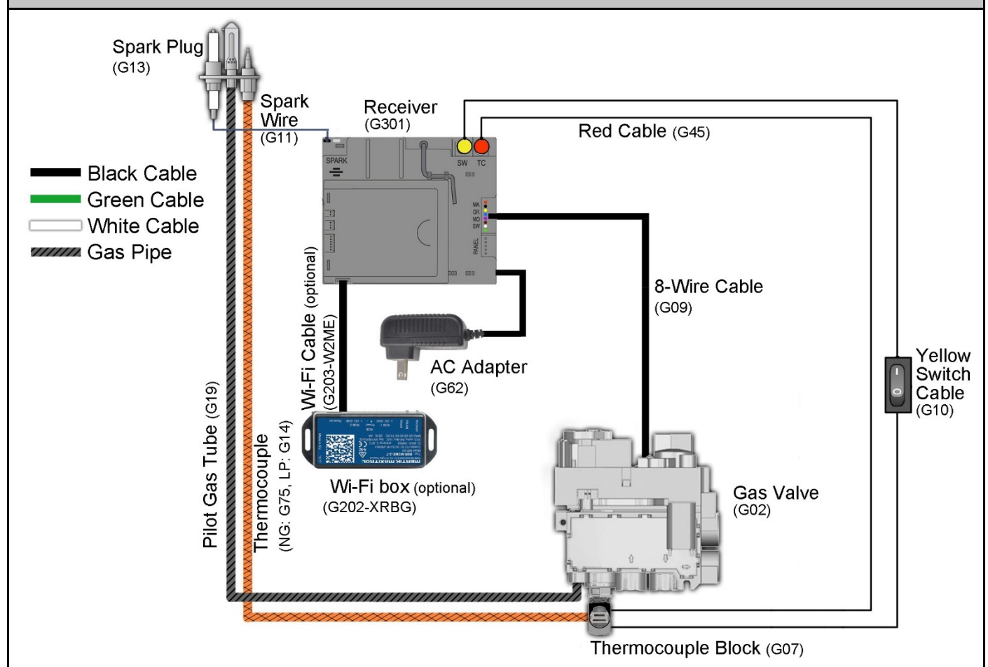
Wiring Diagram: Screen Fireplace
