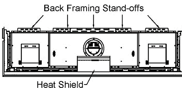
Zero-Clearance Stand-Offs (Top View)
