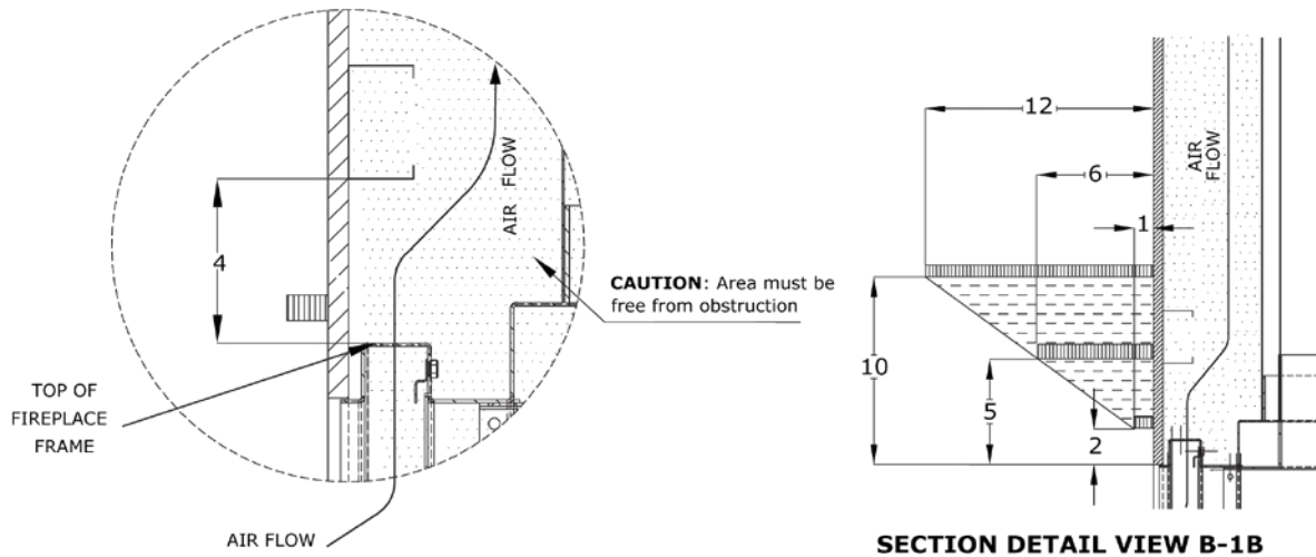
SECTION DETAIL VIEW B-1B
