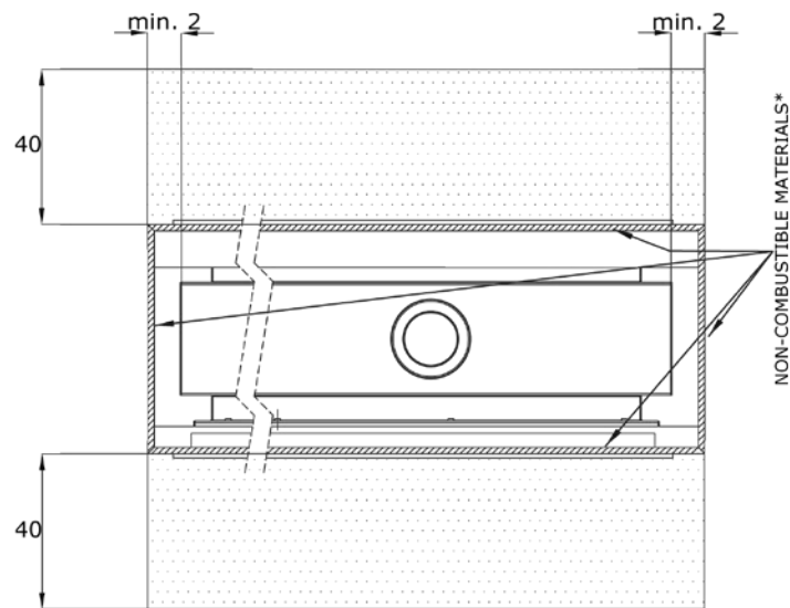
SECTION DETAIL VIEW B-1B
