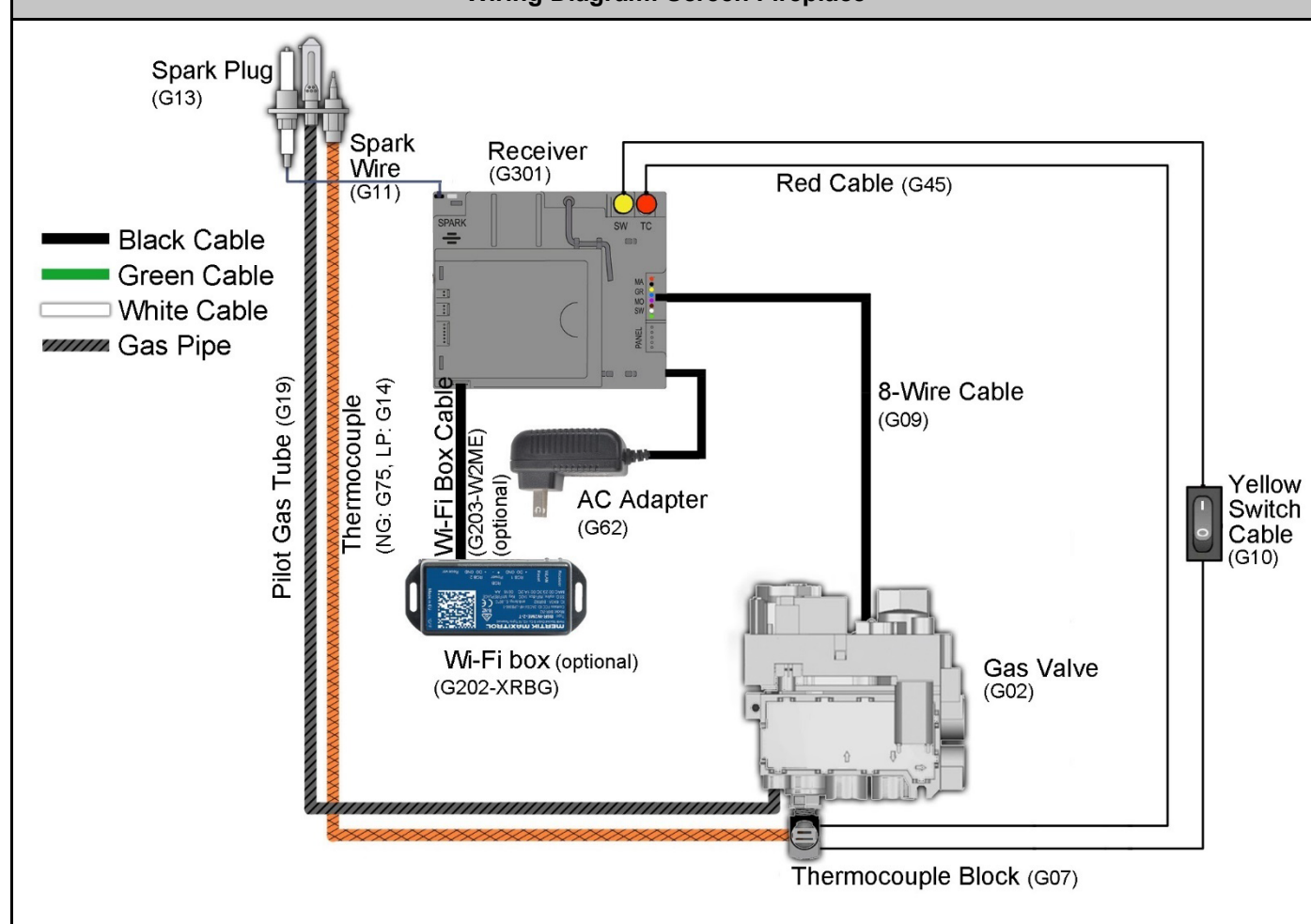
Wiring Diagram: Screen Fireplace
